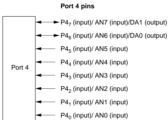
Figure 9-4 Port 4 Pin Functions
