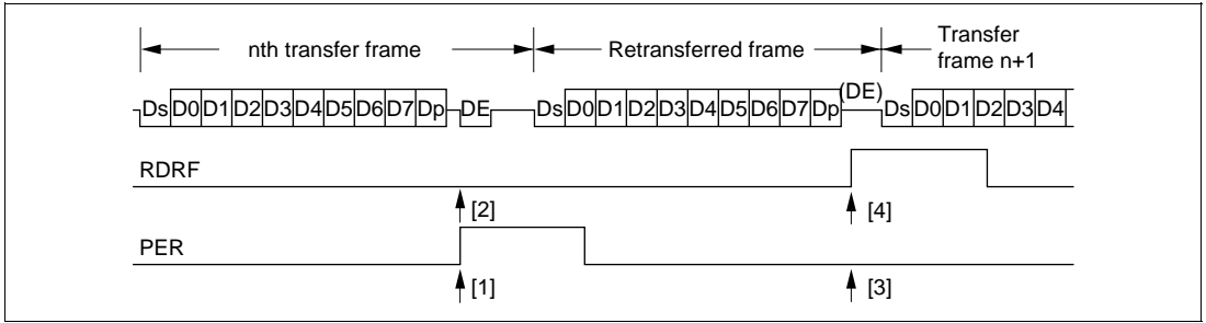
Figure 14-11 Retransfer Operation in SCI Receive Mode
