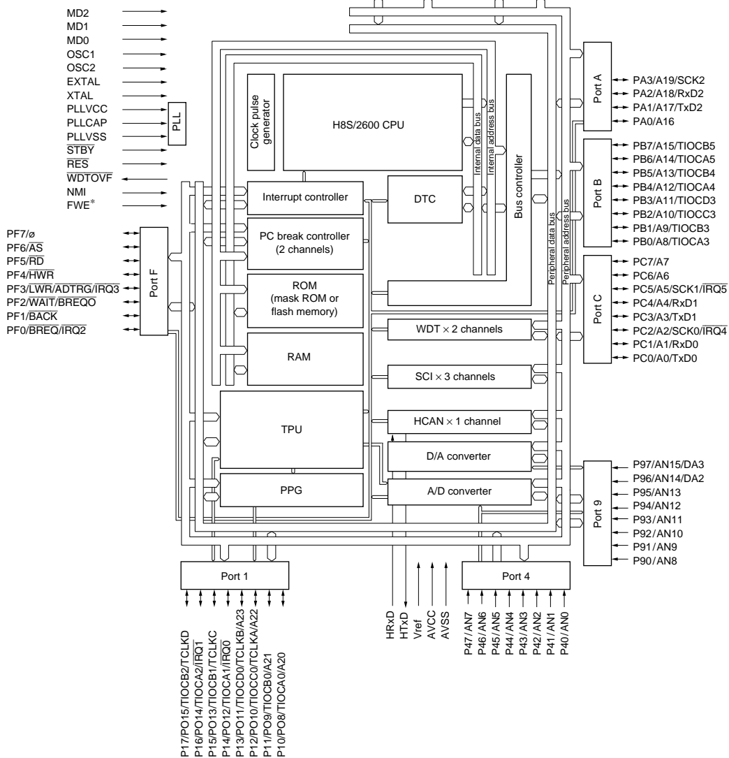
Figure 1-2 Internal Block Diagram (H8S/2626 Series)
