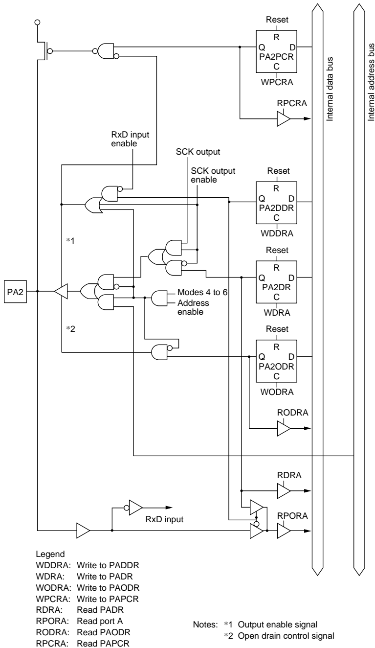
Figure C-4 (c) Port A Block Diagram (Pin PA2)
