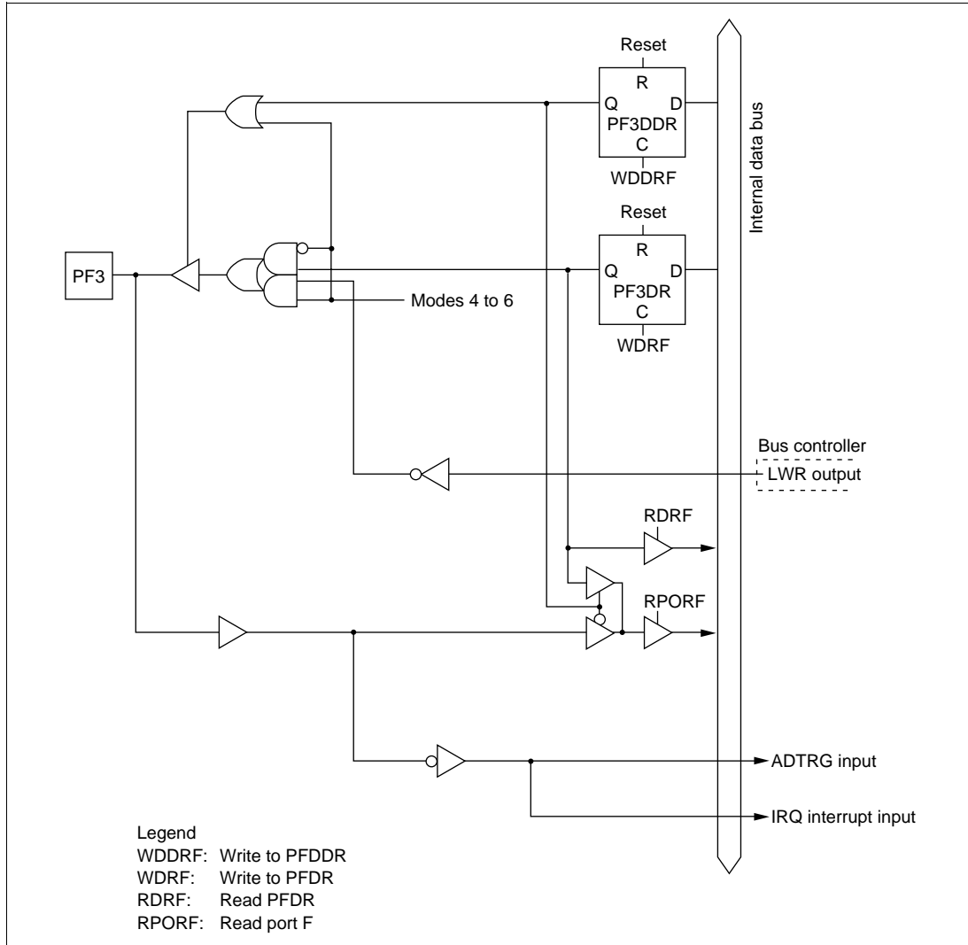
Figure C-9 (e) Port F Block Diagram (Pin PF3)
