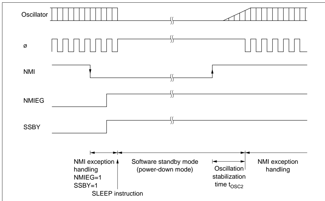
Figure 21A-3 Software Standby Mode Application Example
