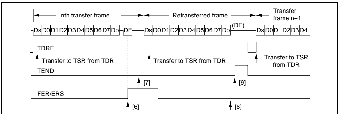
Figure 14-12 Retransfer Operation in SCI Transmit Mode
