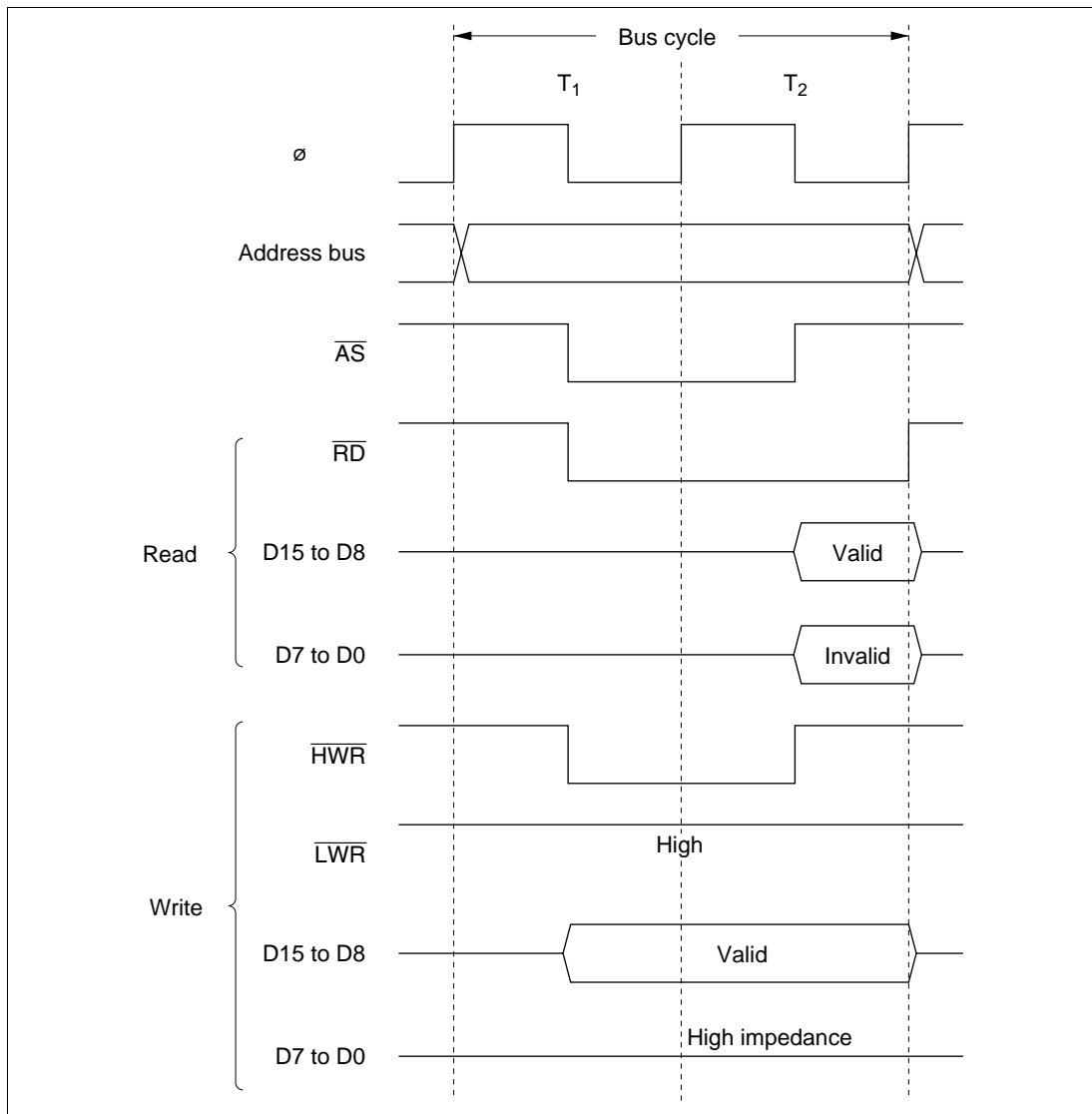
Figure 7-5 Bus Timing for 8-Bit 2-State Access Space
