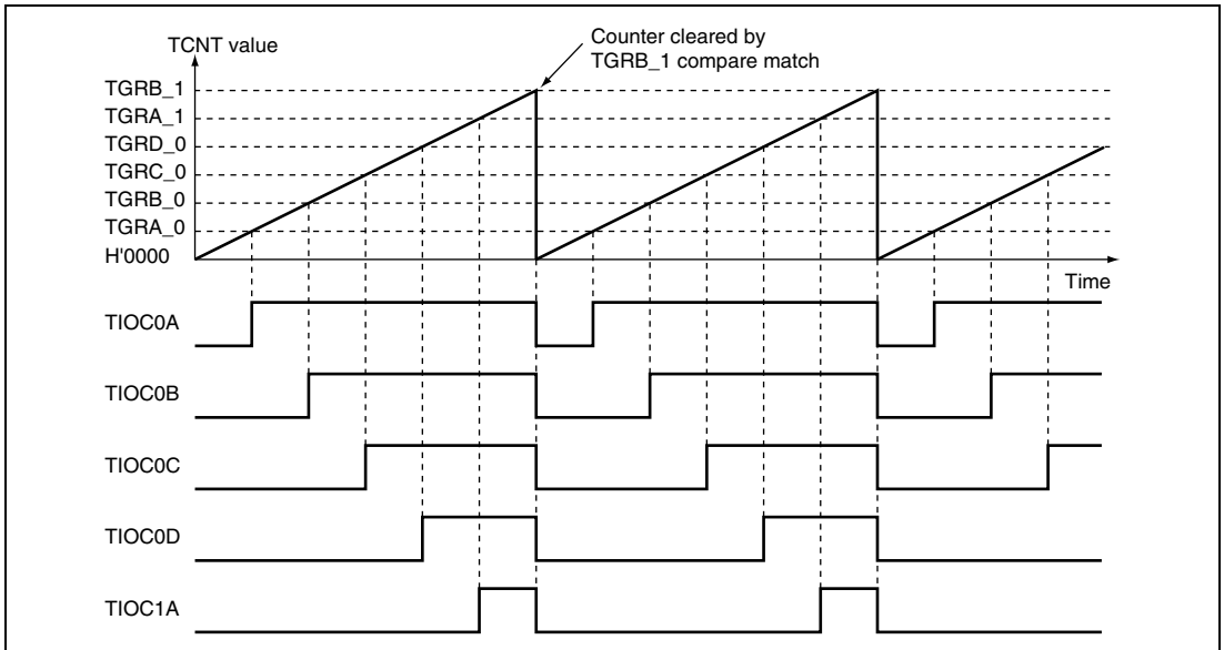
Figure 18.22 Example of PWM Mode Operation (2)
