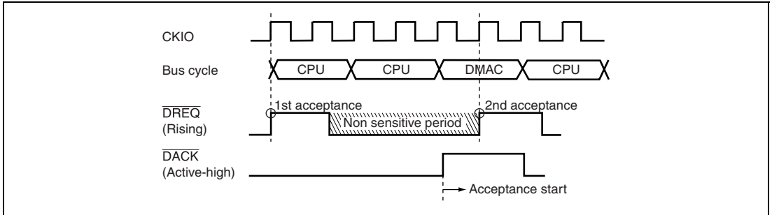
Figure 13.13 Example of \overline{\text{DREQ}} Input Detection in Cycle Steal Mode Edge Detection
