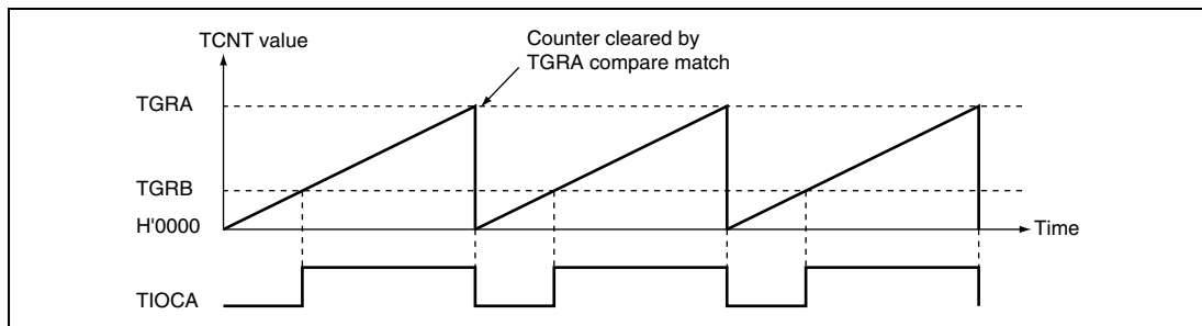
Figure 18.21 Example of PWM Mode Operation (1)
