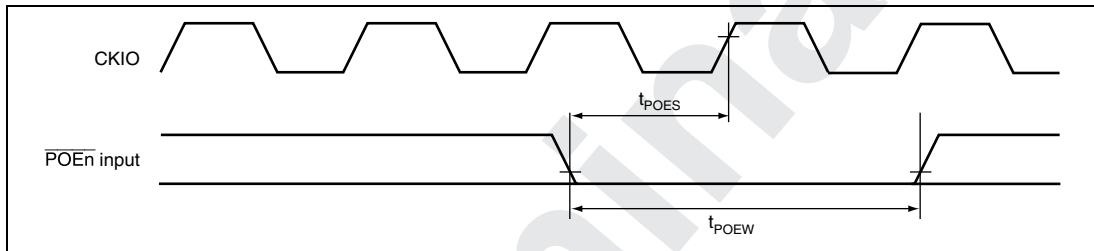
Figure 25.49 POE Input/Output Timing
