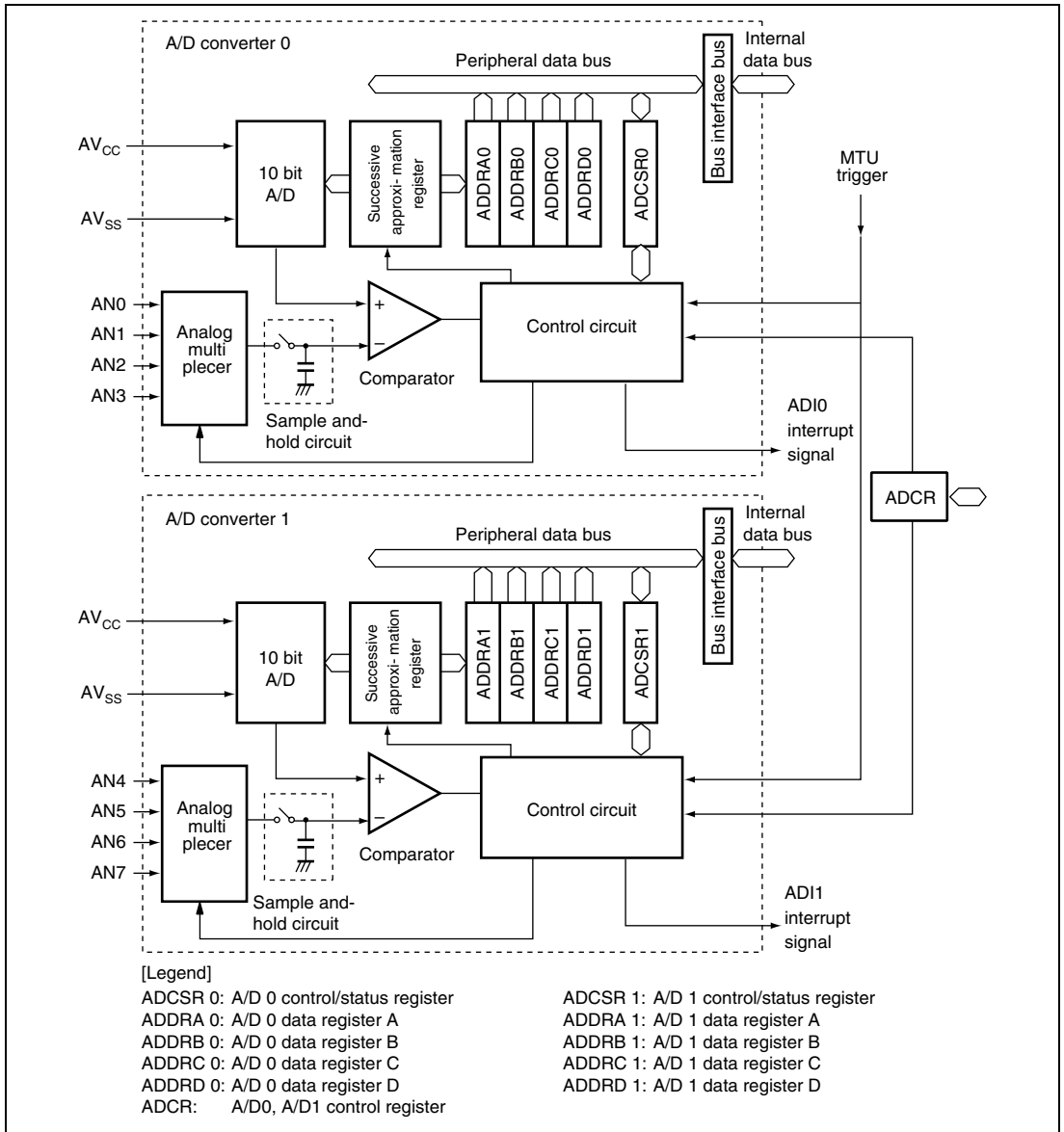
Figure 21.1 Block Diagram of A/D Converter
