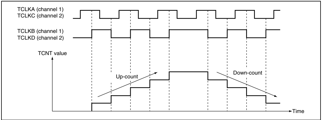
Figure 18.28 Example of Phase Counting Mode 4 Operation
