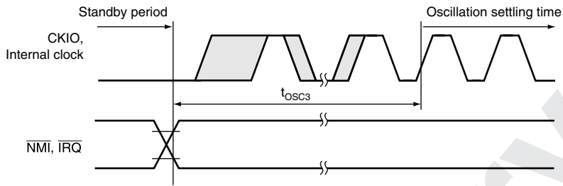
Figure 25.8 Oscillation Settling Timing (Standby Mode Canceled by \overline{\text{NMI}} or \overline{\text{IRQ}} )
