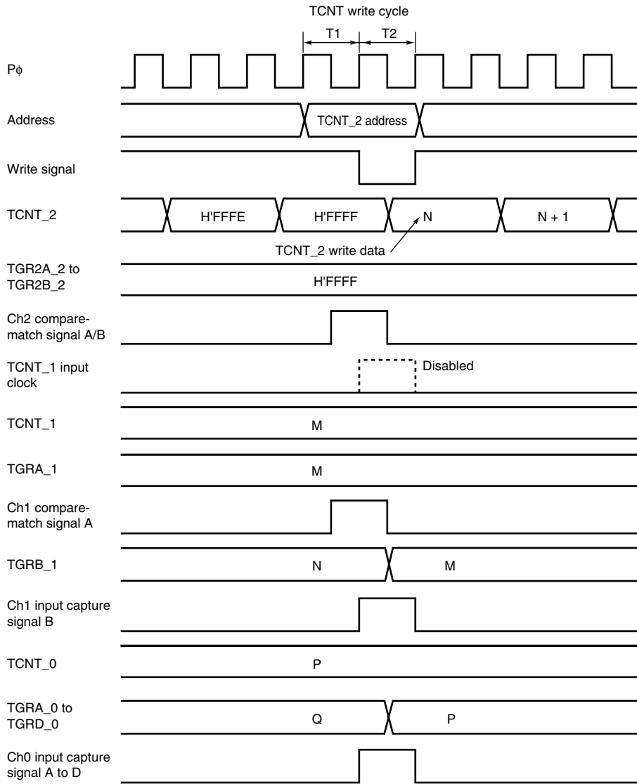
Figure 18.79 TCNT_2 Write and Overflow/Underflow Conflict with Cascade Connection
