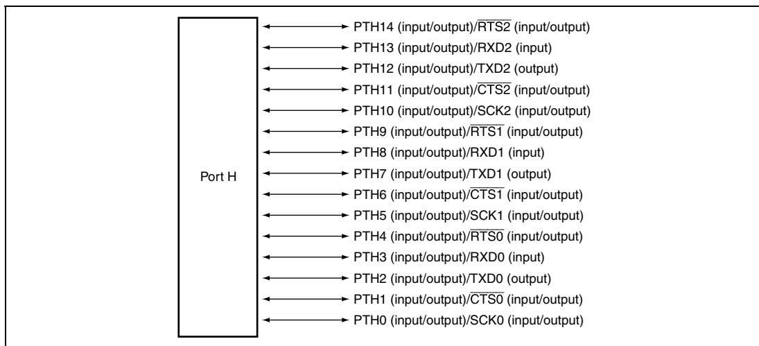
Figure 23.9 Port H
