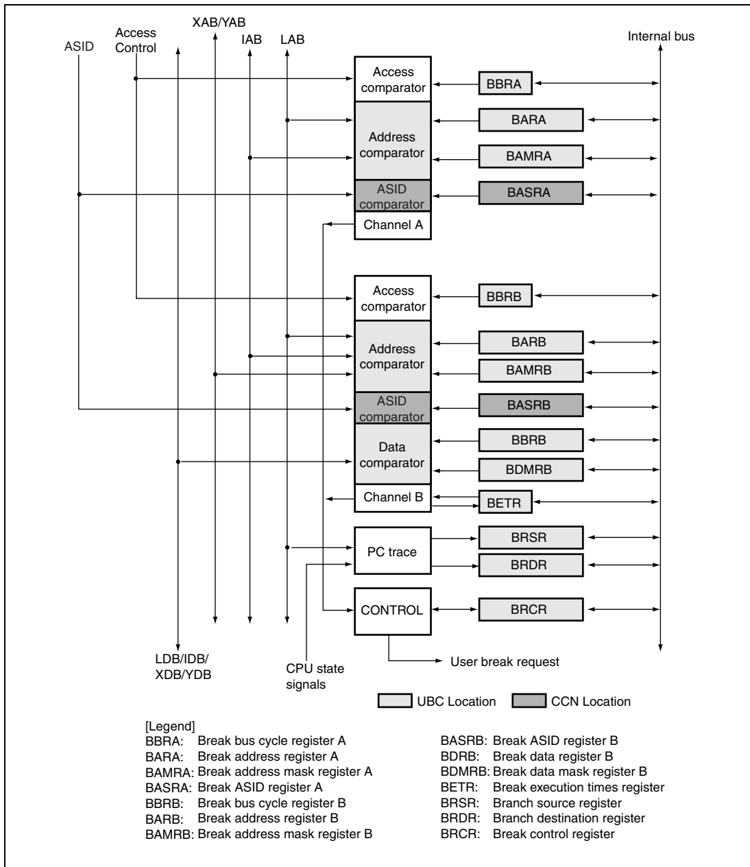
Figure 11.1 Block Diagram of User Break Controller
