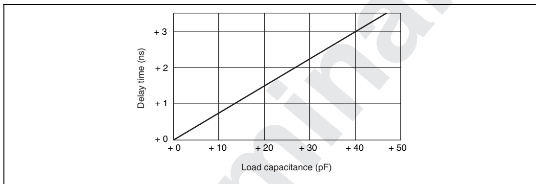
Figure 25.58 Load Capacitance vs. Delay Time
