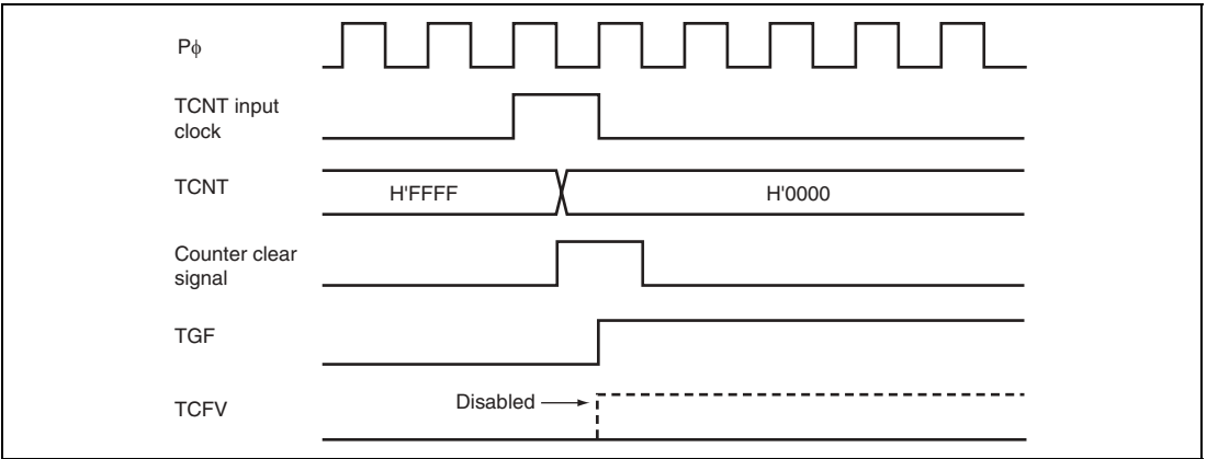
Figure 18.83 Conflict between Overflow and Counter Clearing
