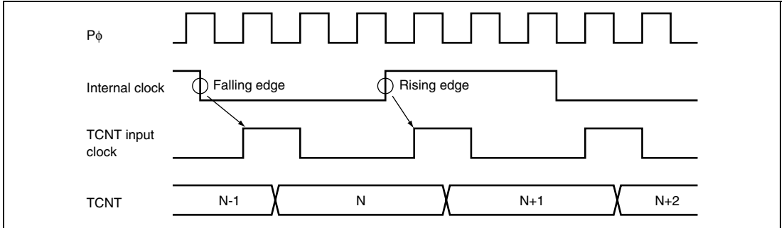
Figure 18.54 Count Timing in Internal Clock Operation
