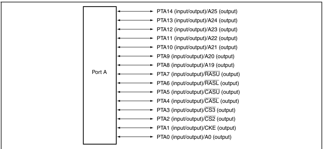
Figure 23.1 Port A
