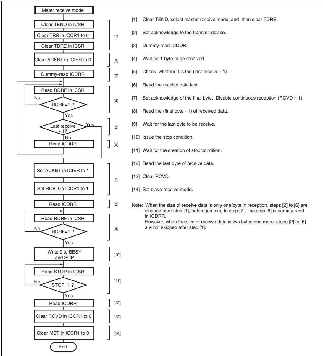
Figure 16.19 Sample Flowchart for Master Receive Mode
