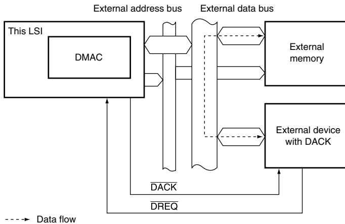
Figure 13.7 Data Flow in Single Address Mode
