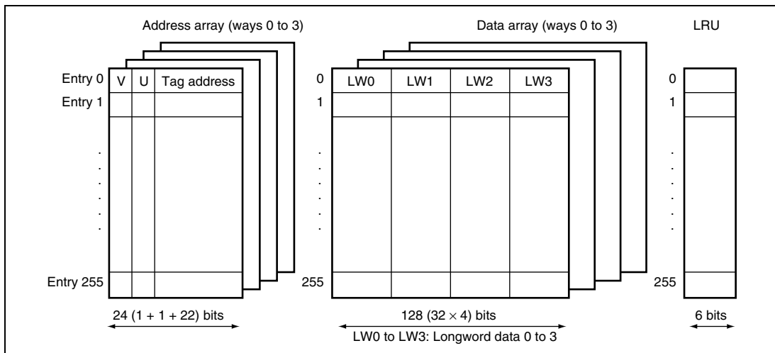
Figure 7.1 Cache Structure
