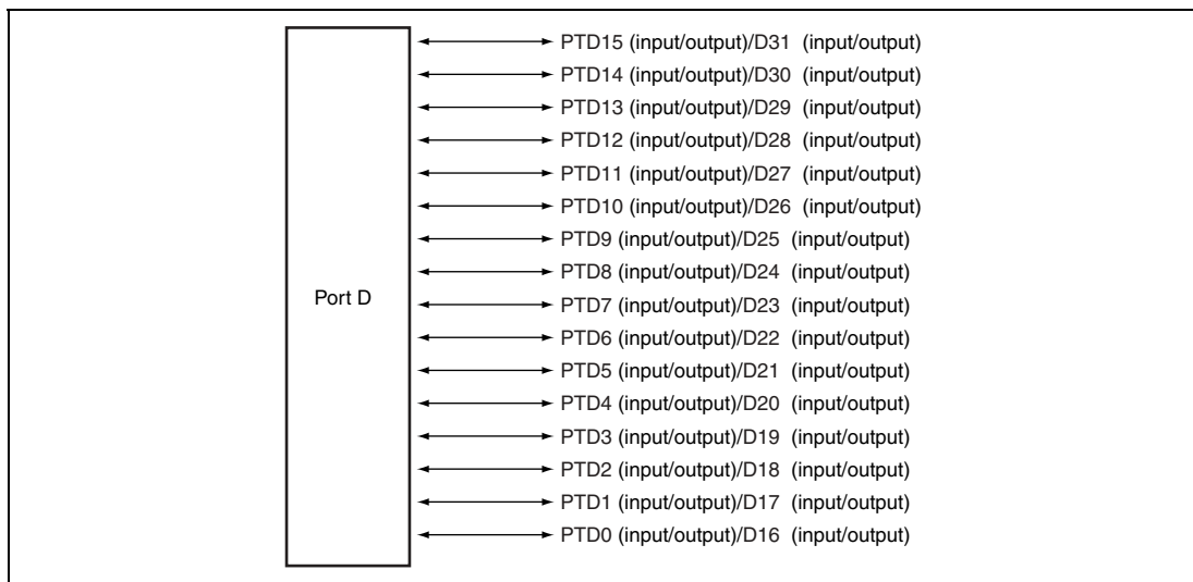
Figure 23.4 Port D
