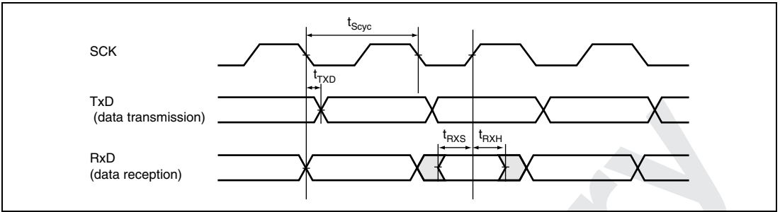
Figure 25.43 SCIF Input/Output Timing in Synchronous Mode
