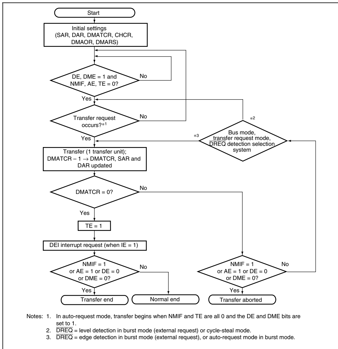
Figure 13.2 DMA Transfer Flowchart
