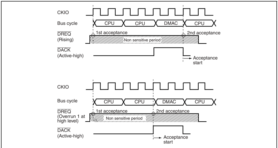
Figure 13.14 Example of \overline{\text{DREQ}} Input Detection in Cycle Steal Mode Level Detection
