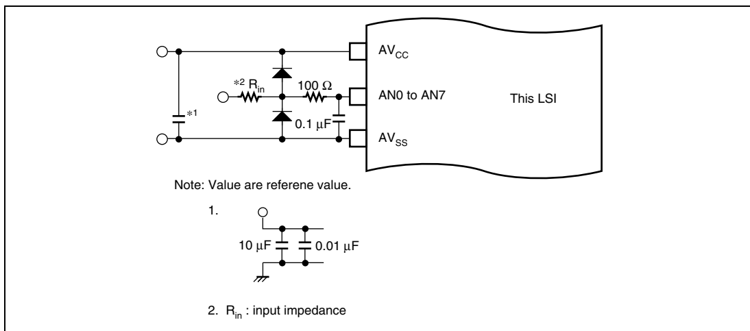
Figure 21.7 Example of Analog Input Protection Circuit
