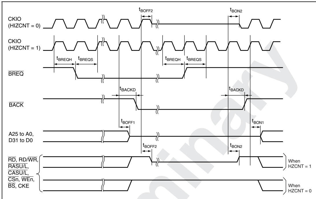
Figure 25.11 Bus Release Timing
