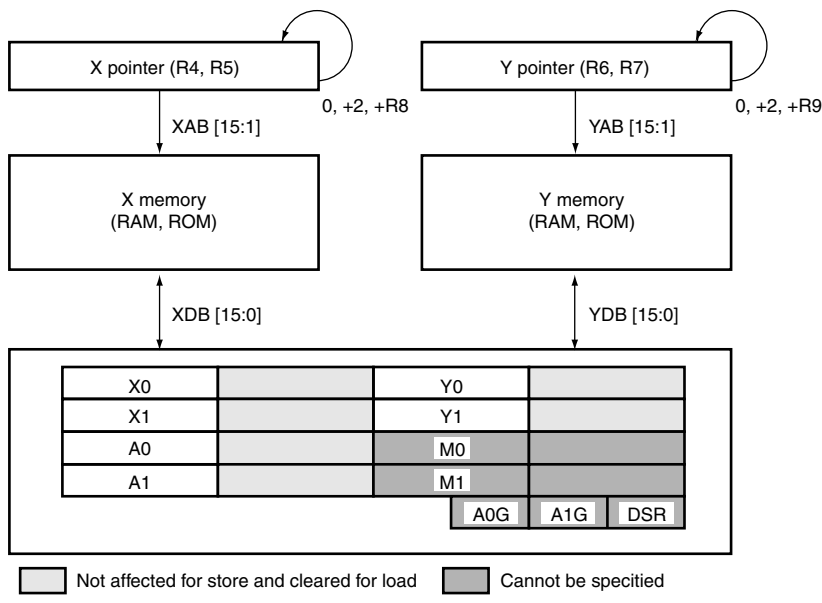
Figure 3.14 Data Transfer Operation Flow
