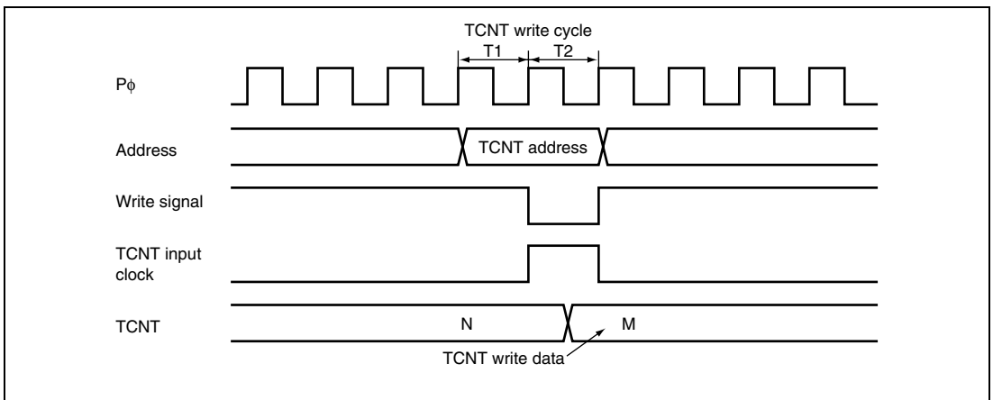
Figure 18.72 Conflict between TCNT Write and Increment Operations
