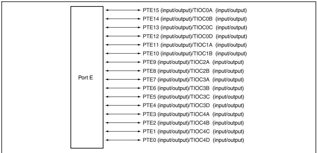
Figure 23.5 Port E
