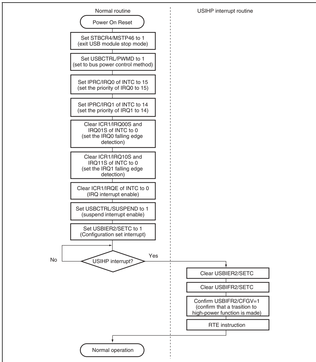
Figure 20.21 Sample Flowchart for Initialization of the USB Bus Power Control Method
