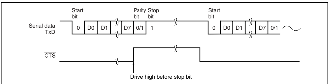
Figure 19.6 Example of Operation Using Modem Control ( \overline{\text{CTS}} )
