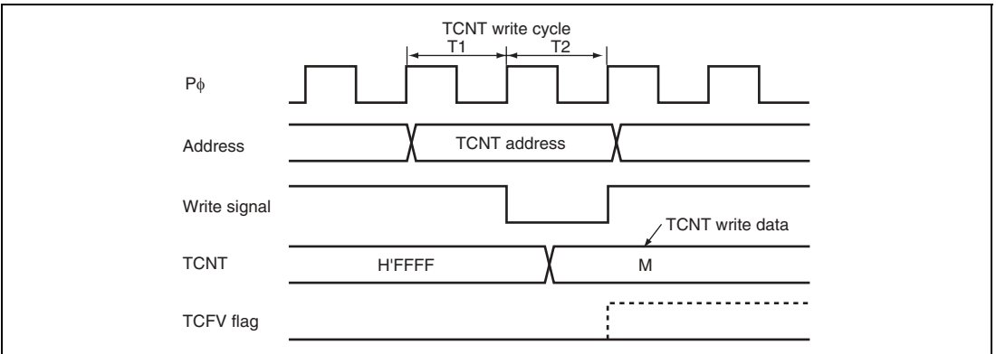
Figure 18.84 Conflict between TCNT Write and Overflow
