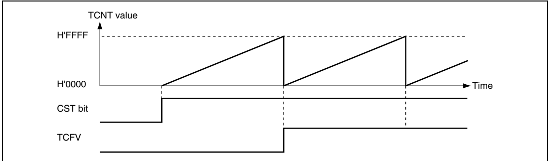
Figure 18.4 Free-Running Counter Operation
