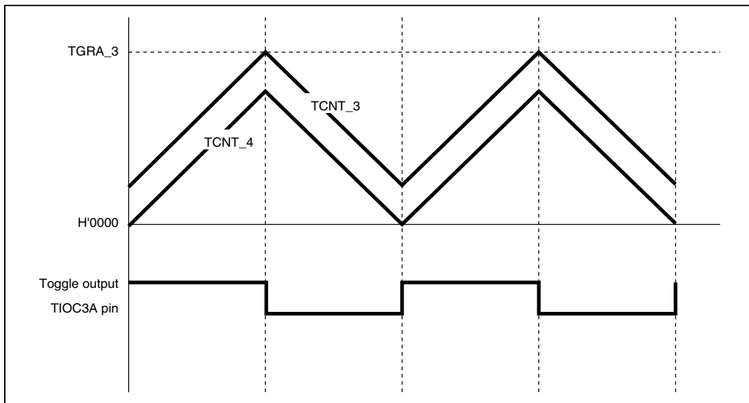
Figure 18.48 Example of Toggle Output Waveform Synchronized with PWM Output
