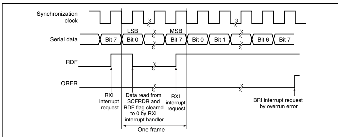
Figure 19.17 Example of SCIF Receive Operation
