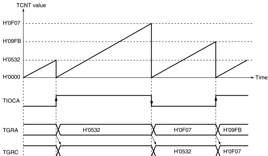
Figure 18.17 Example of Buffer Operation (2)
