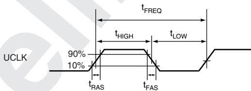
Figure 25.56 USB Clock Timing
