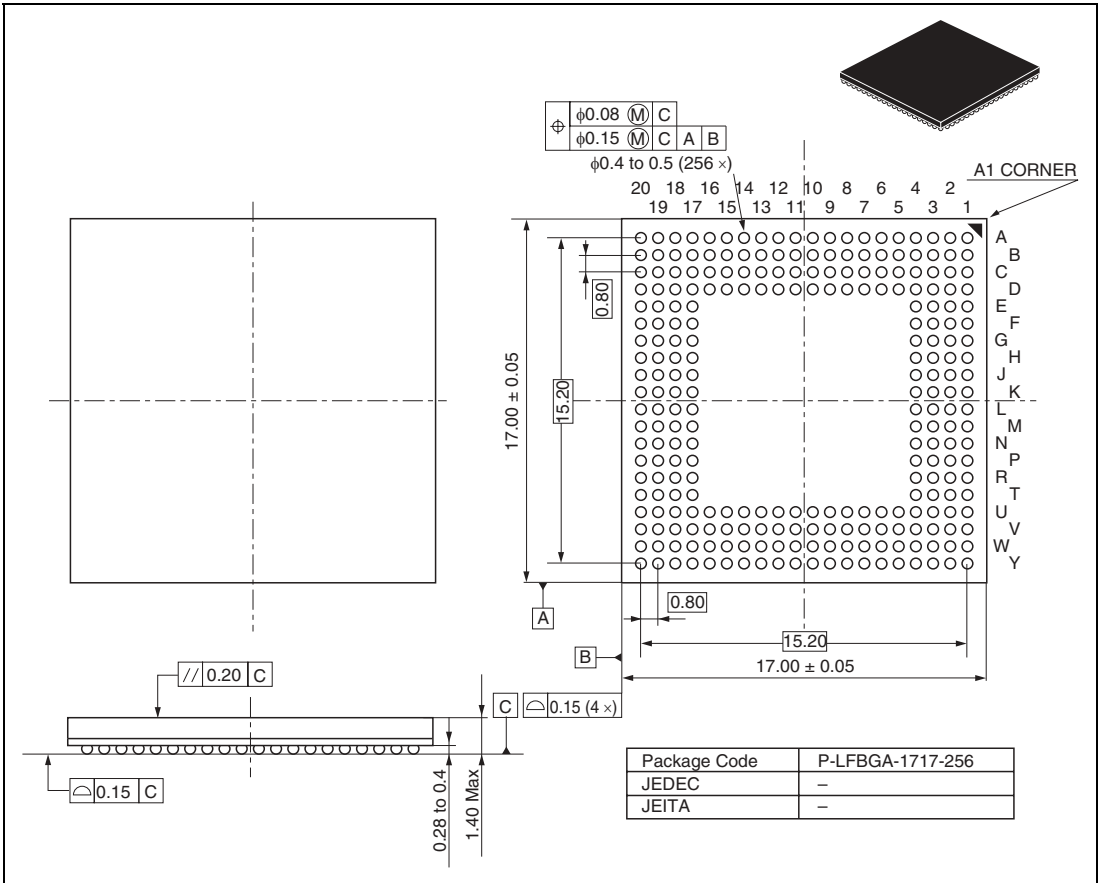
Figure C.1 Package Dimensions
