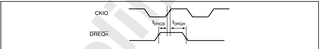
Figure 25.45 \overline{\text{DREQ}} Input Timing
