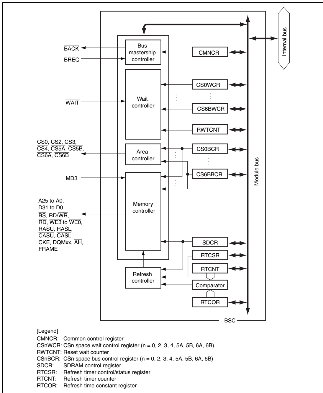
Figure 12.1 BSC Functional Block Diagram
