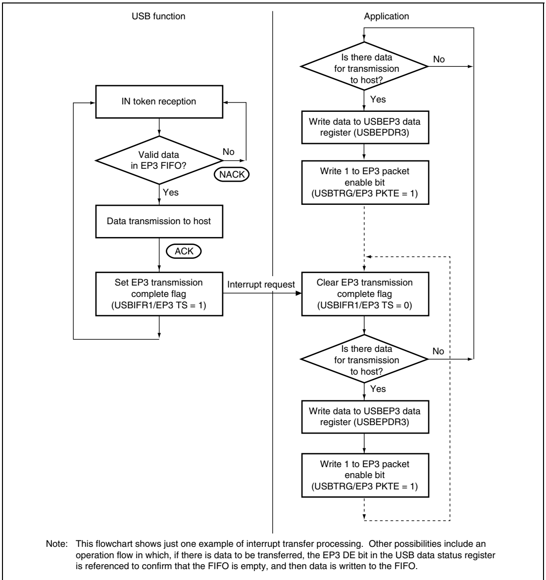
Figure 20.12 EP3 Interrupt-IN Transfer Operation
