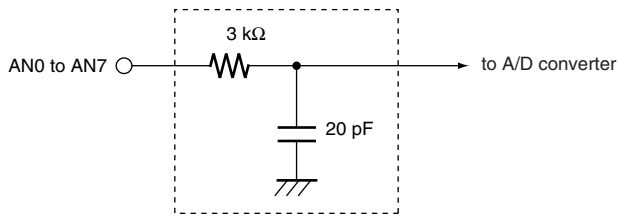
Figure 21.8 Analog Input Pin Equivalent Circuit
