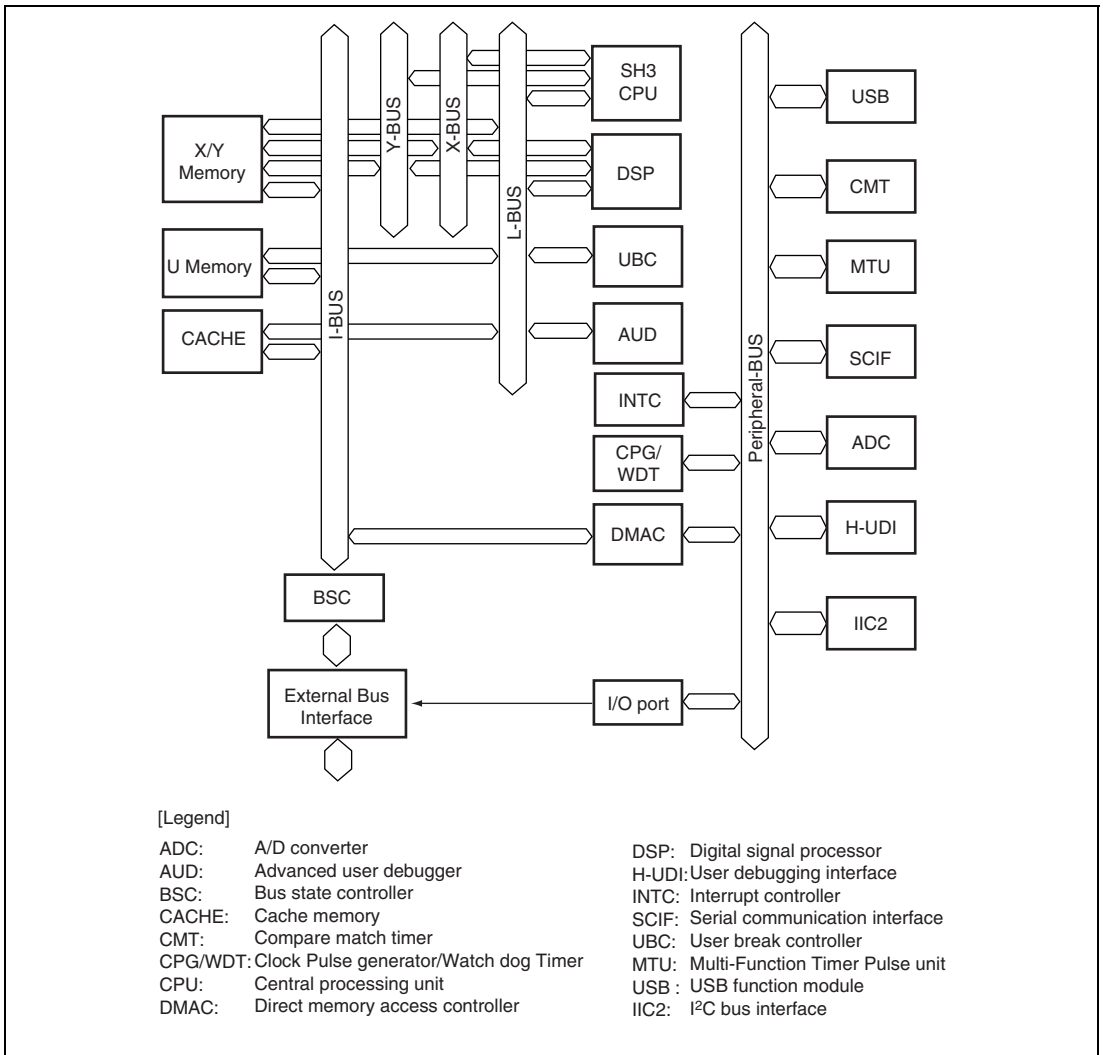
Figure 1.1 Block Diagram
