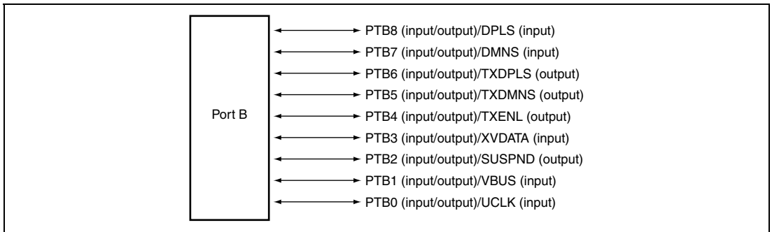
Figure 23.2 Port B
