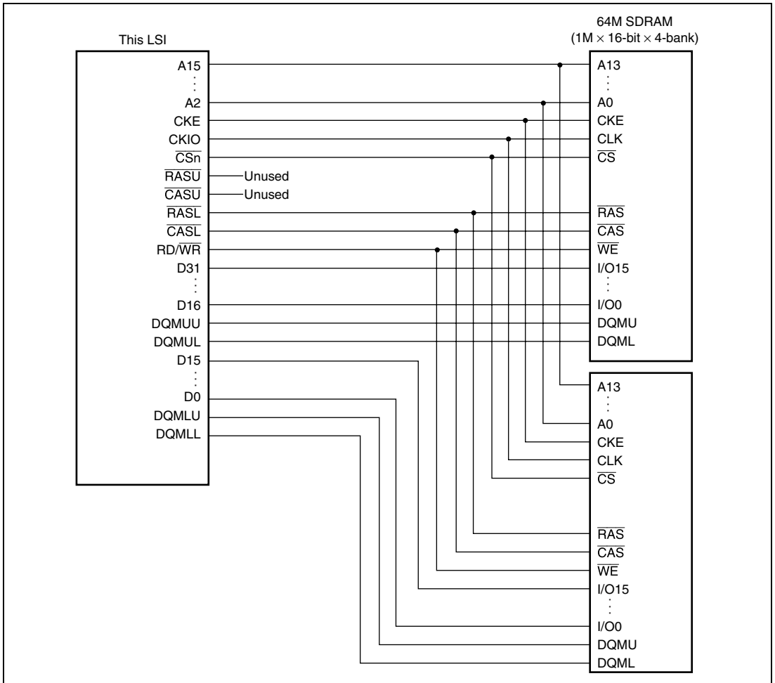
Figure 12.15 Example of 32-Bit Data Width SDRAM Connection (RASU and CASU are Not Used)
