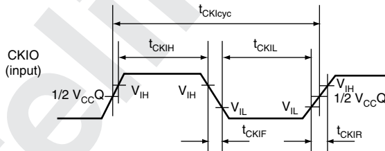
Figure 25.3 CKIO Clock Input Timing
