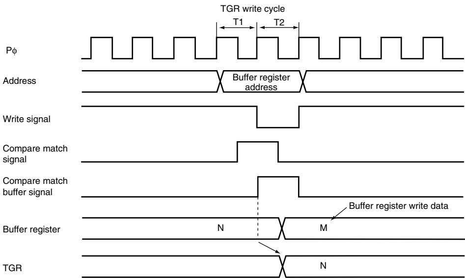
Figure 18.75 Conflict between Buffer Register Write and Compare Match (Channels 3 and 4)
