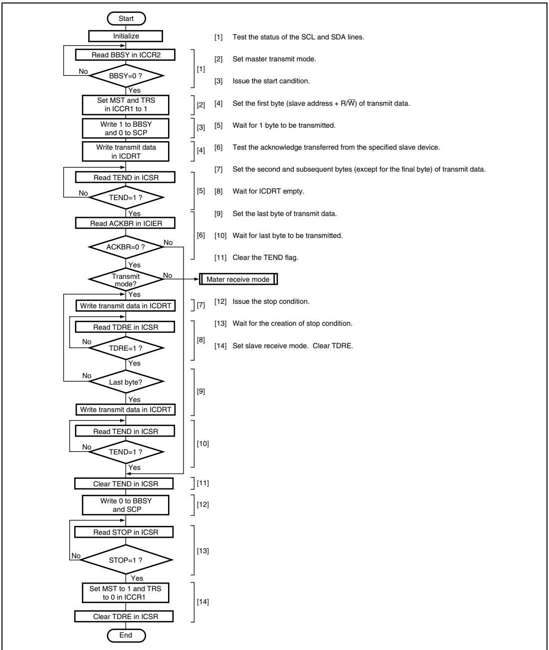
Figure 16.18 Sample Flowchart for Master Transmit Mode
