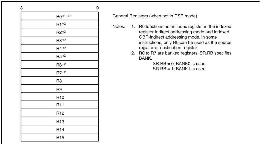
Figure 2.3 General Registers (Not in DSP Mode)
