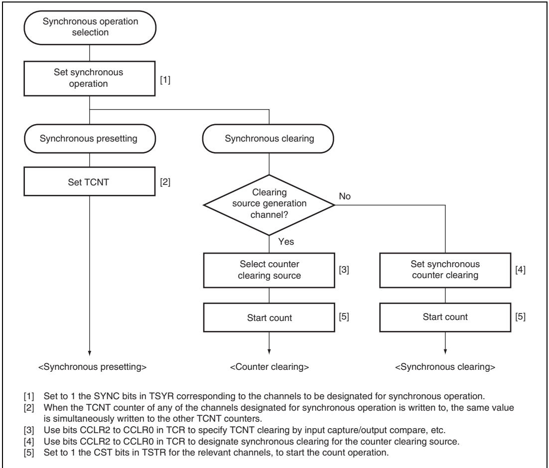
Figure 18.11 Example of Synchronous Operation Setting Procedure
