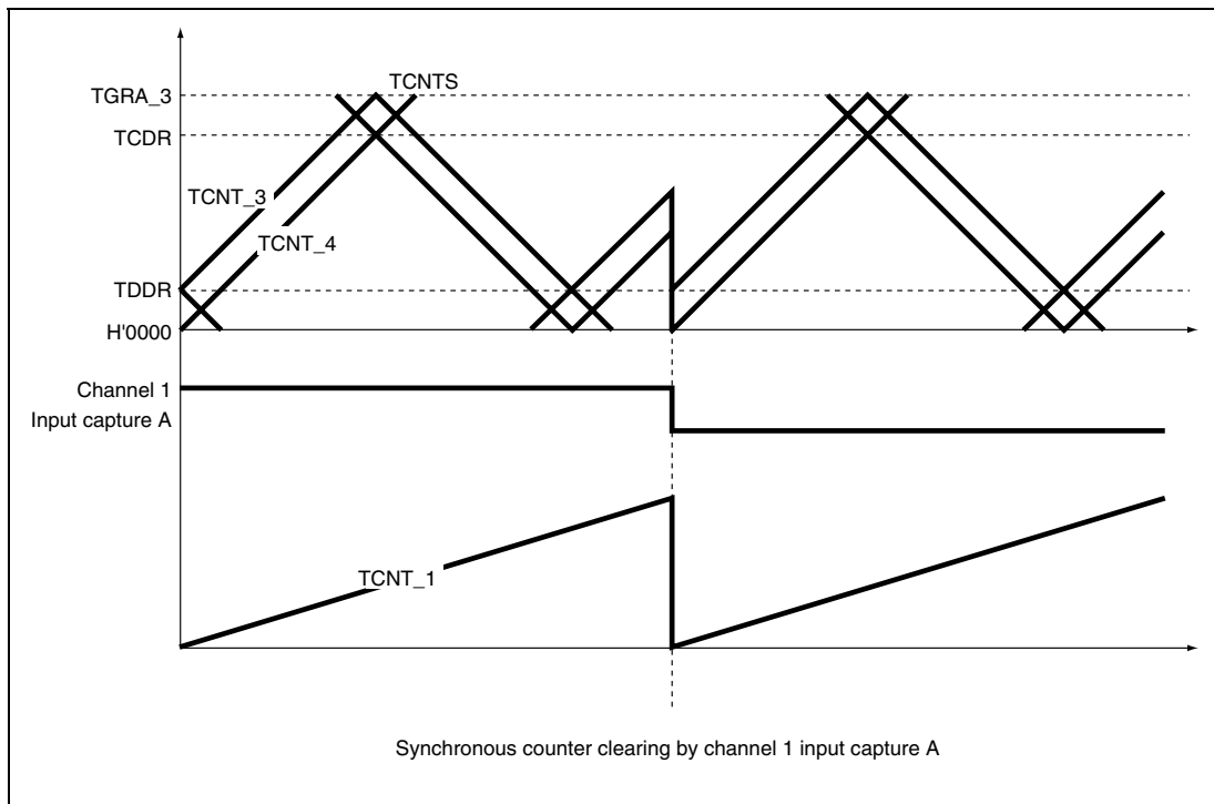
Figure 18.49 Counter Clearing Synchronized with Another Channel
