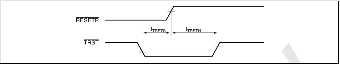
Figure 25.52 \overline{\text{TRST}} Input Timing (Reset-Hold State)
