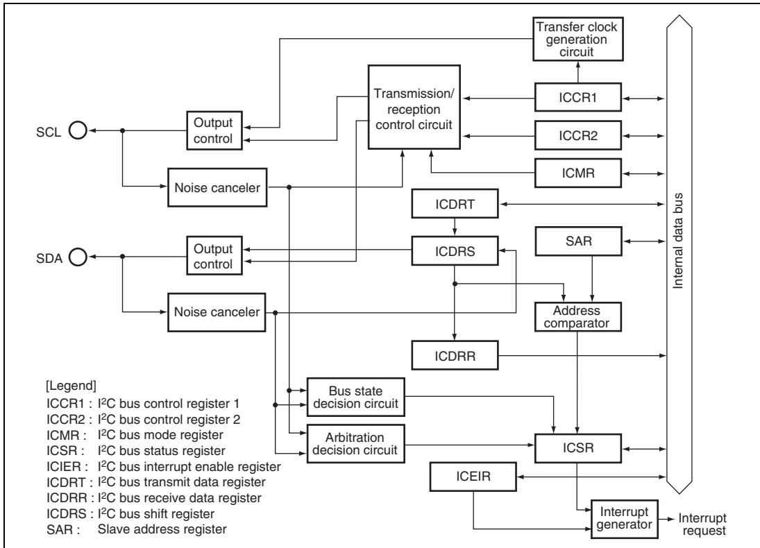
Figure 16.1 Block Diagram of I 2 C Bus Interface 2
