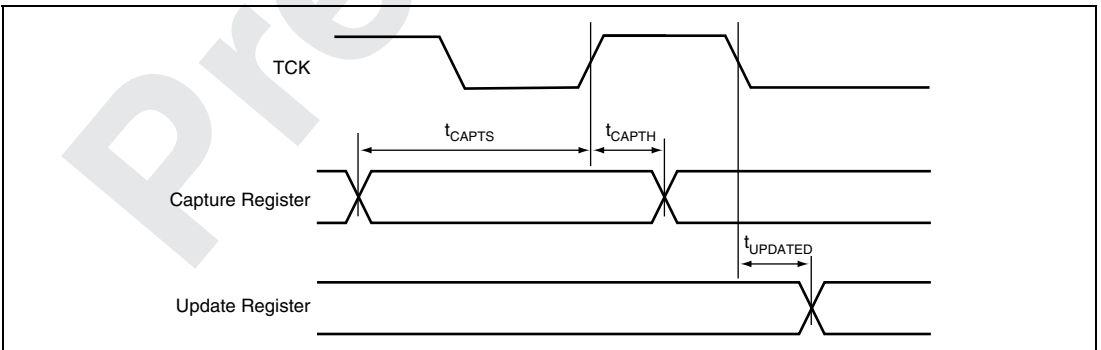
Figure 25.54 Boundary-Scan Input/Output Timing
