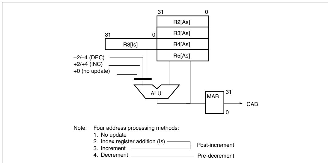
Figure 2.13 Single Data Transfer Addressing
