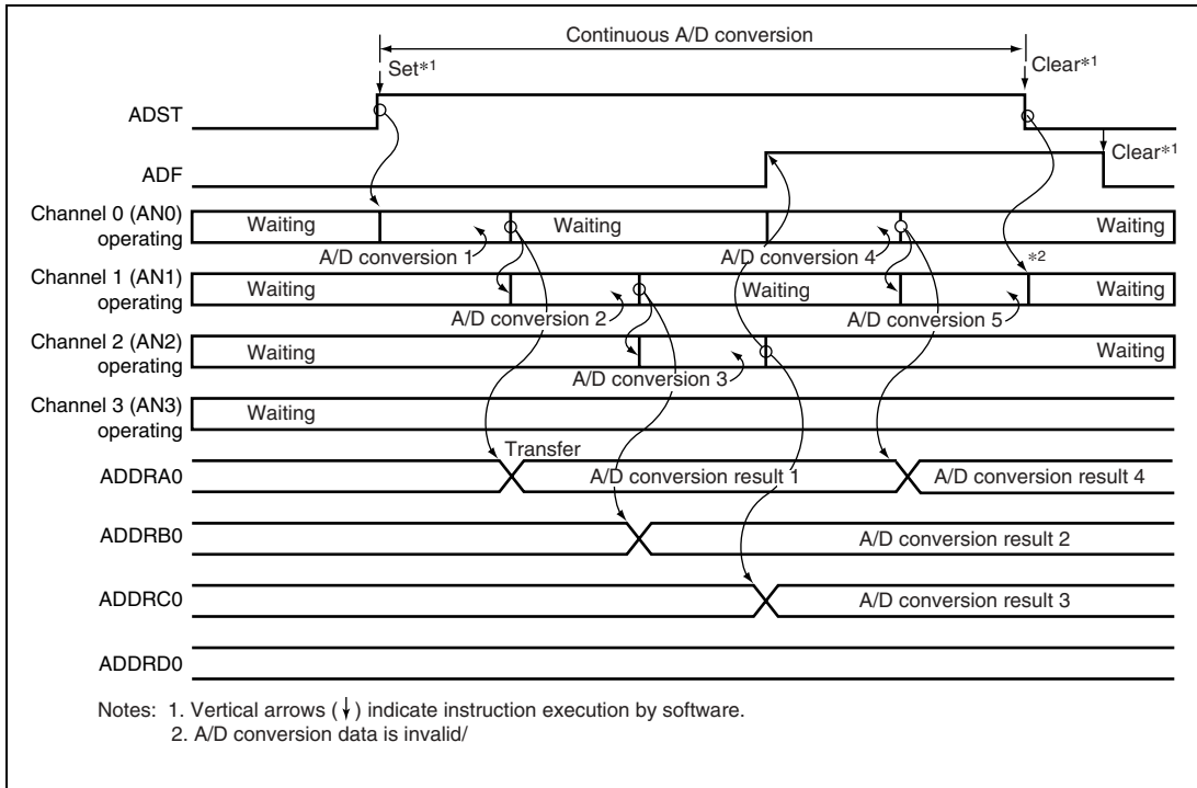
Figure 21.4 Example of A/D Converter Operation (Scan Mode, Channels AN0 to AN2 Selected)
