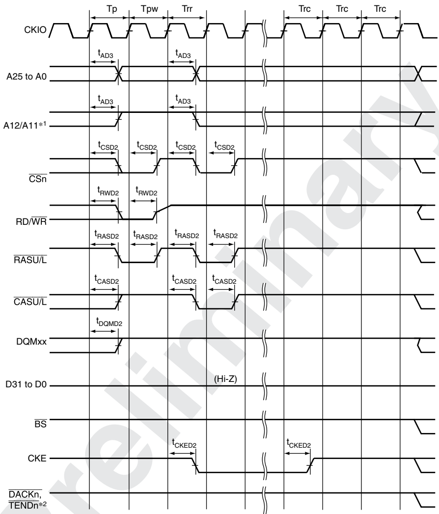
Figure 25.41 Synchronous DRAM Self-Refreshing Timing in Low-Frequency Mode (WTRP = 2 Cycles)
