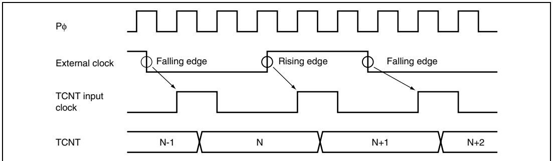
Figure 18.55 Count Timing in External Clock Operation
