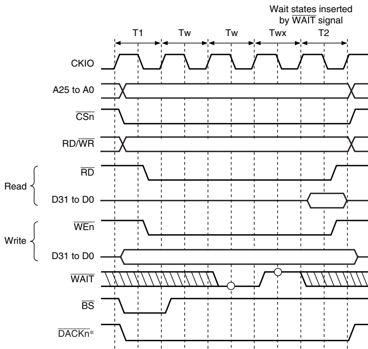
Figure 12.10 Wait State Timing for Normal Space Access (Wait State Insertion Using \overline{\text{WAIT}} Signal)
