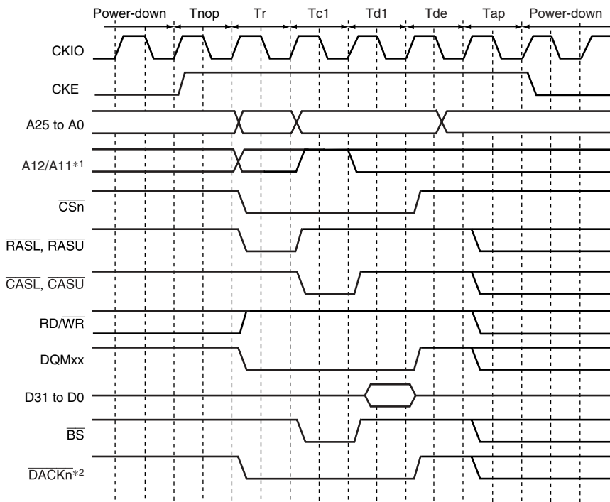
Figure 12.32 Power-Down Mode Access Timing
