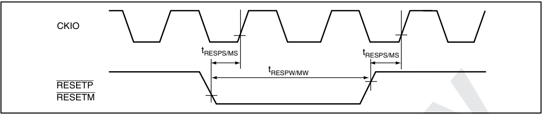
Figure 25.9 Reset Input Timing
