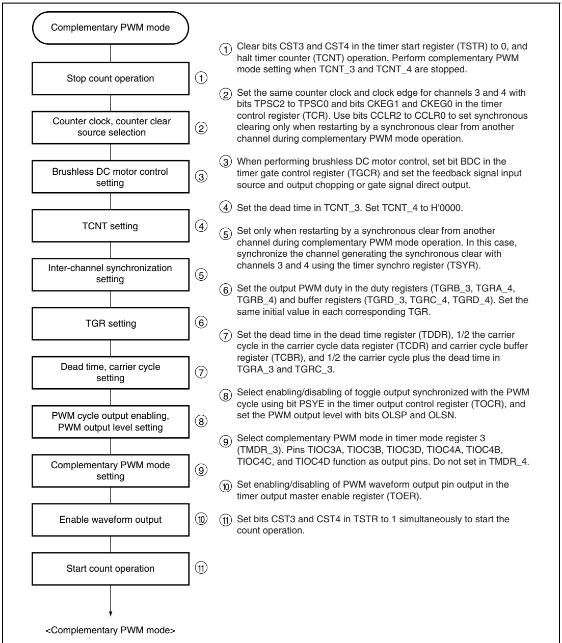
Figure 18.33 Example of Complementary PWM Mode Setting Procedure
