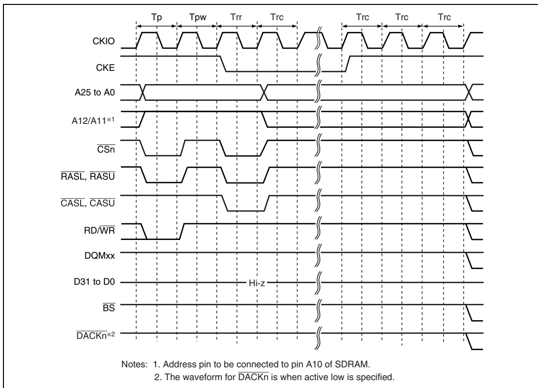
Figure 12.30 Self-Refresh Timing
