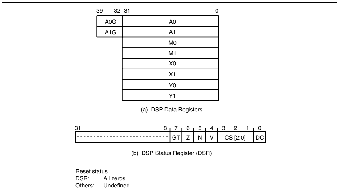
Figure 2.7 DSP Registers
