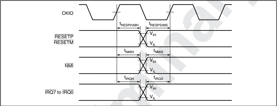
Figure 25.10 Interrupt Input Timing
