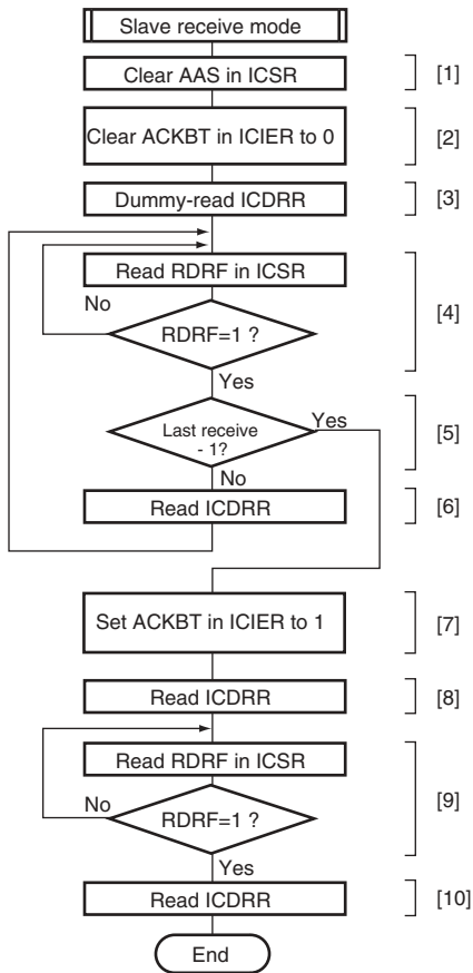
Figure 16.21 Sample Flowchart for Slave Receive Mode
