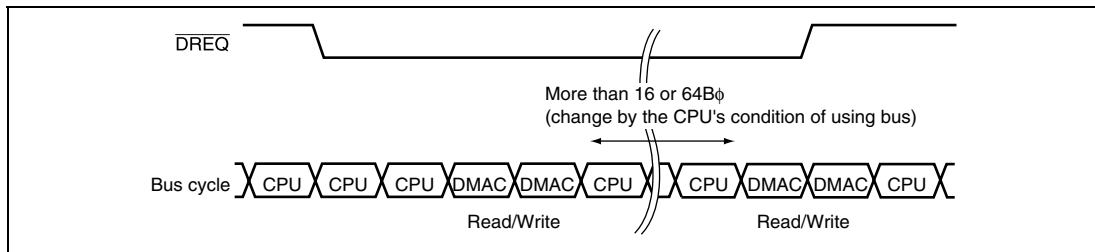
Figure 13.10 Example of DMA Transfer in Cycle Steal Intermittent Mode (Dual Address, \overline{\text{DREQ}} Low Level Detection)
