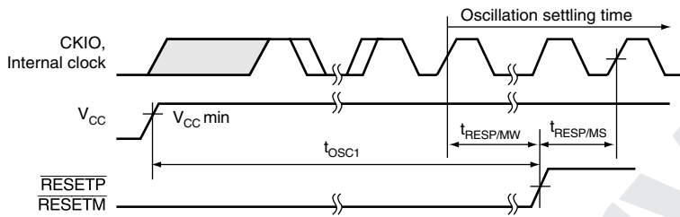
Figure 25.5 Oscillation Settling Timing (Power-On)
