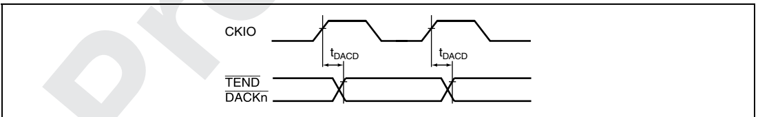
Figure 25.46 \overline{\text{DACK}} , \overline{\text{TEND}} Output Timing
