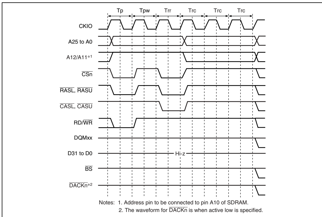
Figure 12.29 Auto-Refresh Timing
