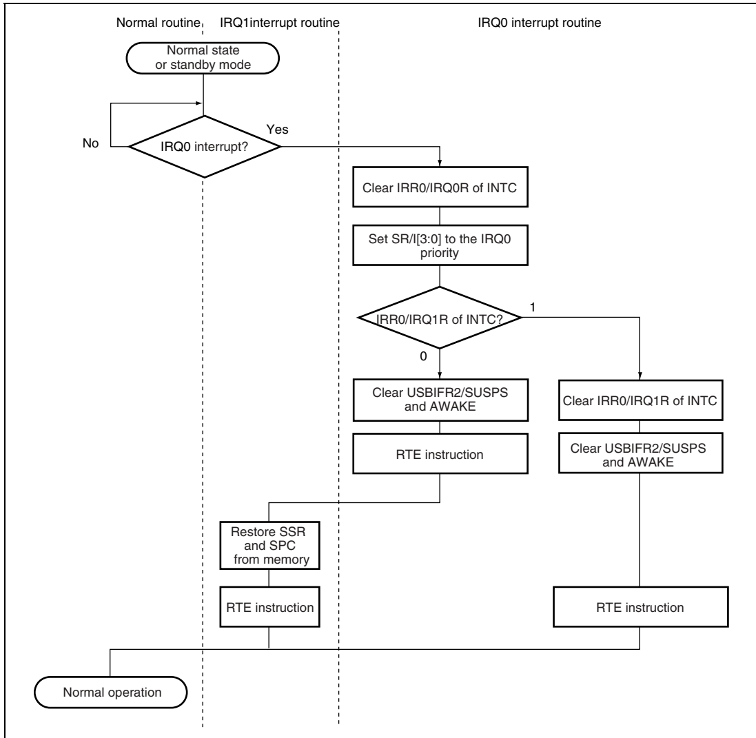
Figure 20.23 Sample Flowchart for AWAKE
