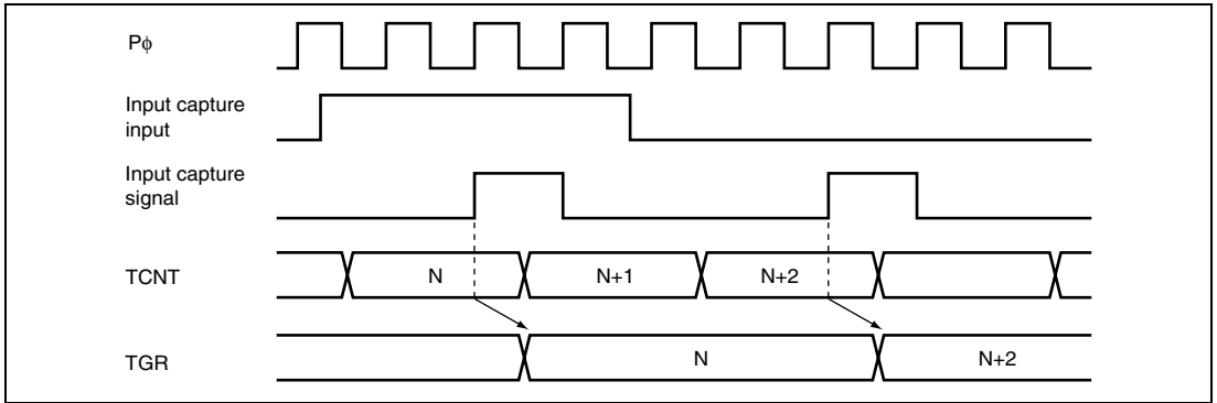
Figure 18.59 Input Capture Input Signal Timing
