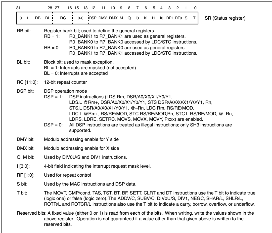
Figure 2.5 Control Registers (1)
