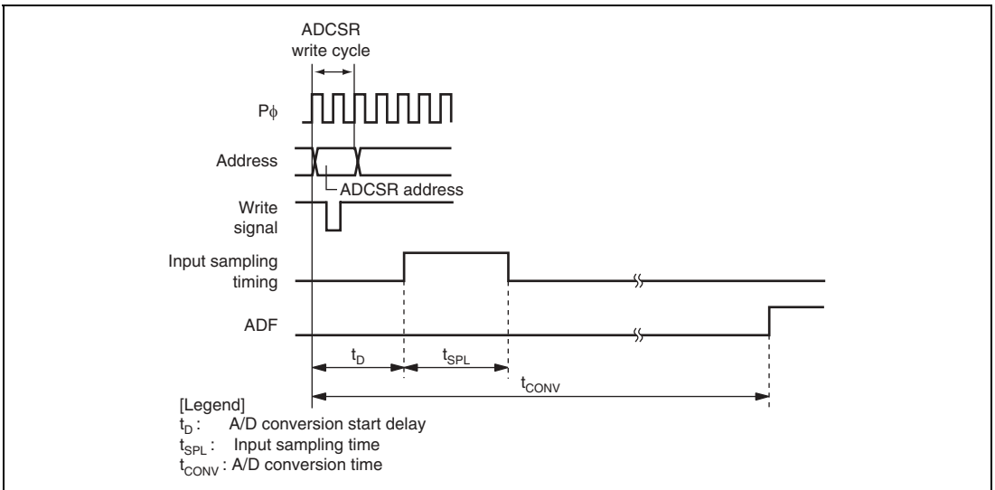
Figure 21.5 A/D Conversion Timing
