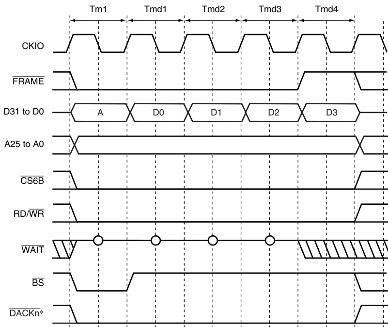
Figure 12.46 Burst MPX Space Access Timing (Burst Write, No Wait, CS6BWCR.MPXMD = 0)
