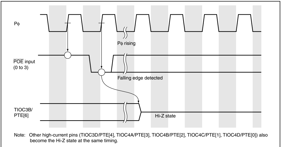
Figure 18.115 Falling Edge Detection Operation
