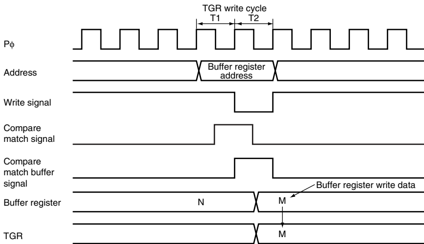
Figure 18.74 Conflict between Buffer Register Write and Compare Match (Channel 0)
