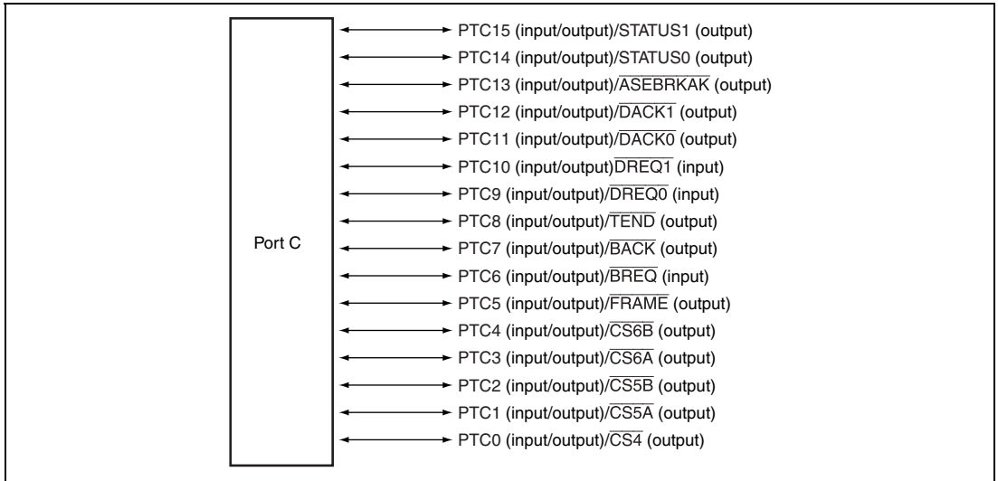
Figure 23.3 Port C
