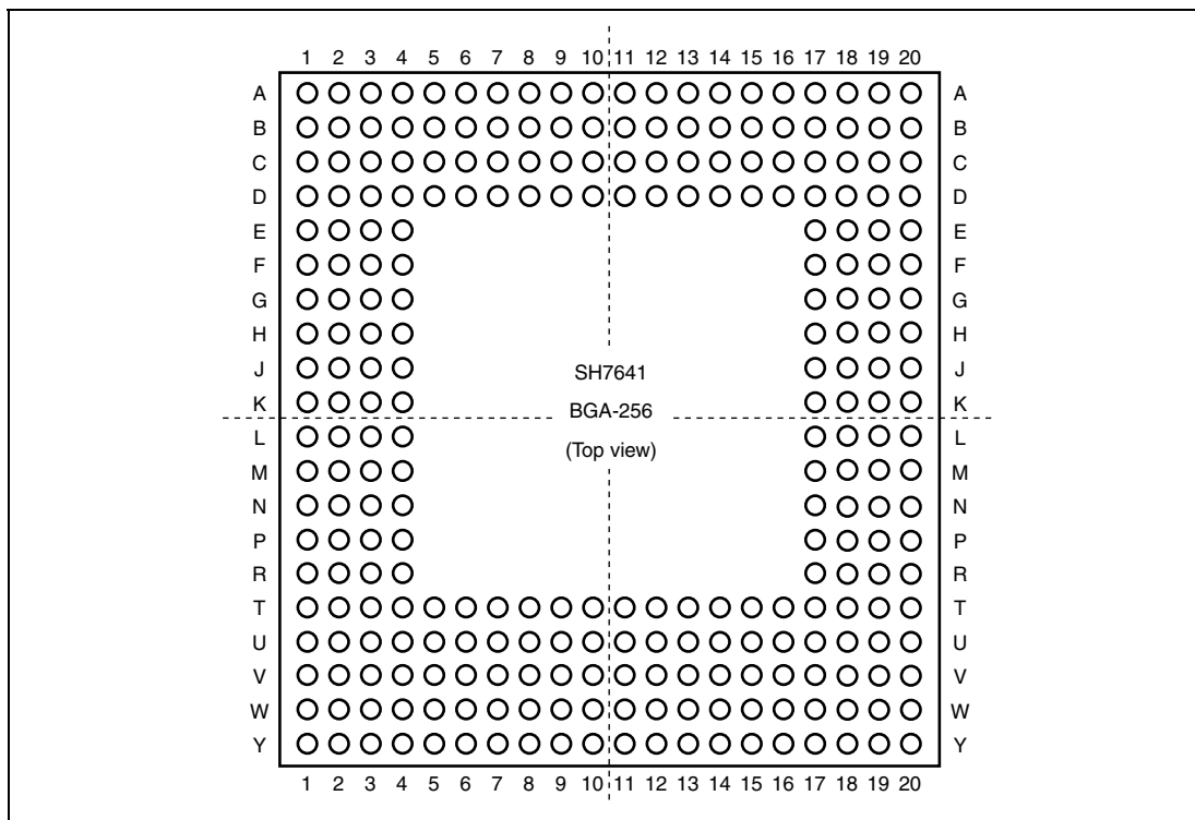
Figure 1.2 Pin Arrangement (BGA-256)
