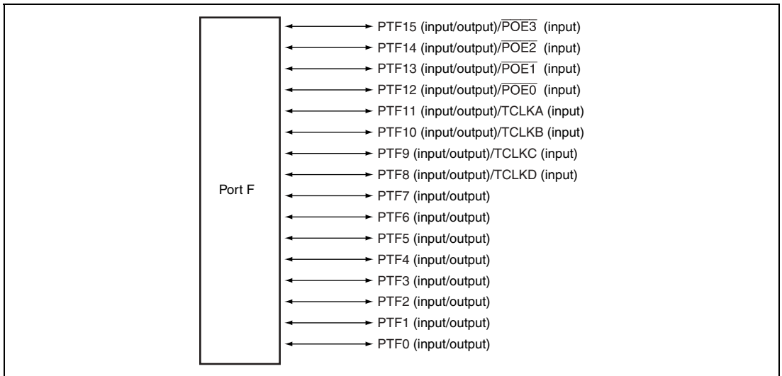
Figure 23.6 Port F
