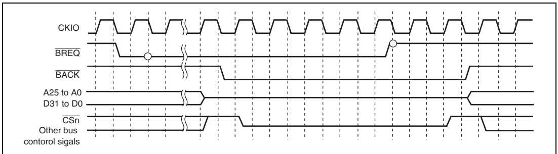
Figure 12.48 Bus Arbitration Timing (Clock Mode 7 or \text{CMNCR.HIZCNT} = 1 )
