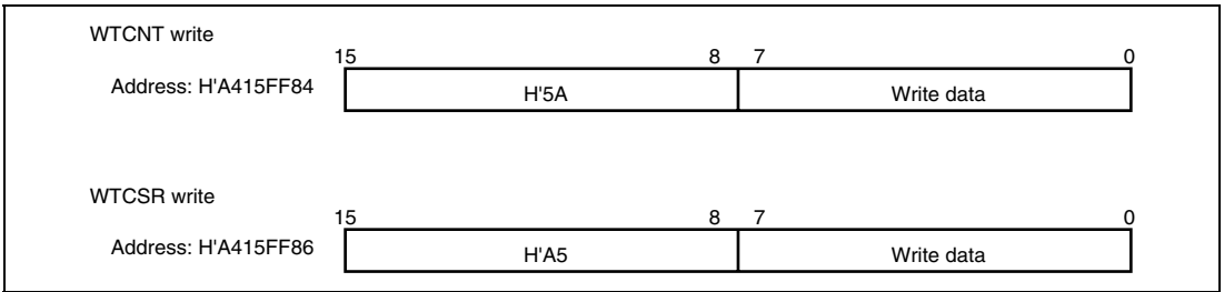
Figure 5.2 Writing to WTCNT and WTCSR
