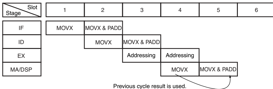
Figure 3.2 Operation Sequence Example
