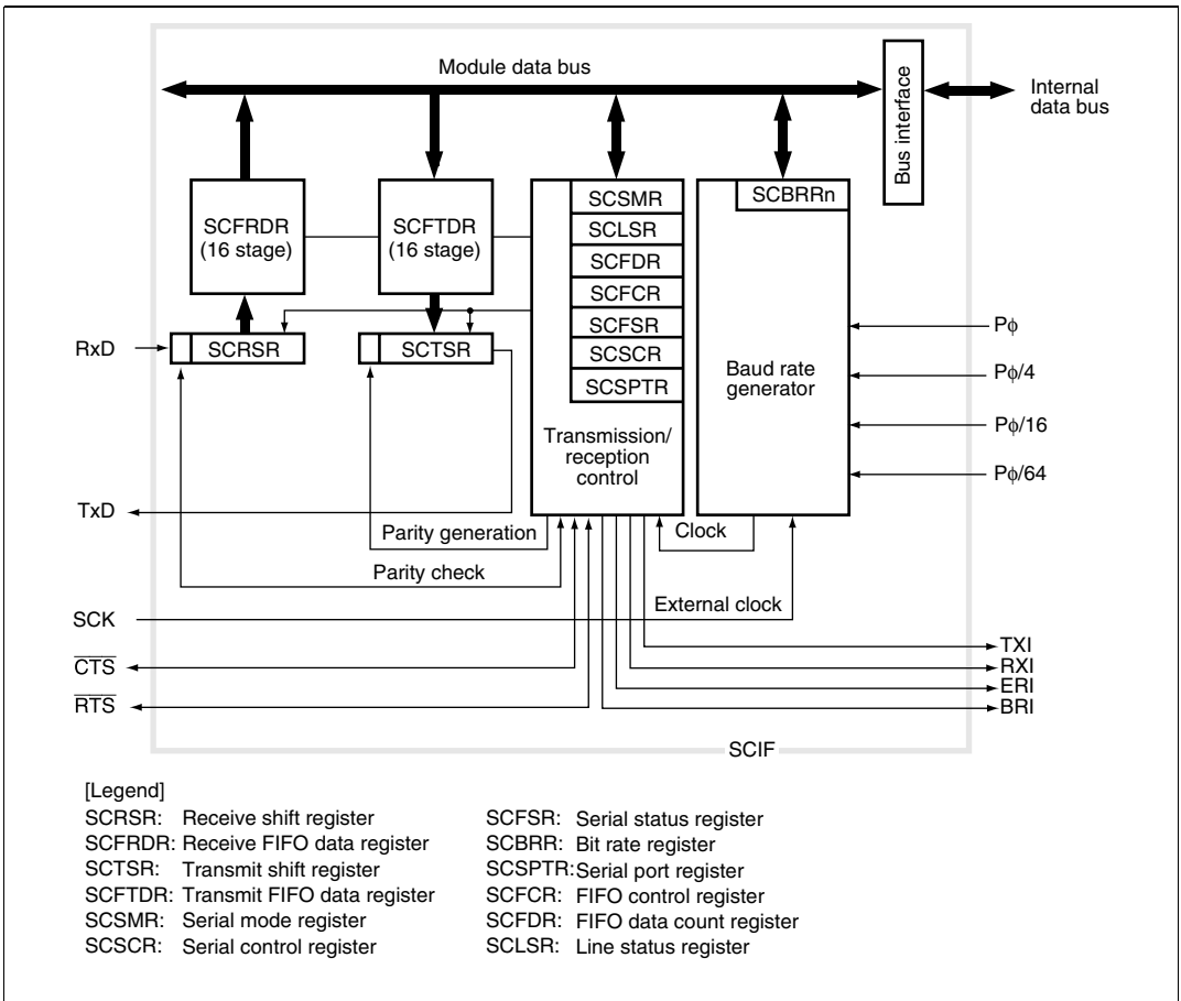
Figure 19.1 Block Diagram of SCIF
