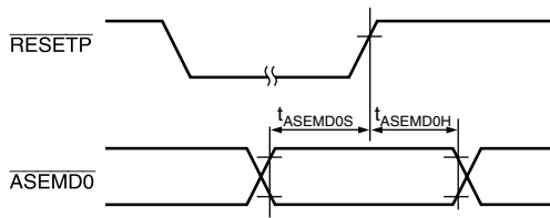
Figure 25.55 ASEMDO Input Timing
