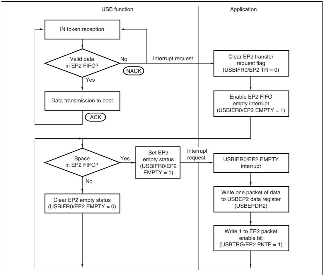
Figure 20.11 EP2 Bulk-IN Transfer Operation
