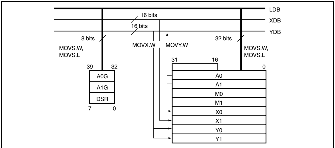
Figure 2.8 Connections of DSP Registers and Buses
