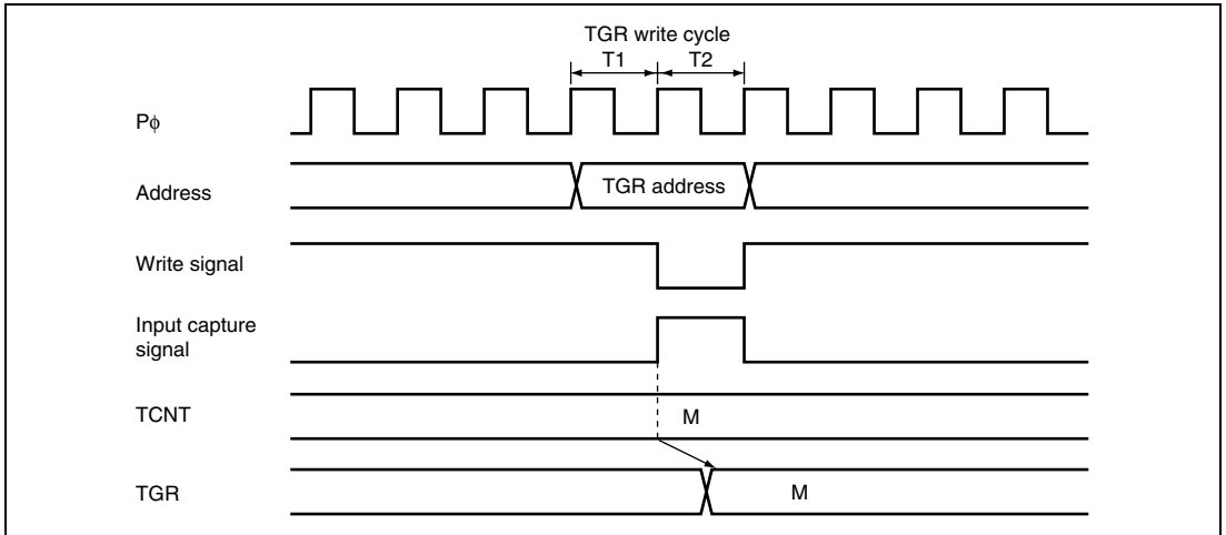
Figure 18.77 Conflict between TGR Write and Input Capture
