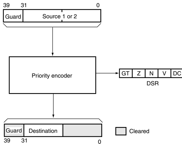
Figure 3.11 PDMSB Operation Flow
