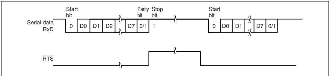
Figure 19.10 Example of Operation Using Modem Control ( \overline{\text{RTS}} )
