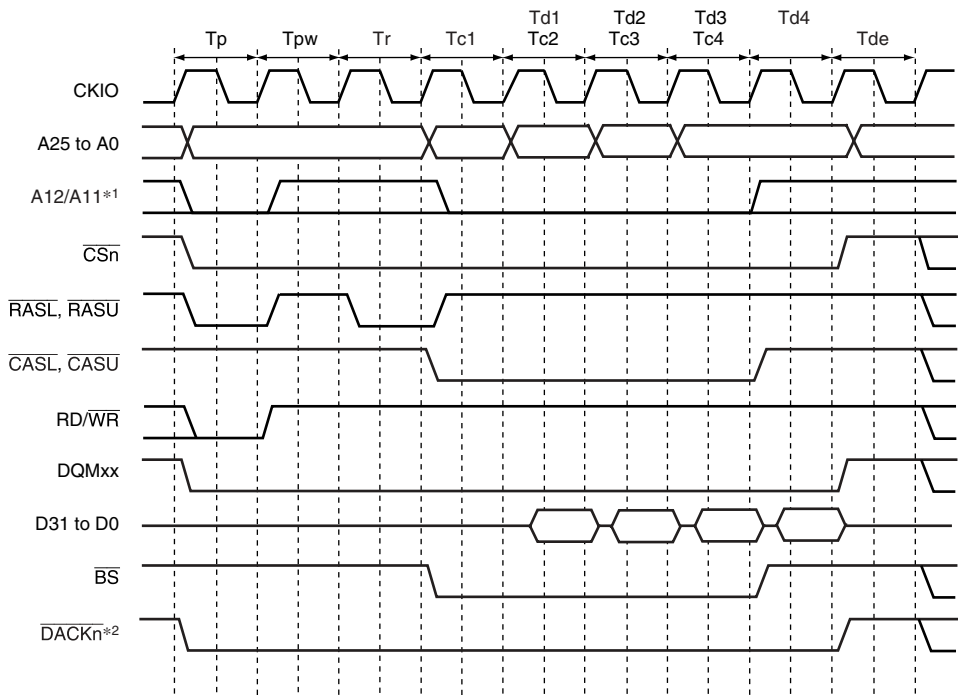
Figure 12.25 Burst Read Timing (Bank Active, Different Row Addresses in the Same Bank, CAS Latency 1)
