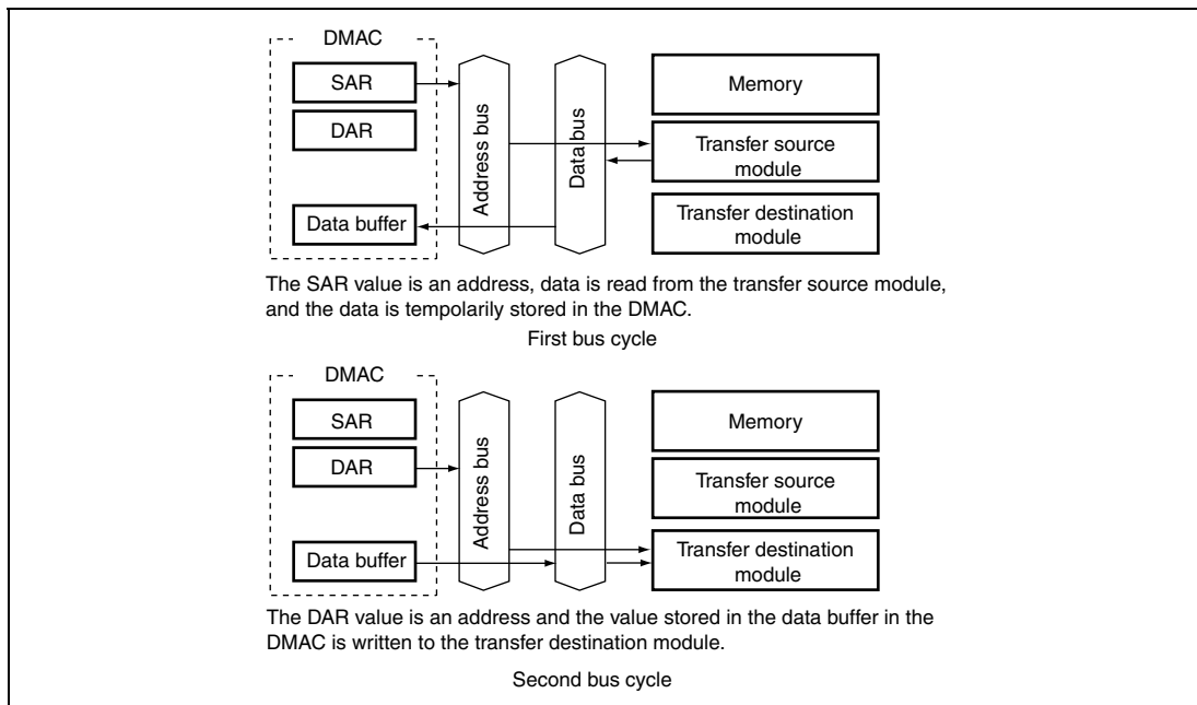
Figure 13.5 Data Flow of Dual Address Mode
