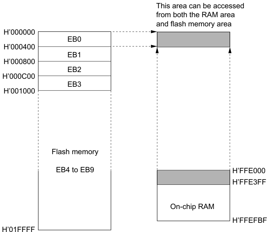
Figure 21A-16 Example of RAM Overlap Operation
