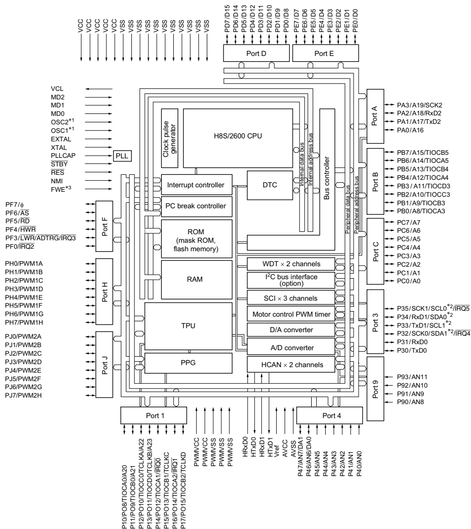
Figure 1-1 (b) shows an internal block diagram of the H8S/2638, H8S/2639, and H8S/2630.
