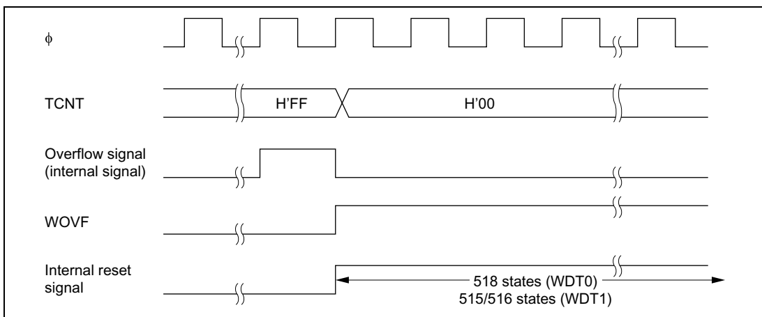
Figure 12-7 Timing of Setting of WOVSF
