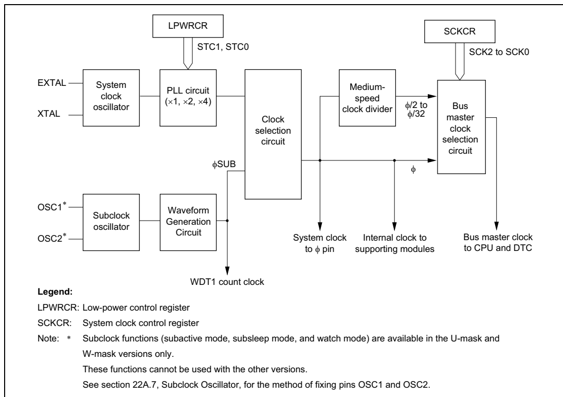
Figure 22A-1 Block Diagram of Clock Pulse Generator
