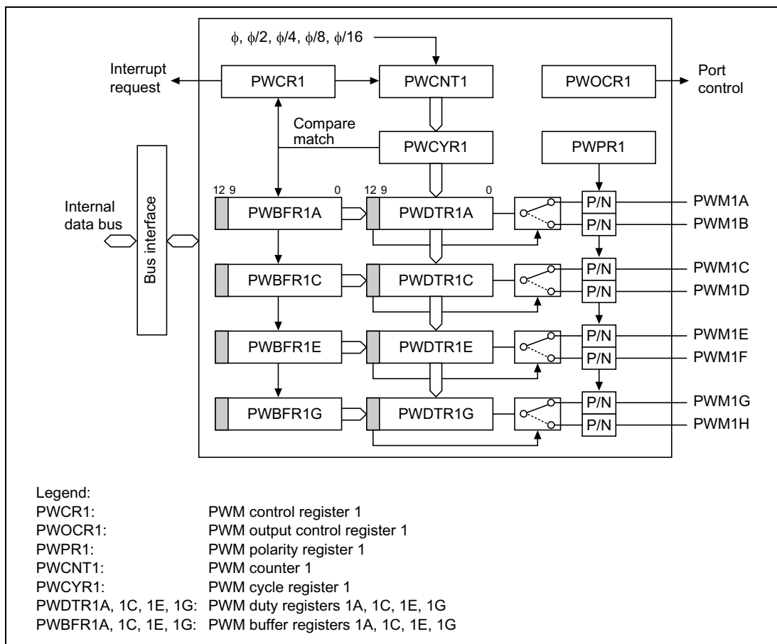
Figure 19-1 Block Diagram of PWM Channel 1
