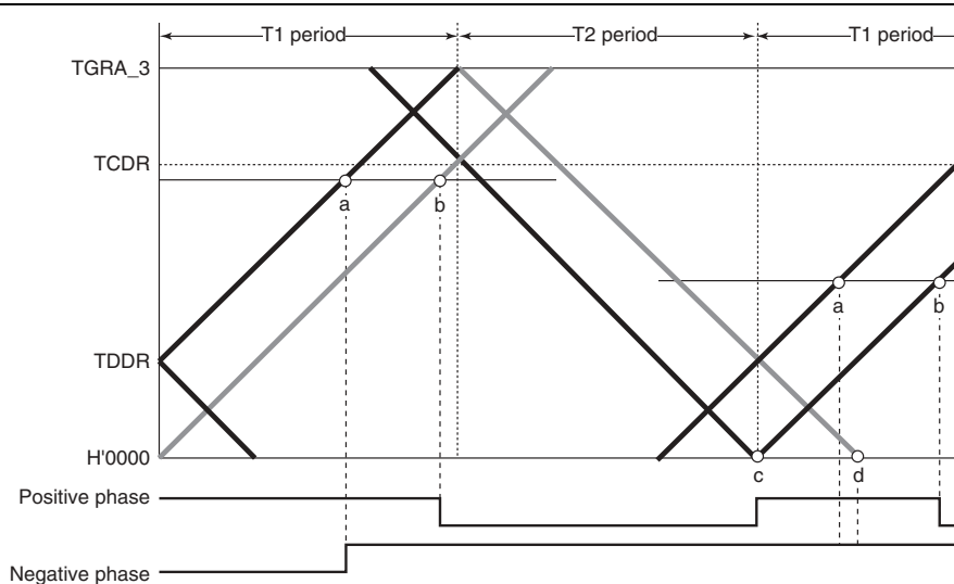
Figure 11.44 Example of Complementary PWM Mode 0% and 100% Waveform Output (2)
