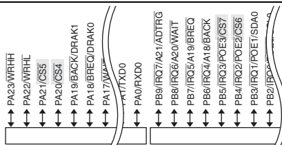
Figure 1.2 Block Diagram of SH7145
