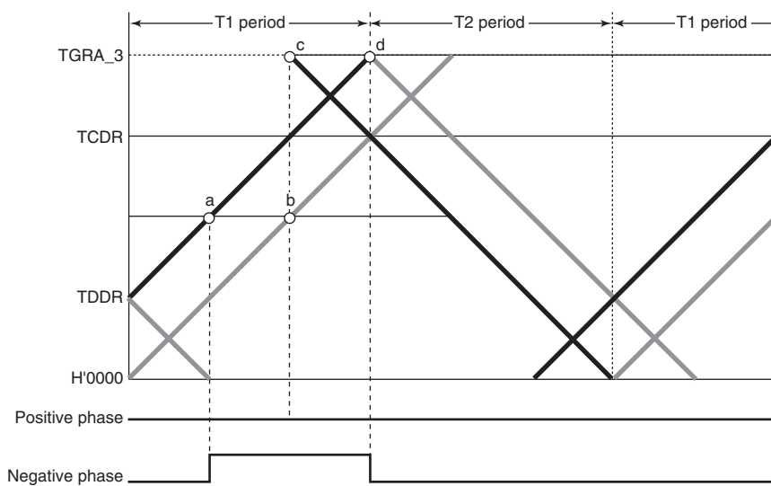
Figure 11.45 Example of Complementary PWM Mode 0% and 100% Waveform Output (3)
