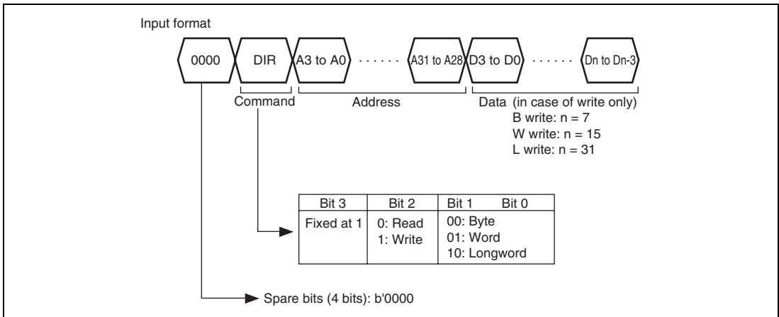
Figure 23.4 AUDATA Input Format
