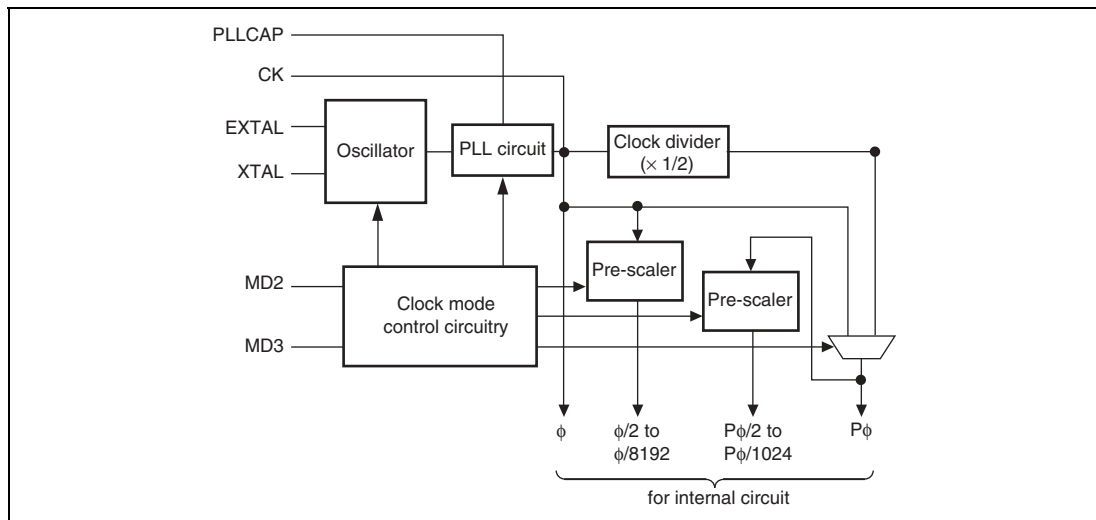
Figure 4.1 Block Diagram of Clock Pulse Generator
