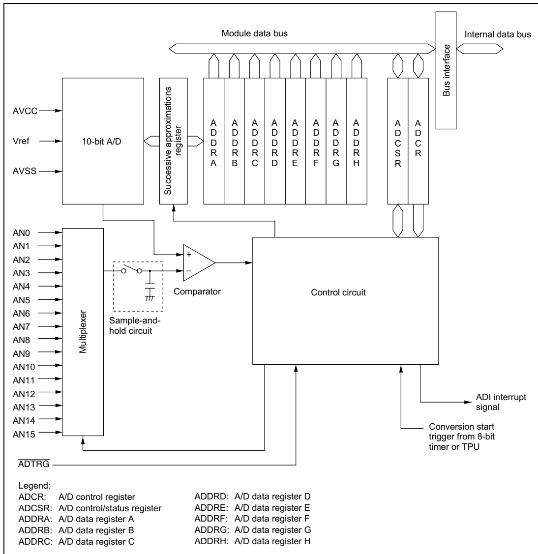
Figure 17.1 Block Diagram of A/D Converter
