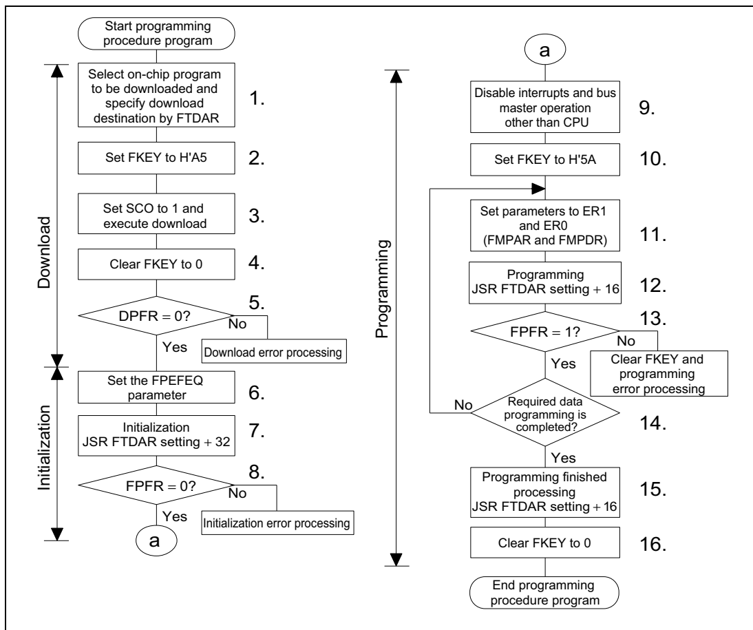
Figure 21.11 Programming Procedure
