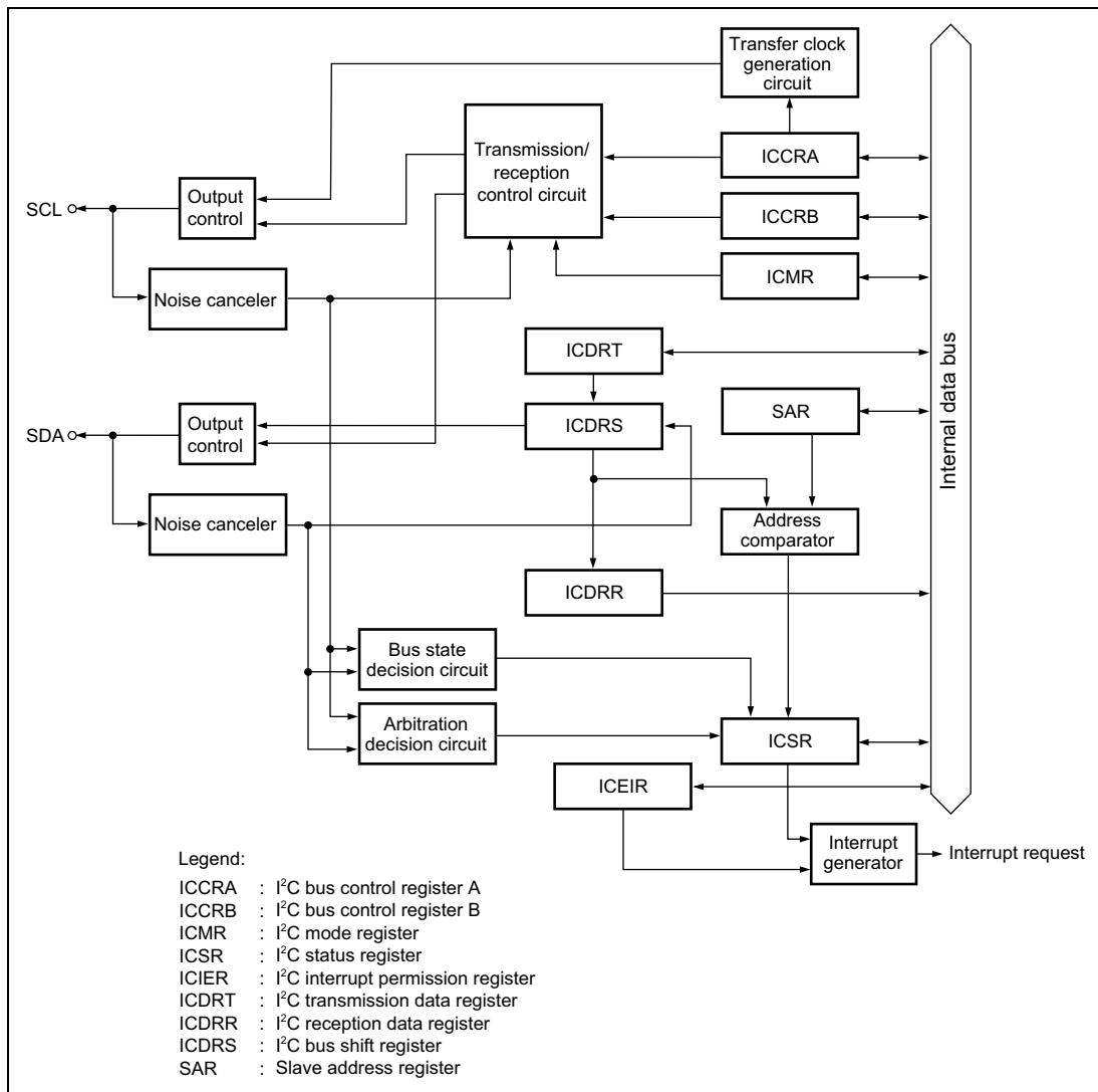
Figure 16.1 Block Diagram of I²C Bus Interface2
