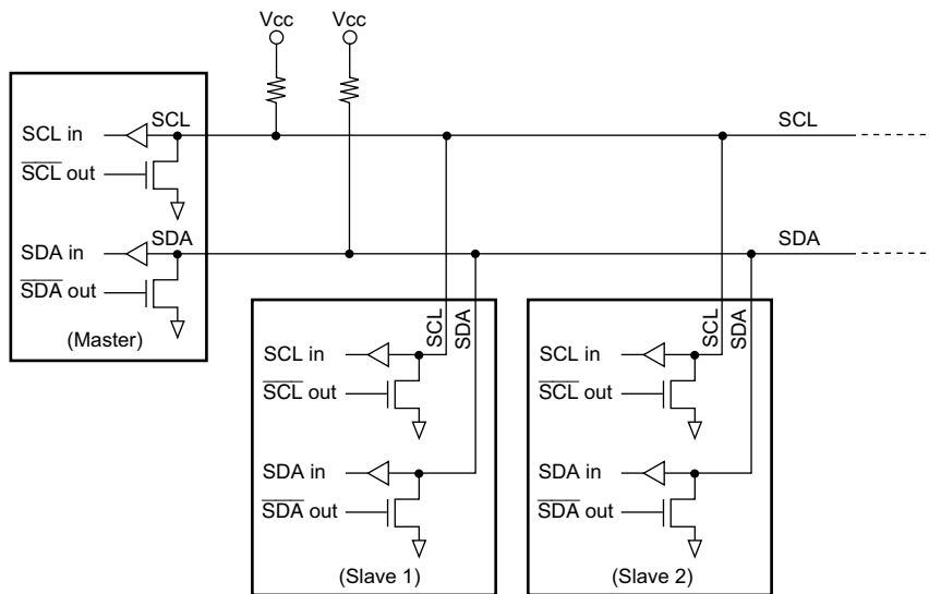
Figure 16.2 External Circuit Connections of I/O Pins
