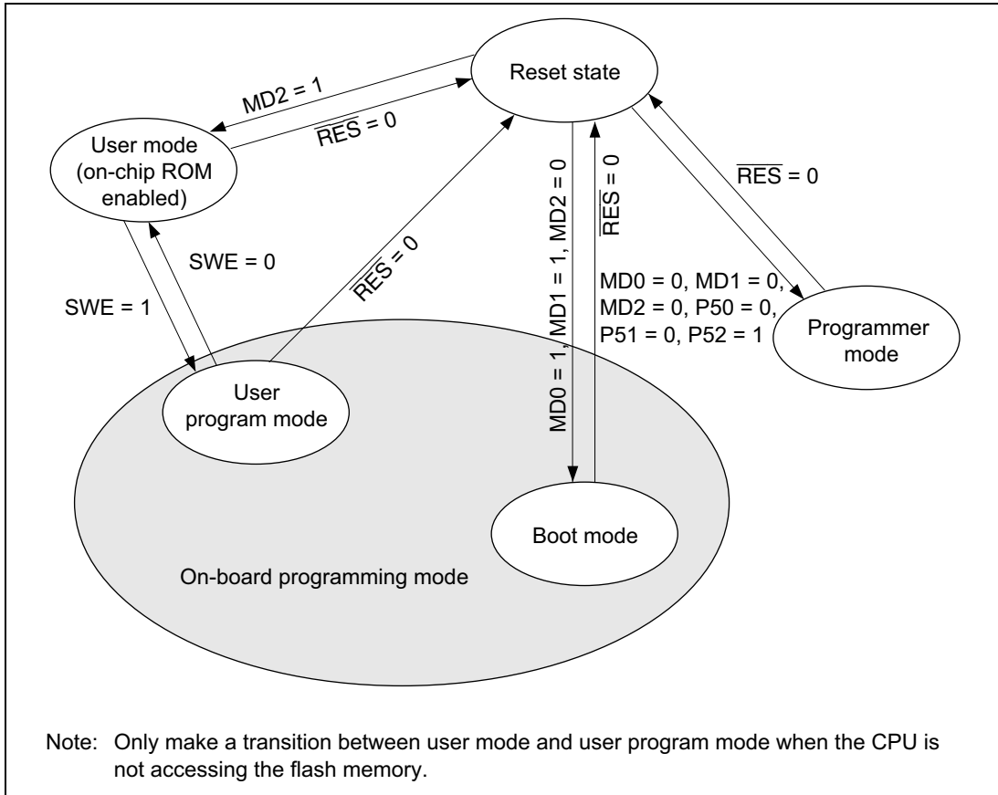
Figure 20.2 Flash Memory State Transitions
