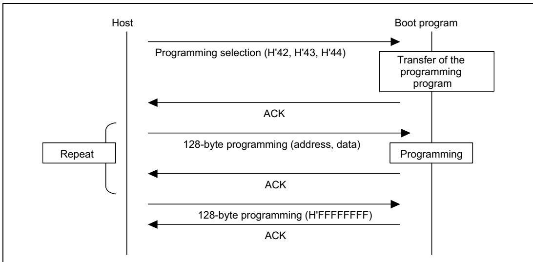
Figure 21.21 Programming Sequence
