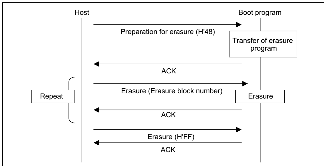
Figure 21.22 Erasure Sequence
