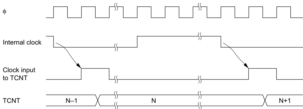
Figure 13.3 Count Timing for Internal Clock Input
