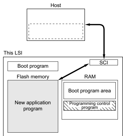
Figure 20.3 Boot Mode
