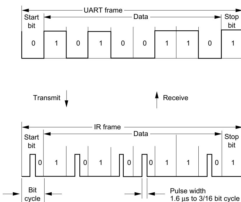
Figure 15.34 IrDA Transmit/Receive Operations
