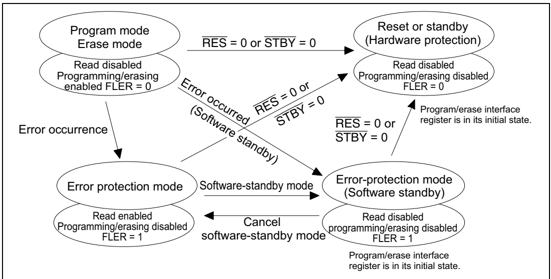
Figure 21.15 Transitions to Error-Protection State
