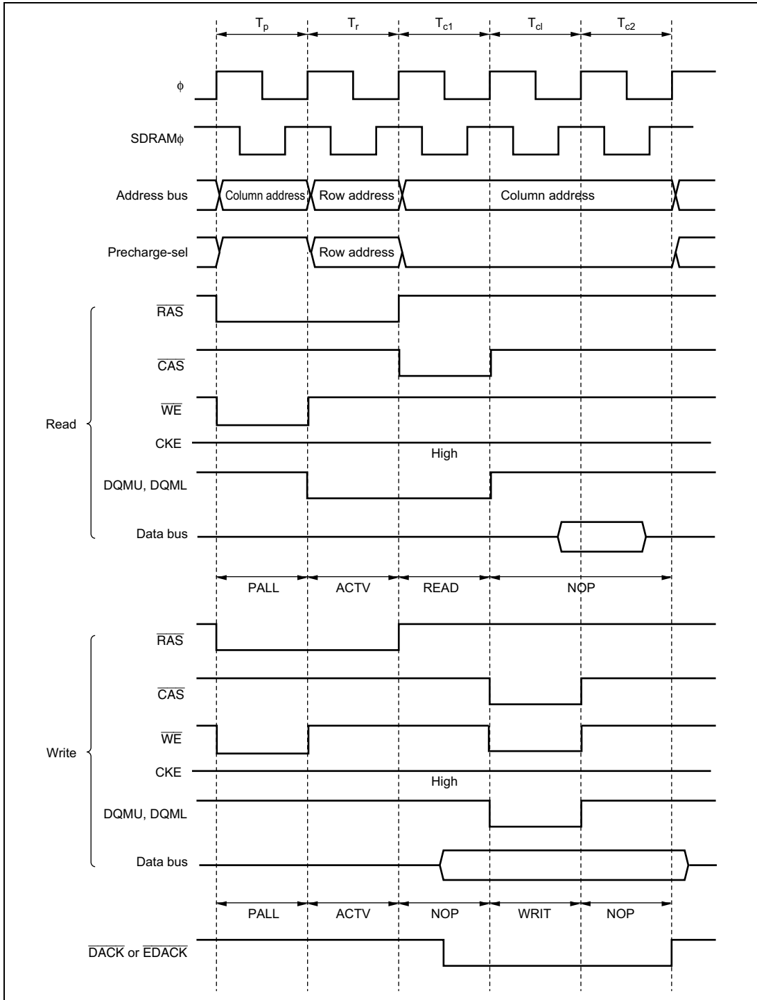
Figure 6.60 Example of \overline{DACK}/\overline{EDACK} Output Timing when DDS = 1 or EDDS = 1
