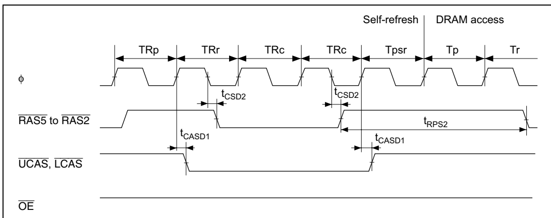
Figure 26.21 Self-Refresh Timing (Return from Software Standby Mode: \text{RAST} = 0 )
