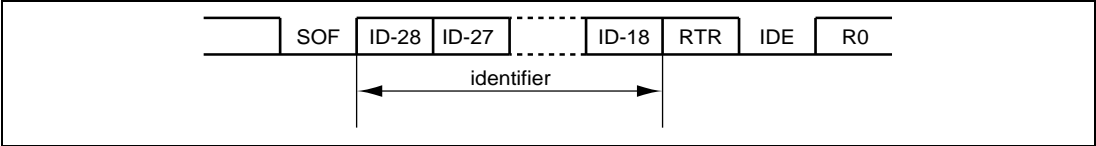
Figure 15.3 Standard Format
