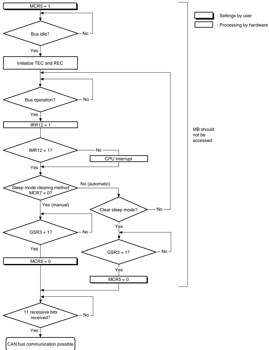
Figure 15.13 HCAN Sleep Mode Flowchart
