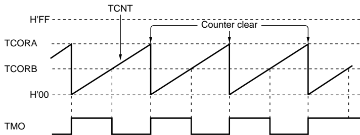
Figure 11.2 Example of Pulse Output
