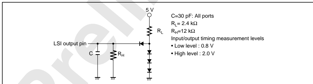
Figure 23.1 Output Load Circuit
