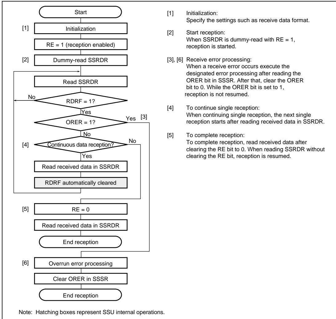
Figure 16.8 Example of Data Reception Flowchart
