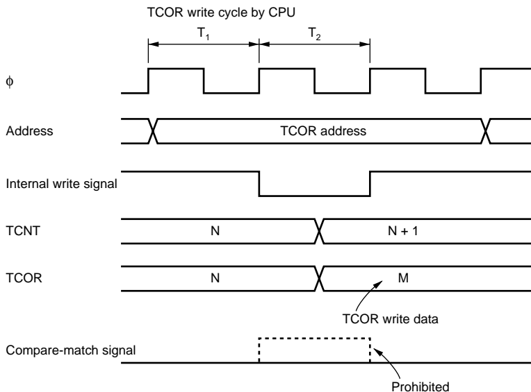
Figure 11.12 Conflict between TCOR Write and Compare-Match
