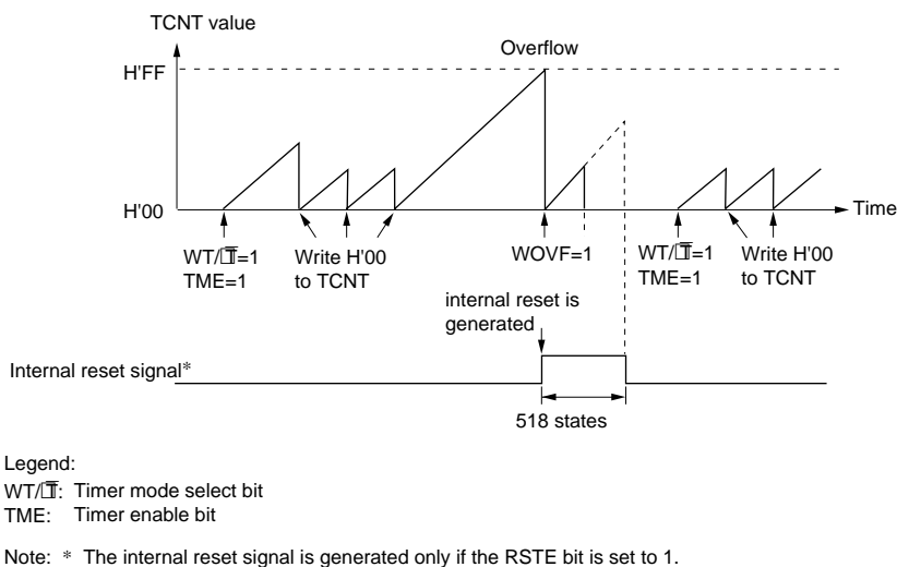
Figure 13.2 Example of WDT0 Watchdog Timer Operation
