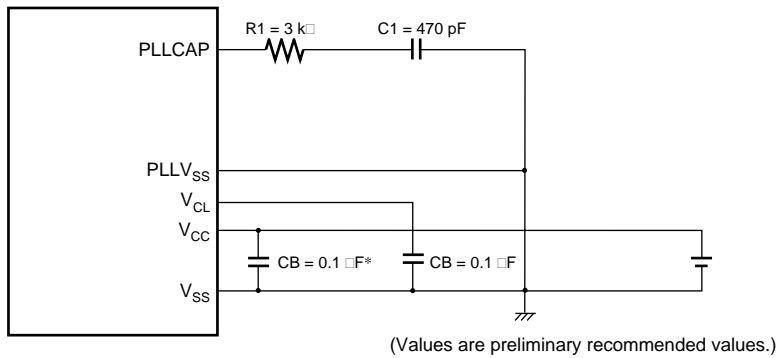
Figure 20.7 External Circuitry Recommended for PLL Circuit
