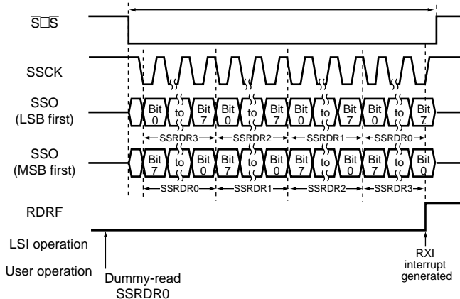
Figure 16.7 Example of Reception Operation
