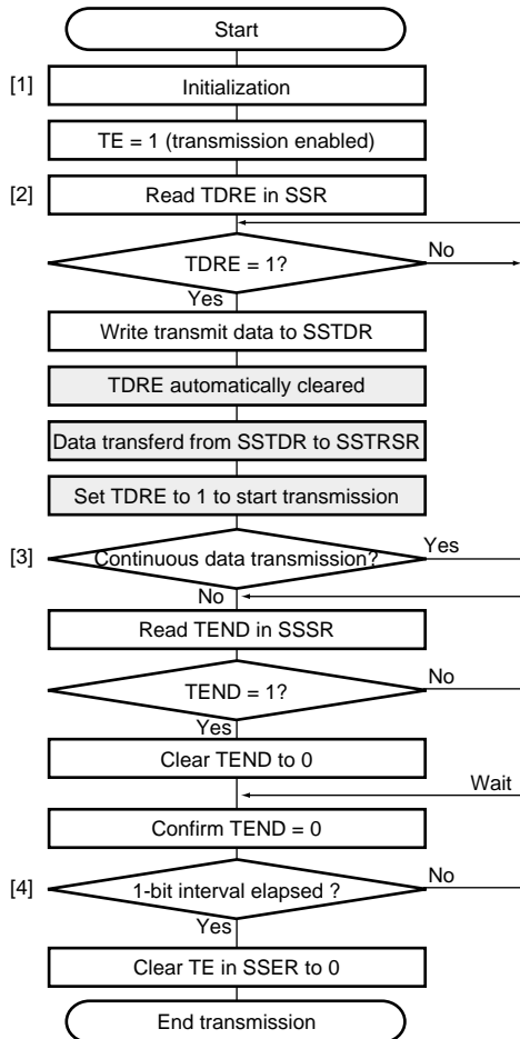
Figure 16.6 Example of Data Transmission Flowchart
