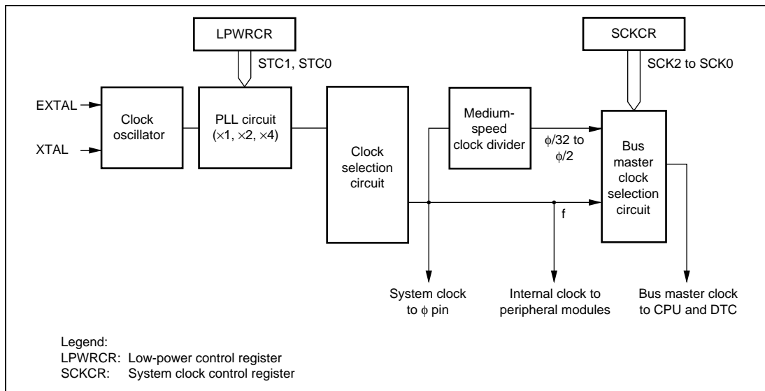
Figure 20.1 Block Diagram of Clock Pulse Generator
