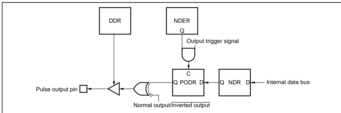
Figure 12.2 PPG Output Operation
