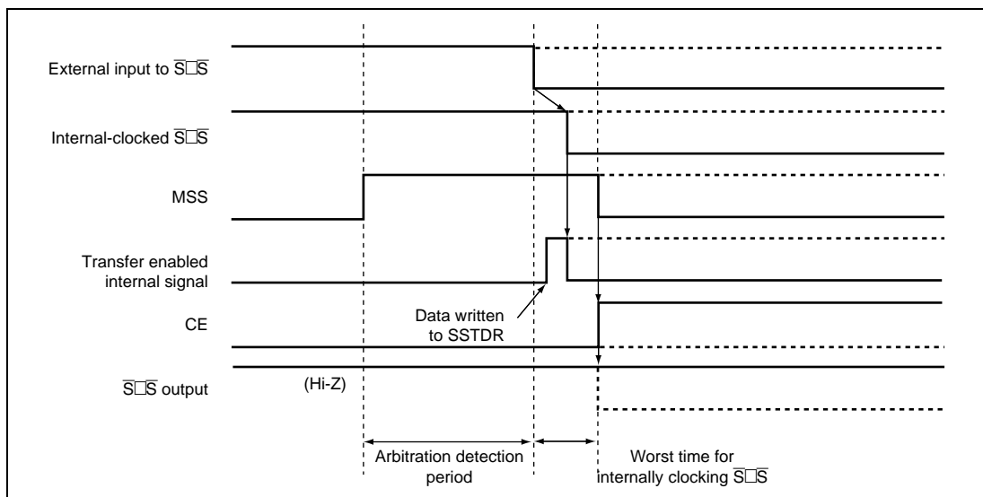
Figure 16.10 Arbitration Detection Timing (Before Transfer Start)
