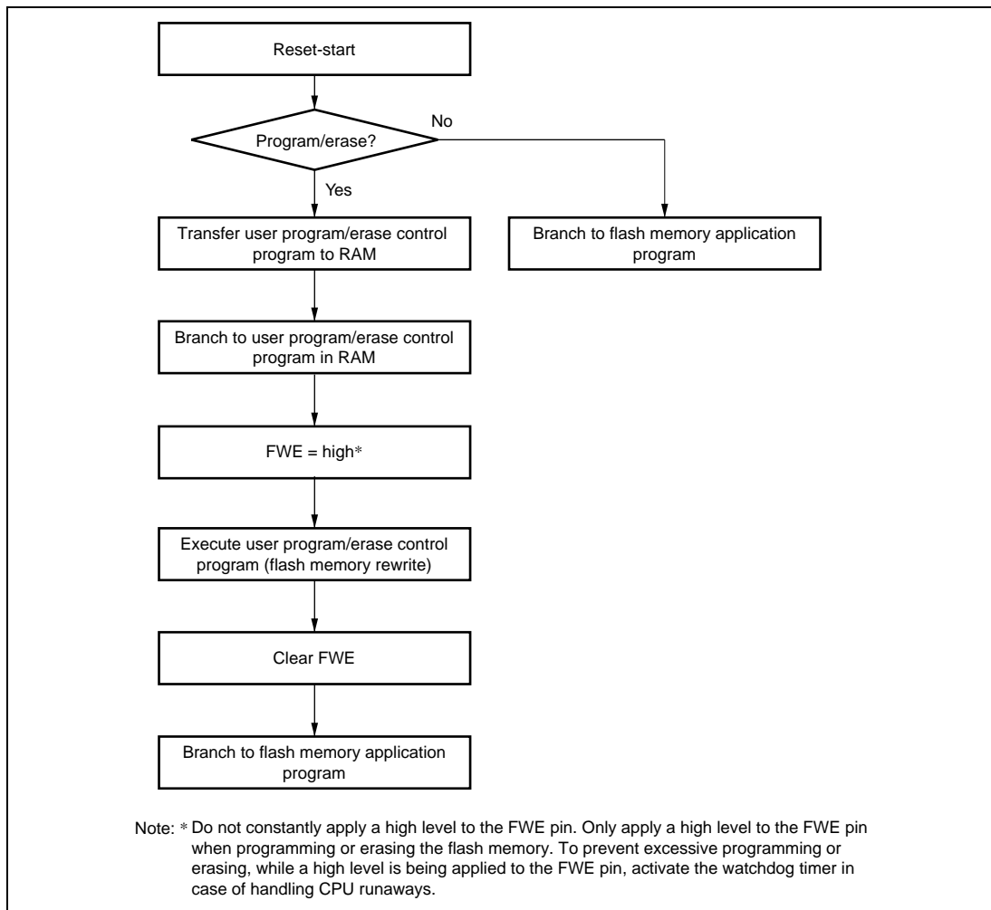
Figure 19.6 Programming/Erasing Flowchart Example in User Program Mode
