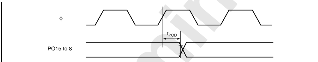
Figure 23.14 PPG Output Timing
