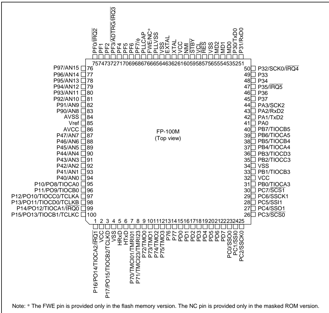
Figure 1.2 Pin Arrangement
