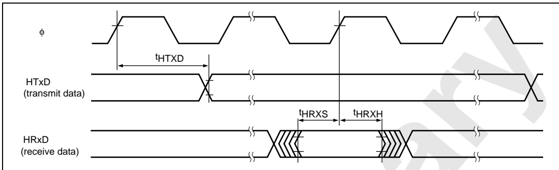
Figure 23.13 HCAN Input/Output Timing
