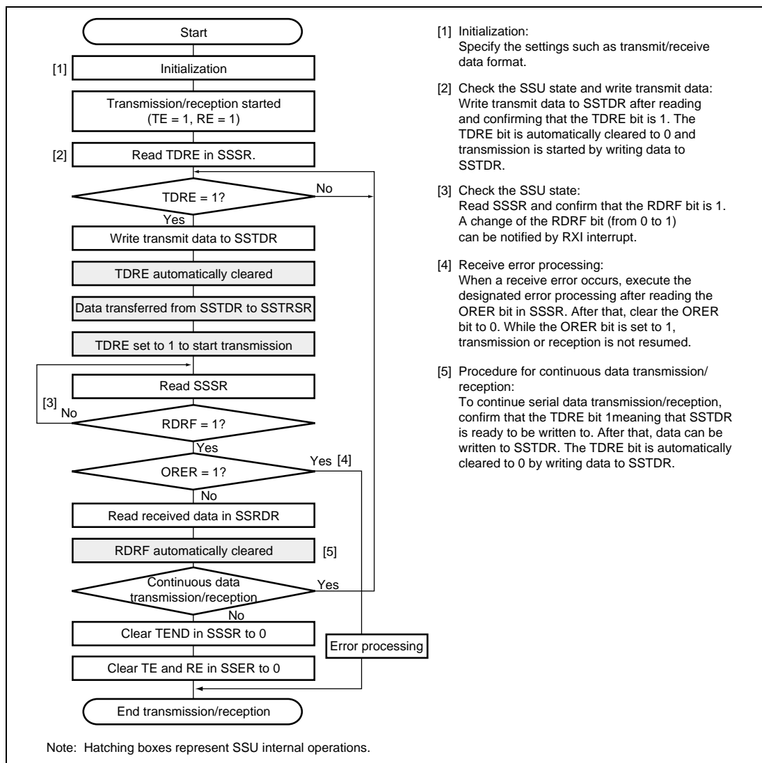
Figure 16.9 Example of Simultaneous Transmission/Reception Flowchart
