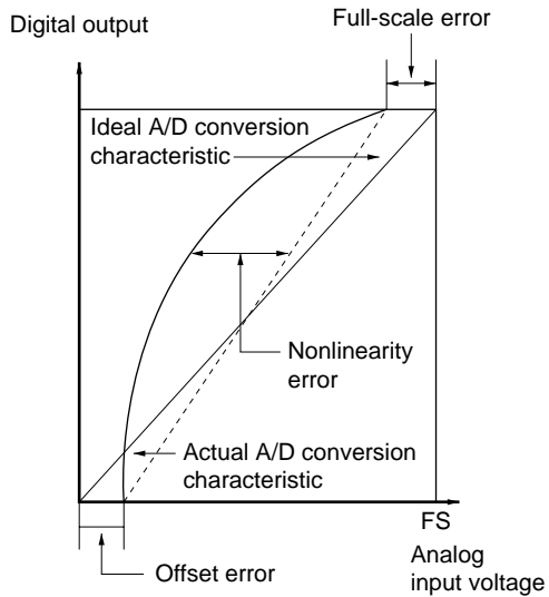
Figure 17.5 A/D Conversion Accuracy Definitions
