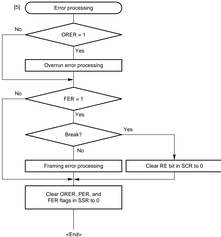
Figure 14.13 Sample Multiprocessor Serial Reception Flowchart (2)
