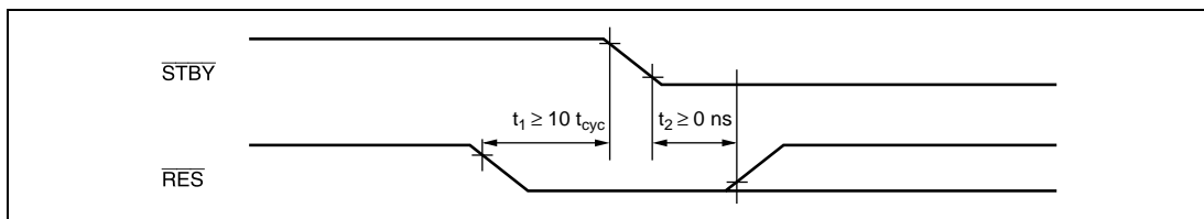
Figure 21.4 Timing of Transition to Hardware Standby Mode
