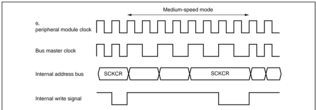
Figure 21.2 Medium-Speed Mode Transition and Clearance Timing
