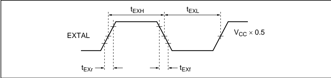
Figure 20.5 External Clock Input Timing
