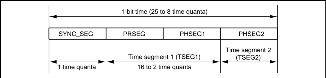
Figure 15.8 Detailed Description of One Bit
