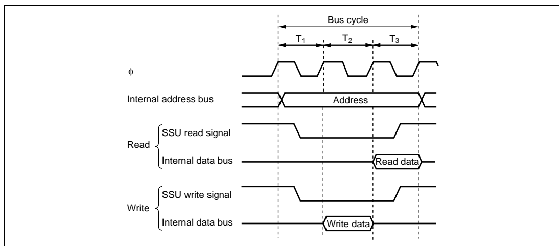
Figure 7.4 On-Chip SSU Module Access Cycle
