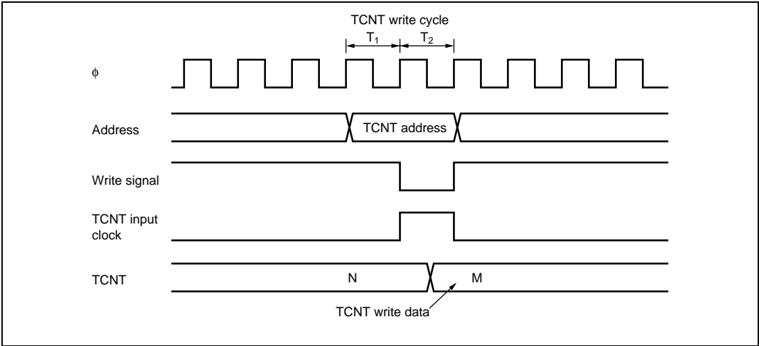
Figure 10.46 Conflict between TCNT Write and Increment Operations
