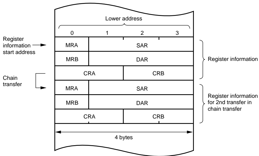
Figure 8.3 Location of DTC Register Information in Address Space
