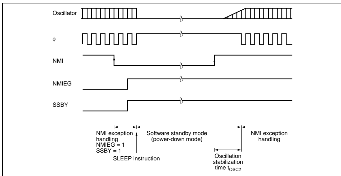
Figure 21.3 Software Standby Mode Application Example
