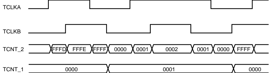
Figure 10.19 Example of Cascaded Operation (2)
