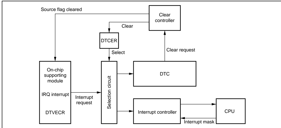
Figure 8.2 Block Diagram of DTC Activation Source Control
