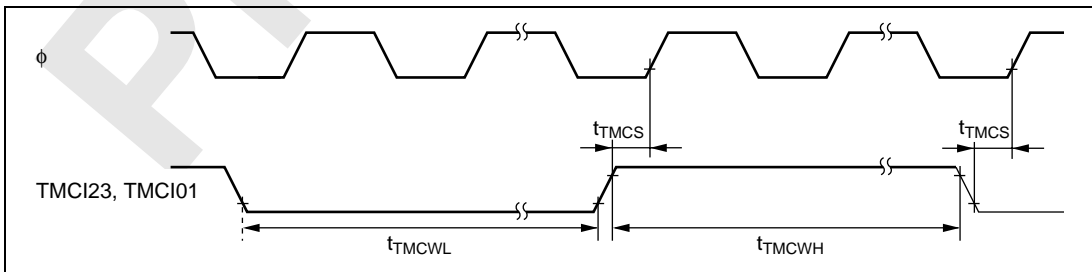
Figure 23.16 8-Bit Timer Clock Input Timing
