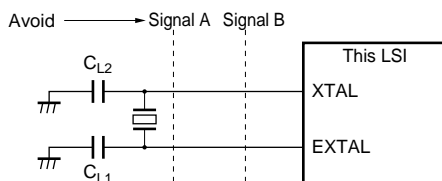
Figure 20.6 Note on Board Design of Oscillator Circuit
