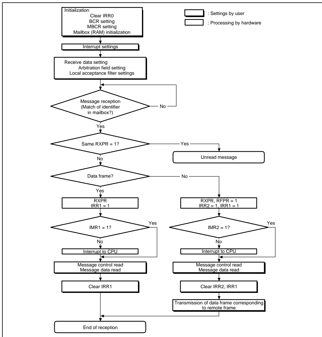
Figure 15.11 Reception Flowchart
