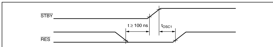
Figure 21.5 Timing of Recovery from Hardware Standby Mode
