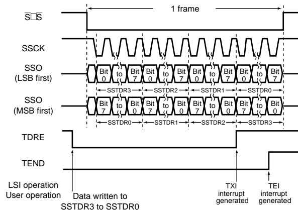
Figure 16.5 Example of Transmission Operation
