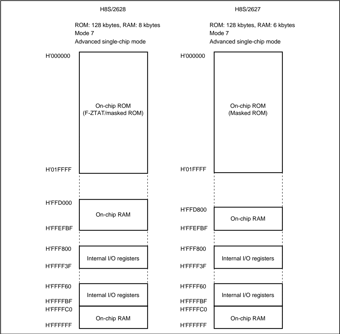
Figure 3.1 Address Map
