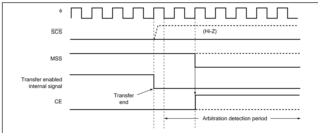
Figure 16.11 Arbitration Detection Timing (After Transfer End)
