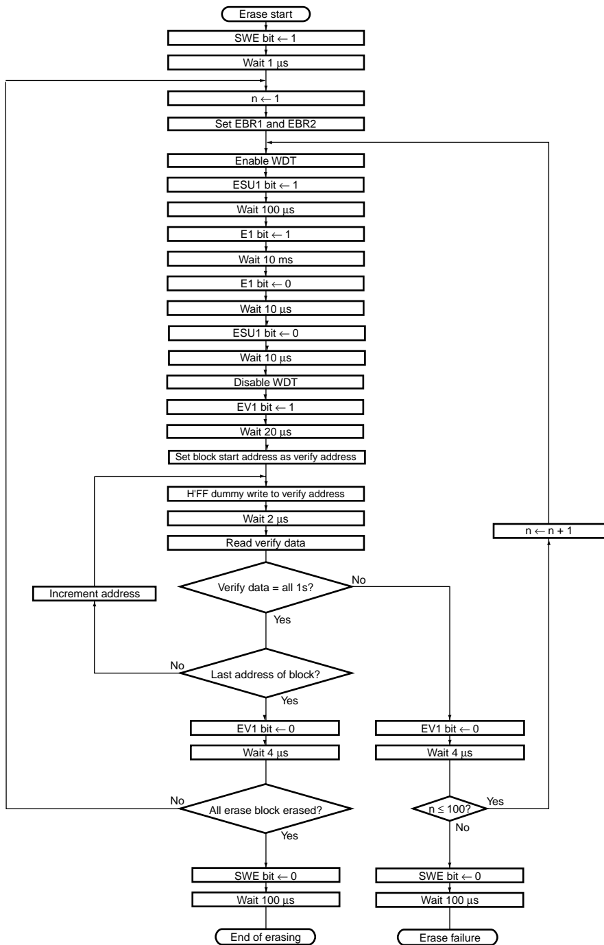
Figure 19.10 Erase/Erase-Verify Flowchart
