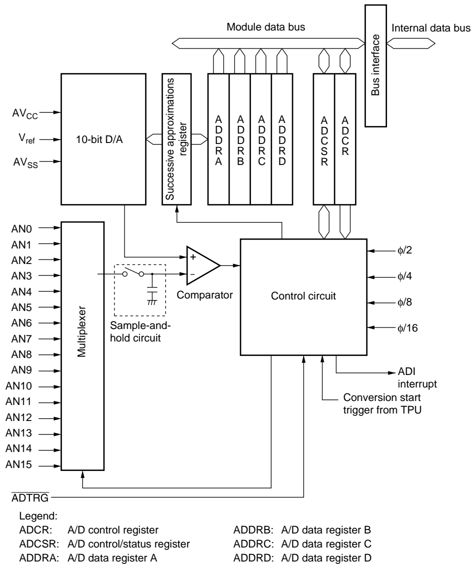
Figure 17.1 Block Diagram of A/D Converter
