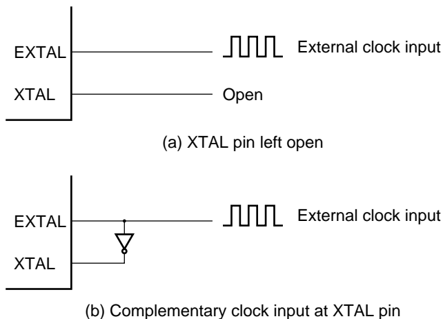
Figure 20.4 External Clock Input (Examples)
