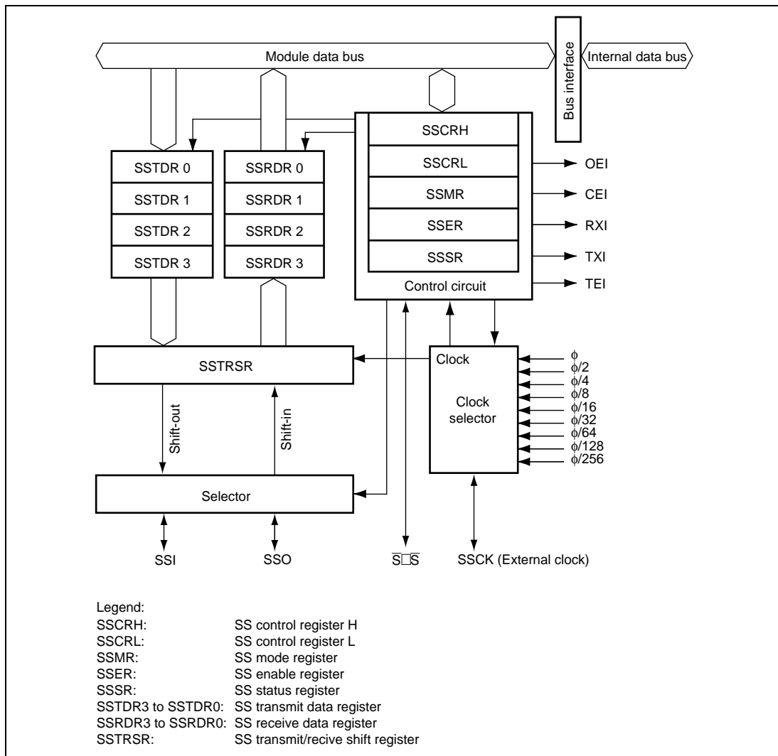
Figure 16.1 Block Diagram of SSU
