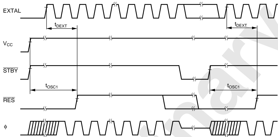
Figure 23.3 Oscillation Settling Timing
