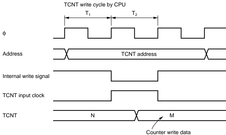
Figure 11.11 Conflict between TCNT Write and Increment
