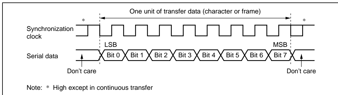
Figure 14.14 Data Format in Synchronous Communication (For LSB-First)
