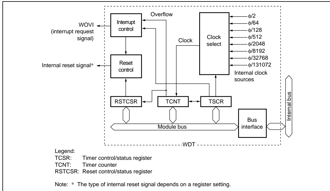
Figure 13.1 Block Diagram of WDT
