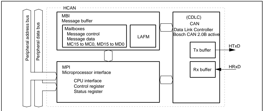
Figure 15.1 HCAN Block Diagram
