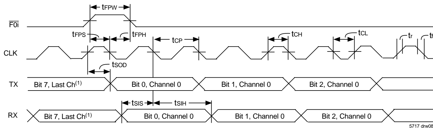
Figure 8. GCI Timing
