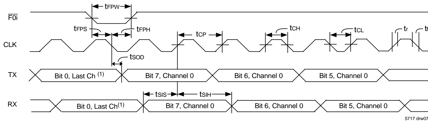
Figure 7. ST-BUS® Timing
