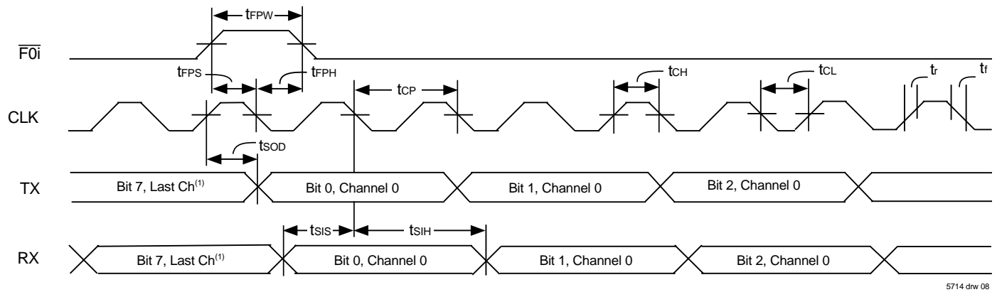
Figure 5. GCI Timing
