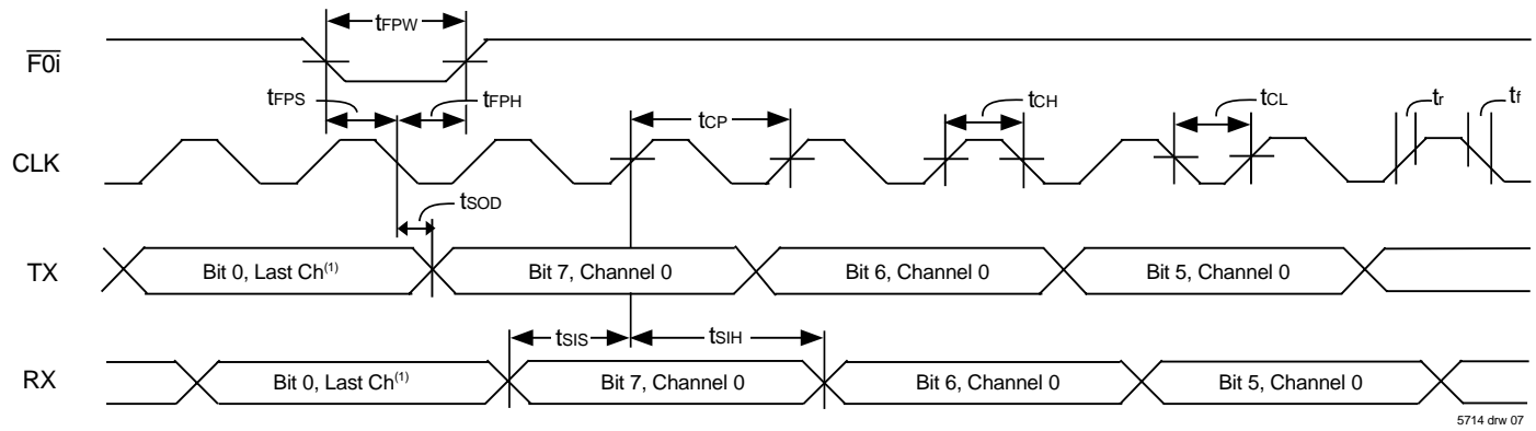
Figure 4. ST-BUS® Timing
