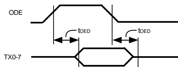
Figure 8. Output Driver Enable
