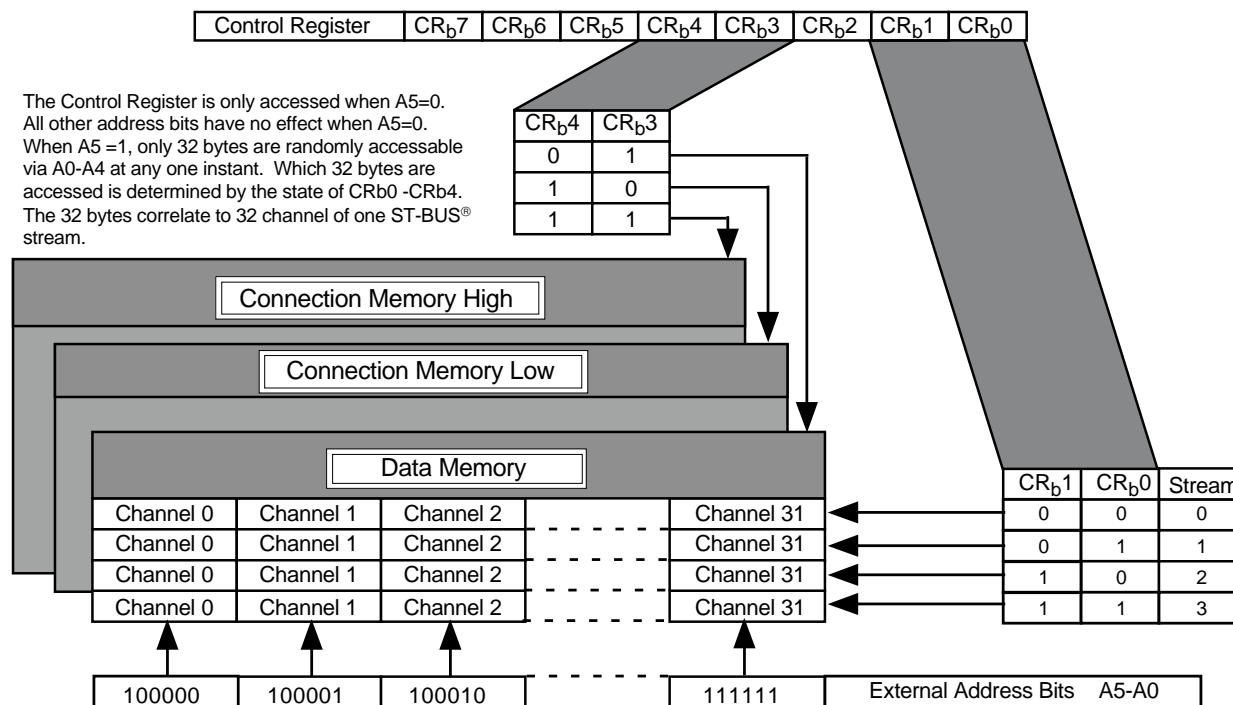
Figure 3. Address Mapping
