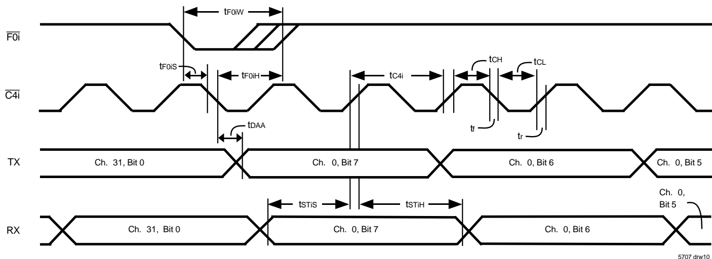
Figure 7. ST-BUS® Timing
