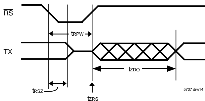
Figure 11. Reset
