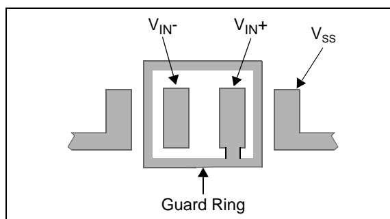
FIGURE 3-5: Example Guard Ring Layout for Inverting Gain.
