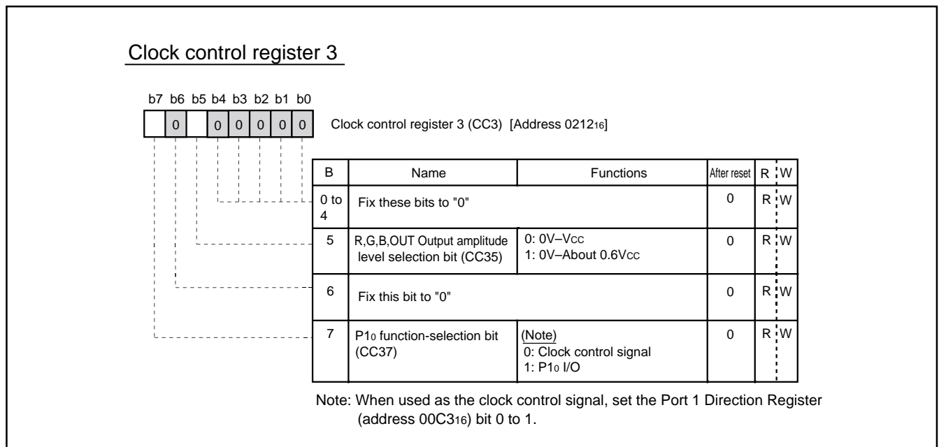
Fig.8.14.6 Clock Control Register 3
