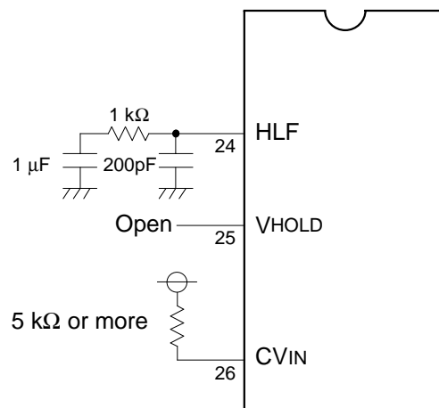
Fig. 8.10.3 Termination of Data Slicer Input/Output Pins when Timing Signal Generating Circuit Is in ON State
