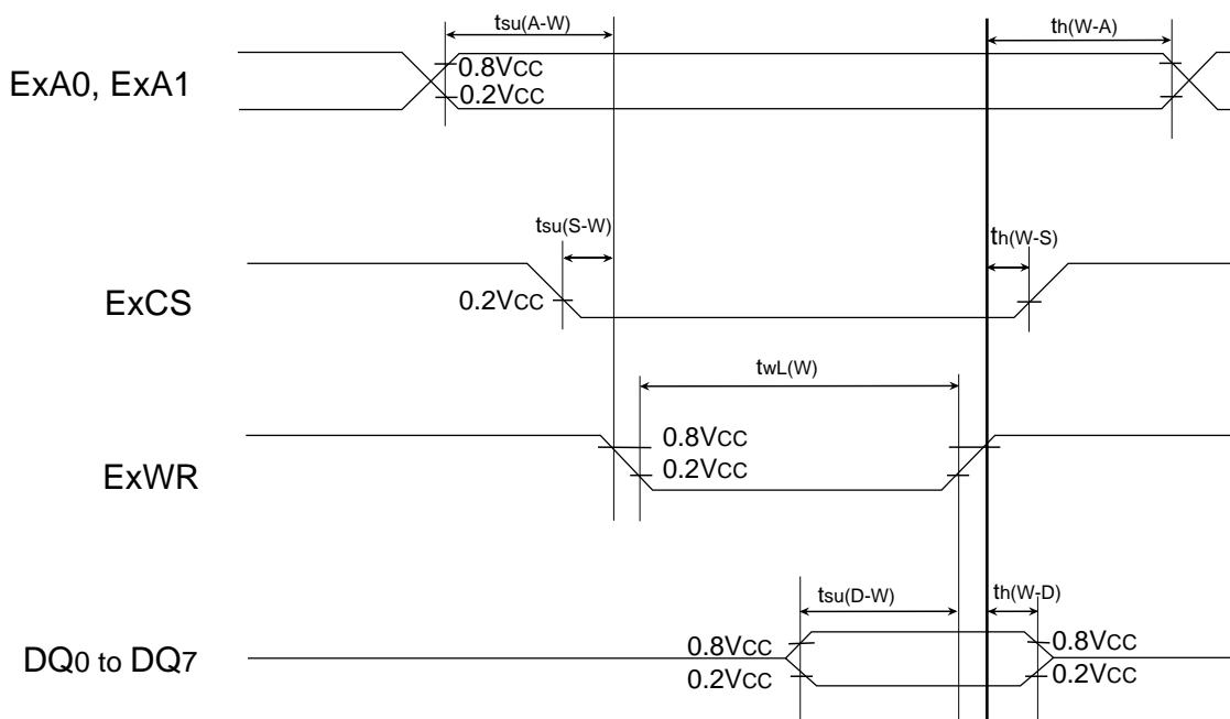
Fig. 175 Timing chart (2)
