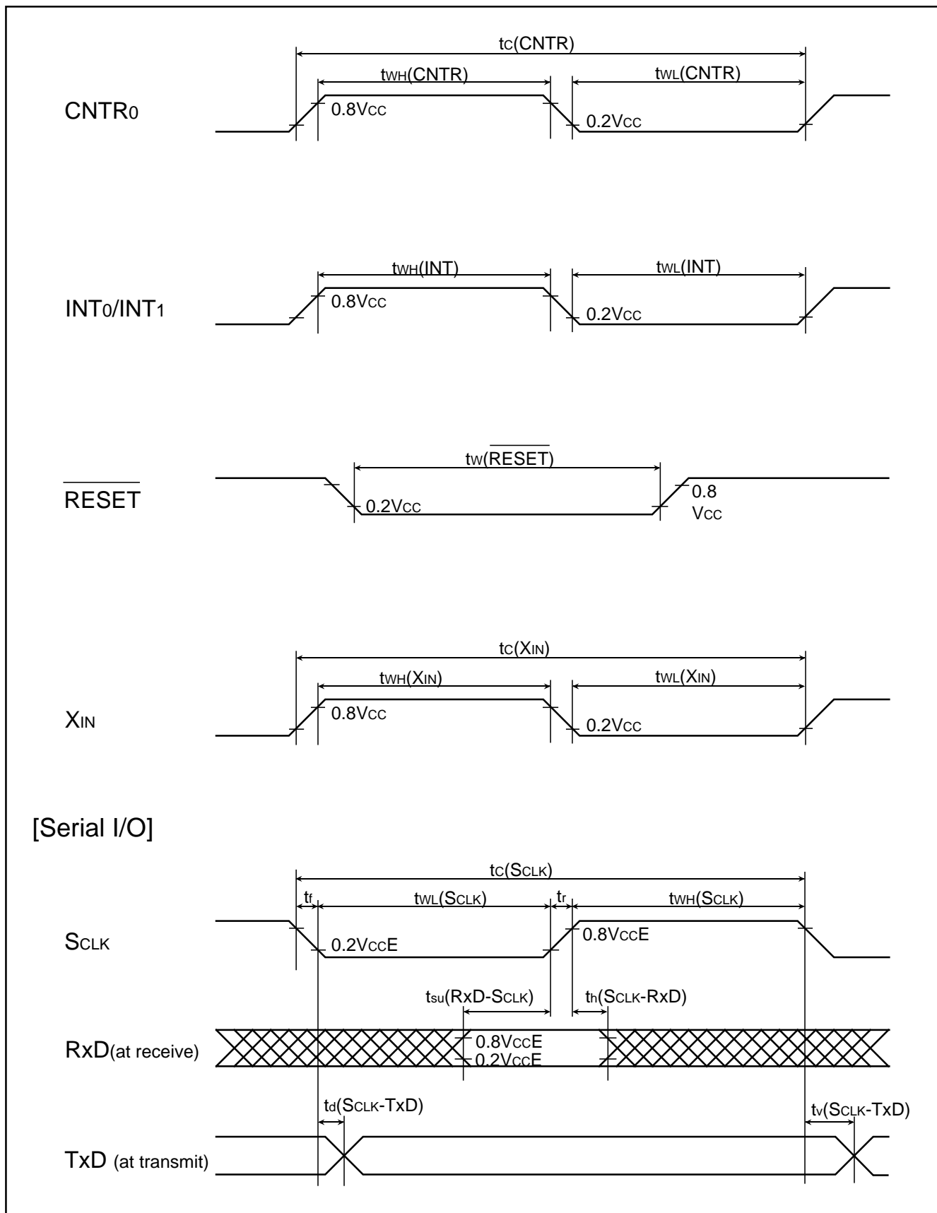
Fig. 174 Timing chart (1)
