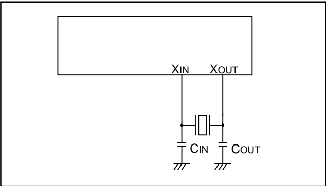
Fig. 141 Ceramic resonator or quartz-crystal oscilltor circuit
