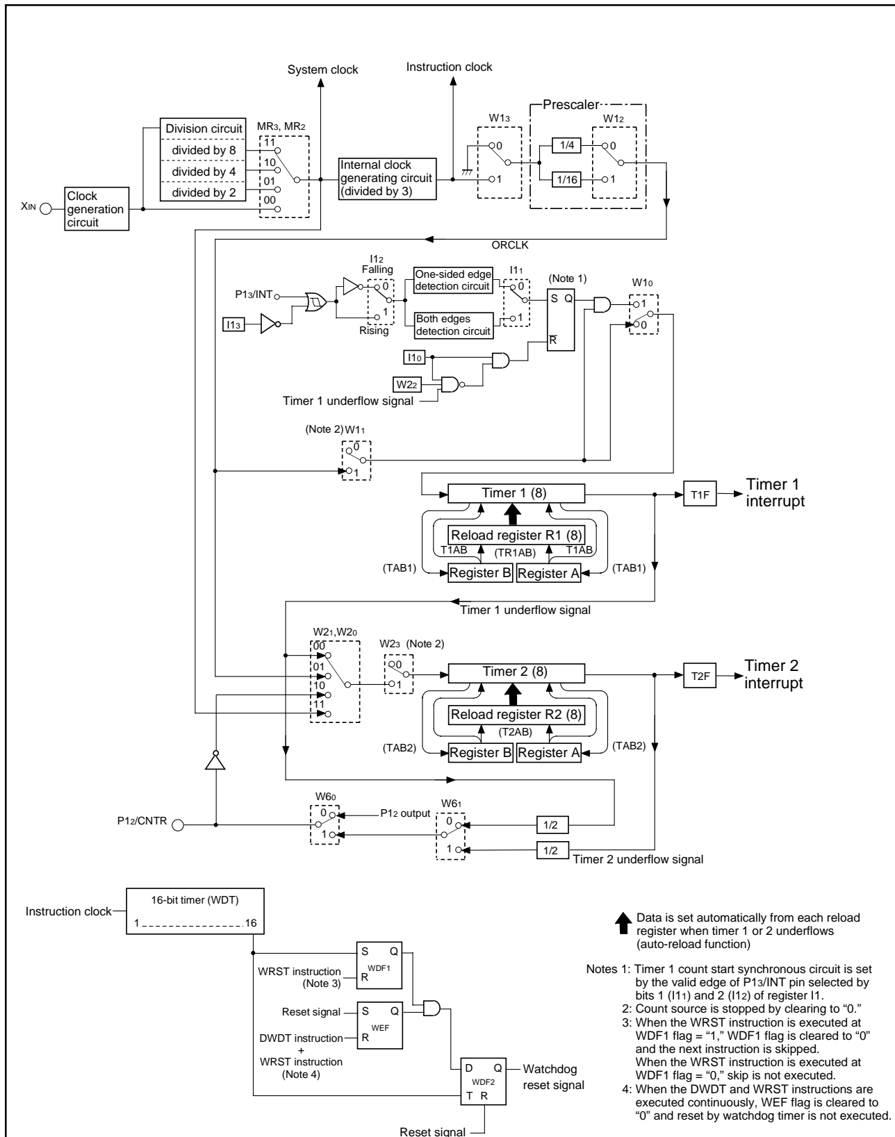
Fig. 22 Timers structure
