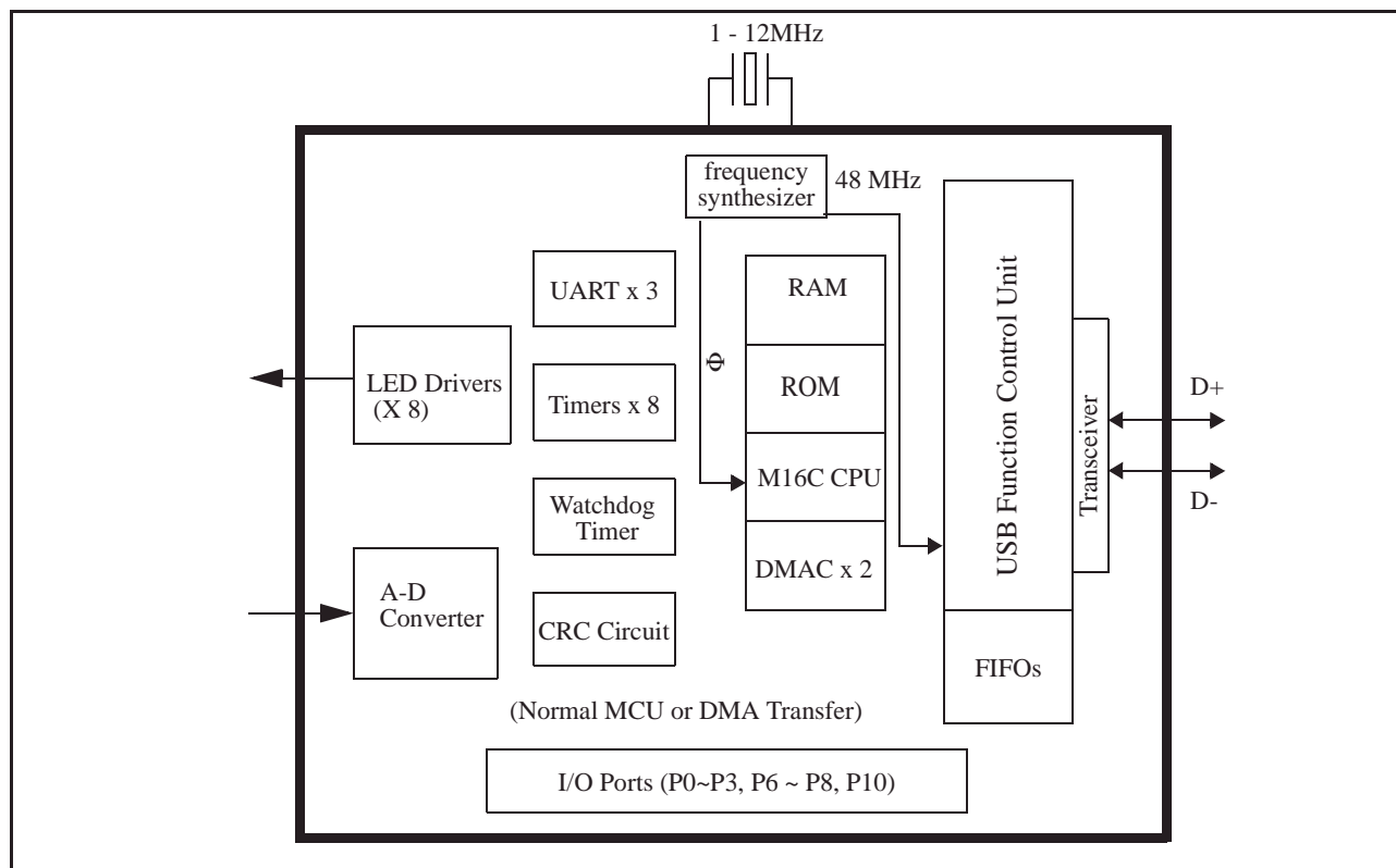
Figure 1.4: M30240 block diagram
