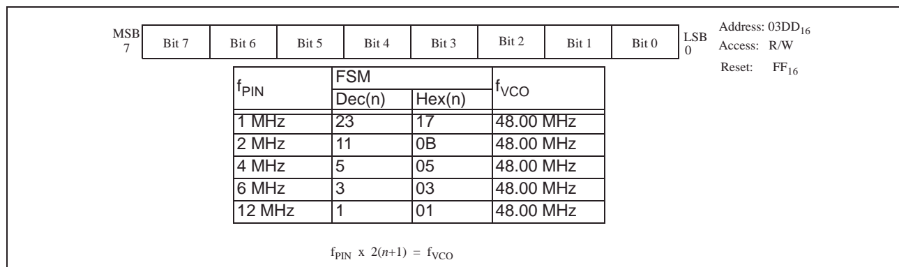
Figure 1.25: Frequency Synthesizer Multiplier Register (FSM)
