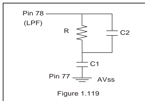
Figure 1.119: LPF Filter Schematic
