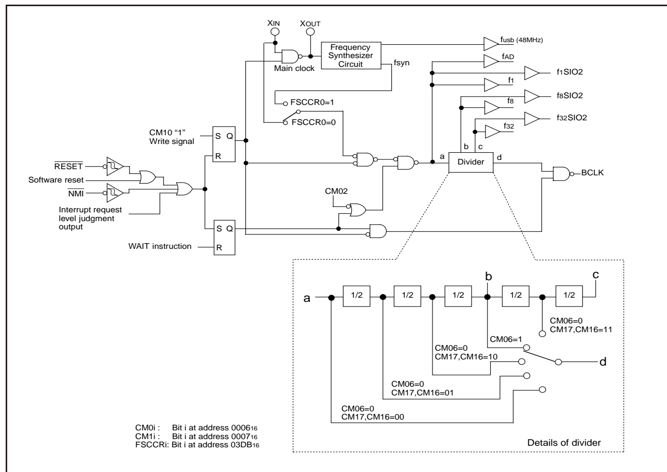
Figure 1.12: Clock-generating circuit
