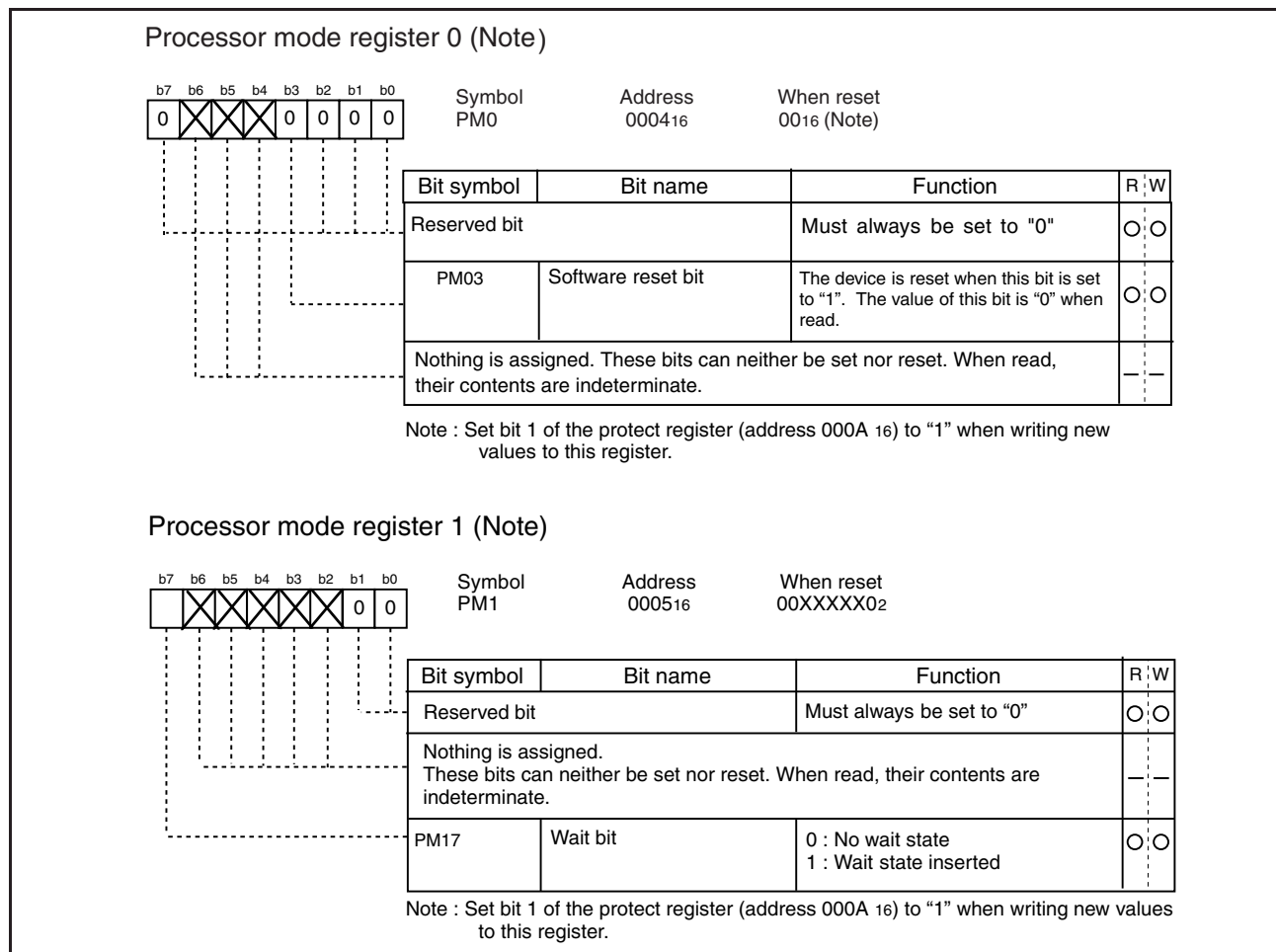
Figure 1.7: Processor mode registers 0 and 1
