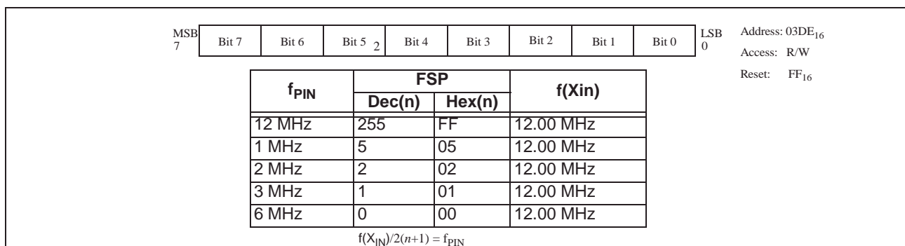
Figure 1.24: Frequency Synthesizer Prescaler Register (FSP)
