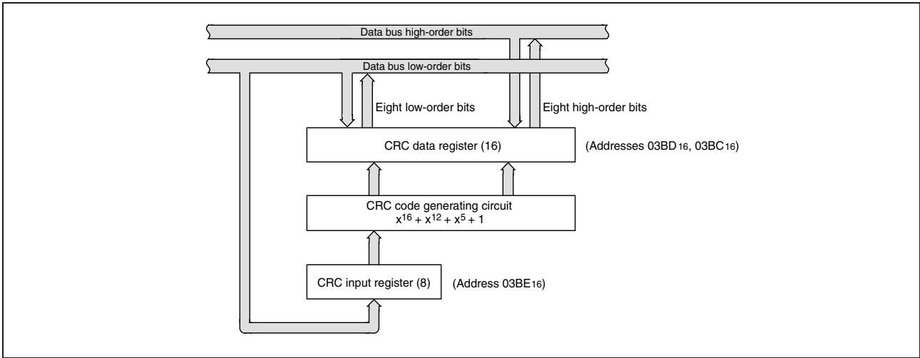
Figure 1.104: Block diagram of CRC circuit
