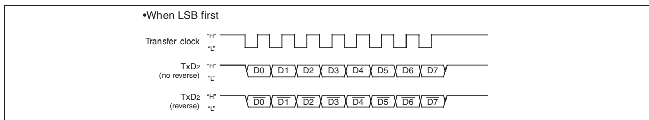
Figure 1.86: Serial data logic switch timing
