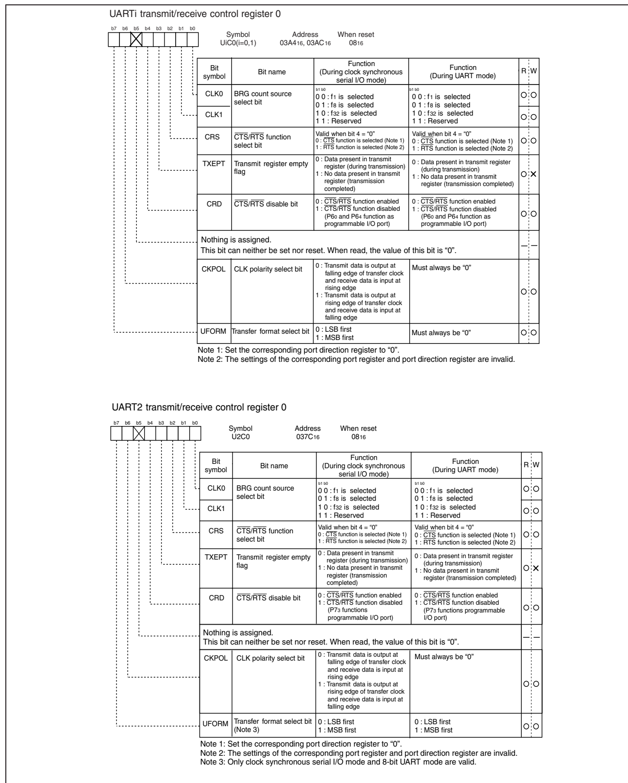
Figure 1.78: Serial I/O-related registers (3)
