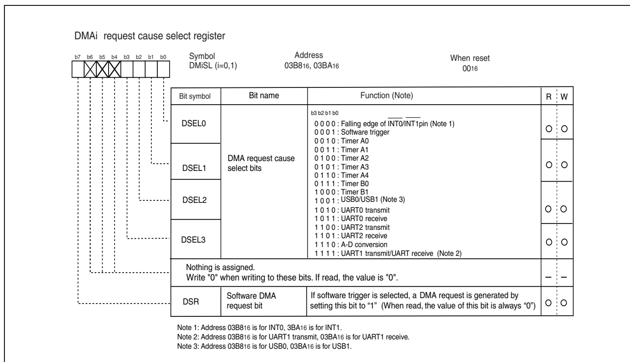
Figure 1.54: DMAC register (1)
