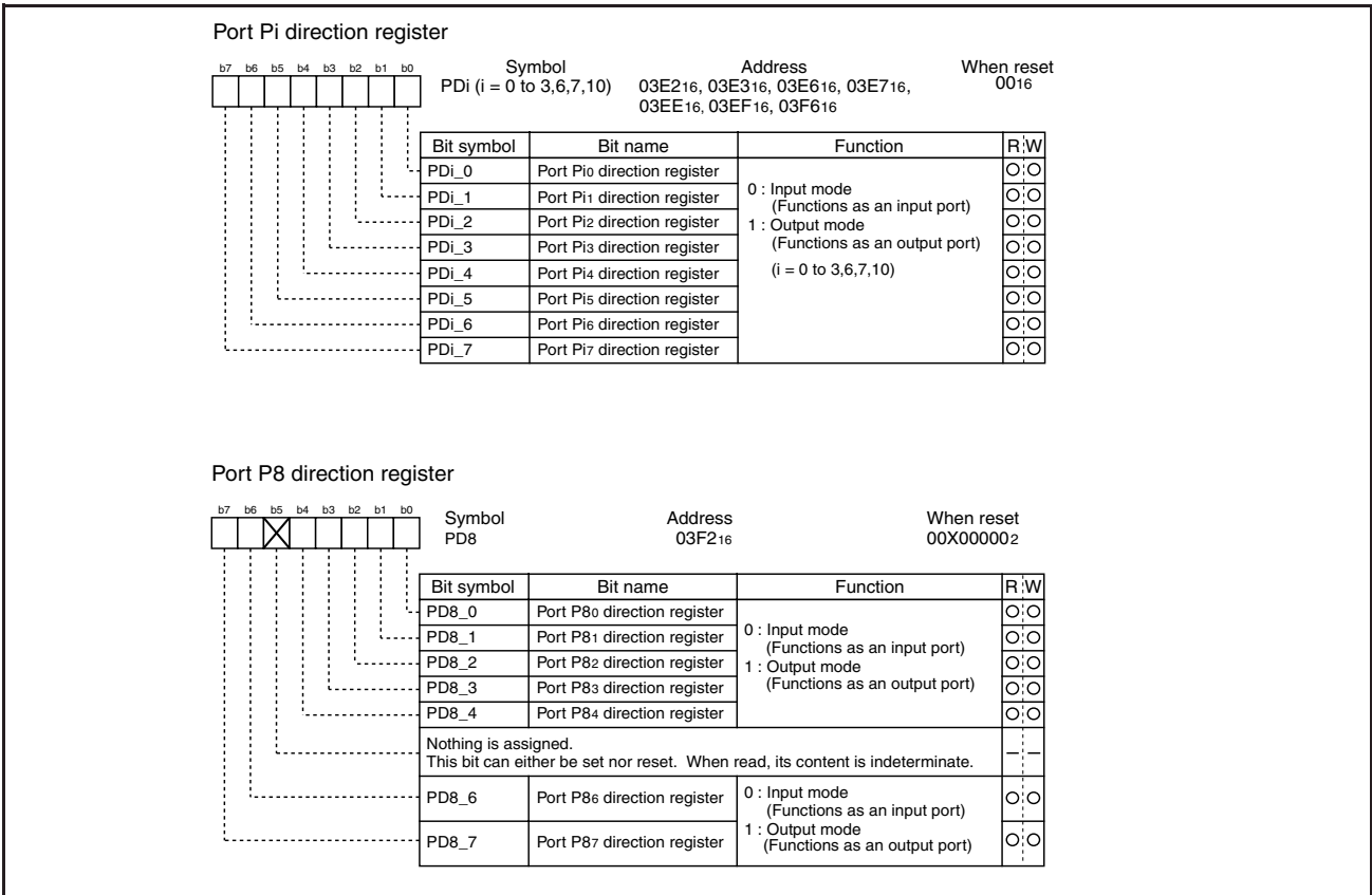
Figure 1.109: Direction register
