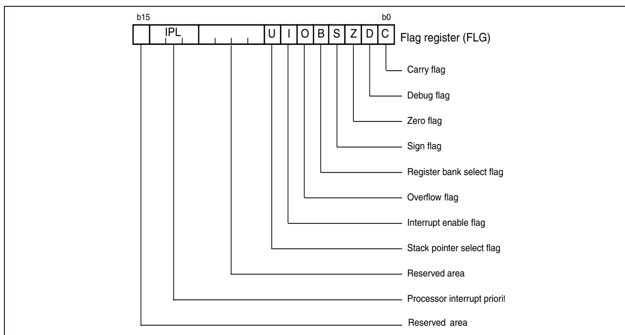
Figure 1.6: Flag register (FLG)
