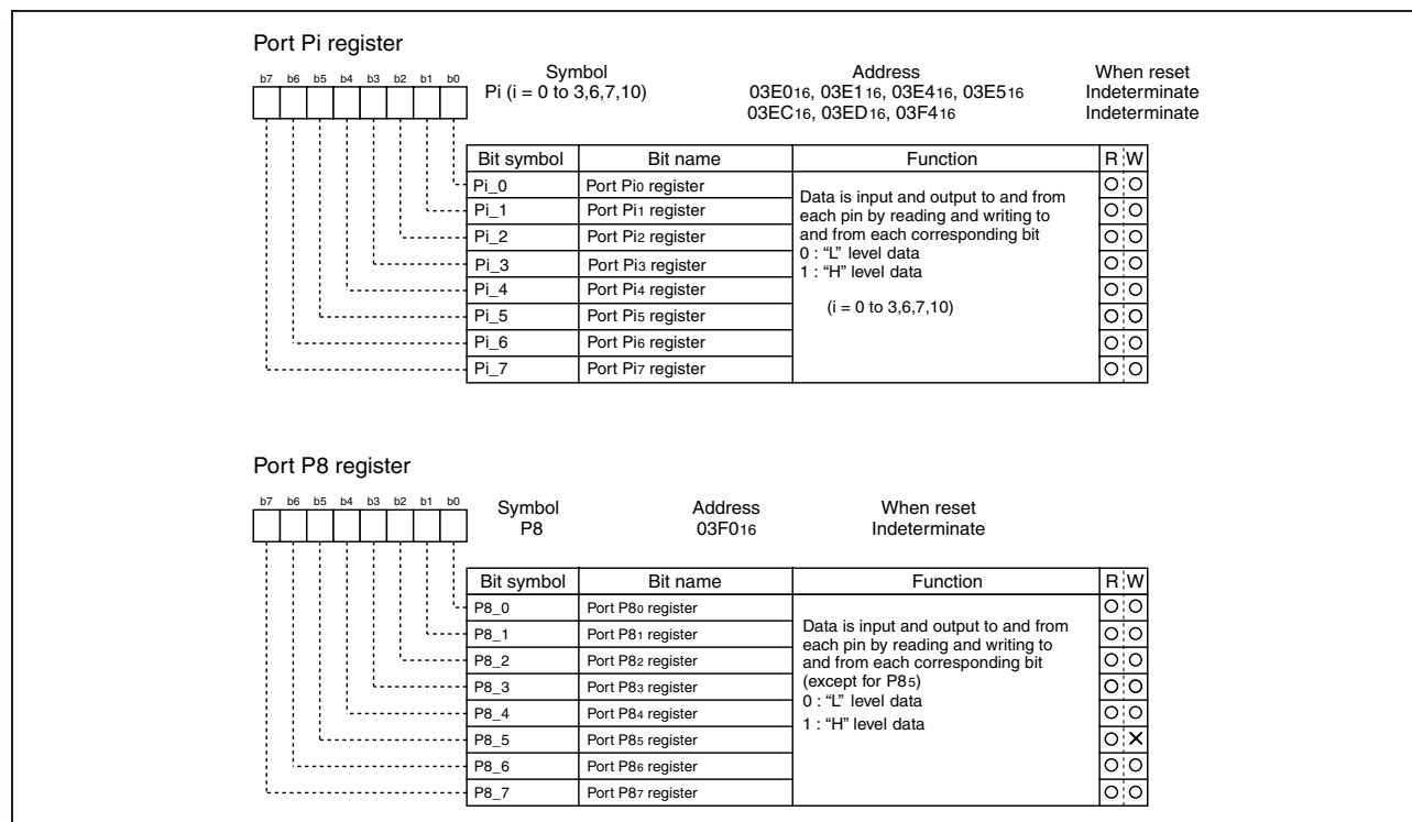
Figure 1.110: Port register
