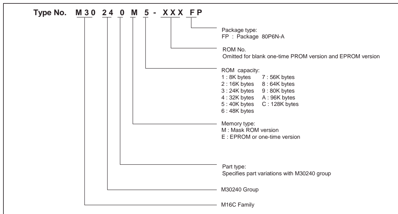
Figure 1.3: Type number, memory size, and package
