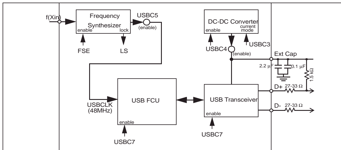
Figure 1.117: PLL, DC-DC Converter and USB Functional Block Diagram
