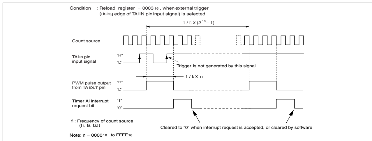
Figure 1.67: Example of how a 16-bit pulse-width modulator operates
