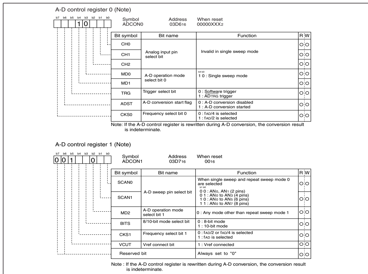
Figure 1.101: A-D conversion register in single-sweep mode
