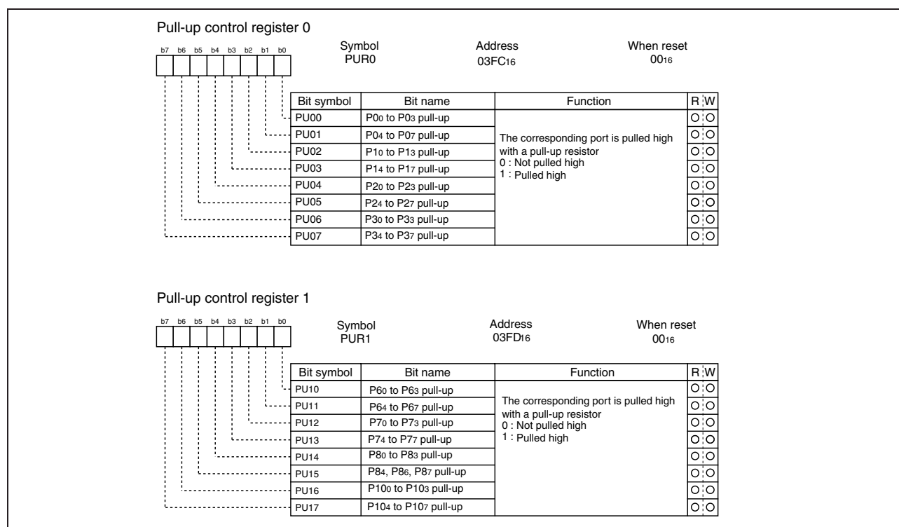
Figure 1.111: Pull-up control register
