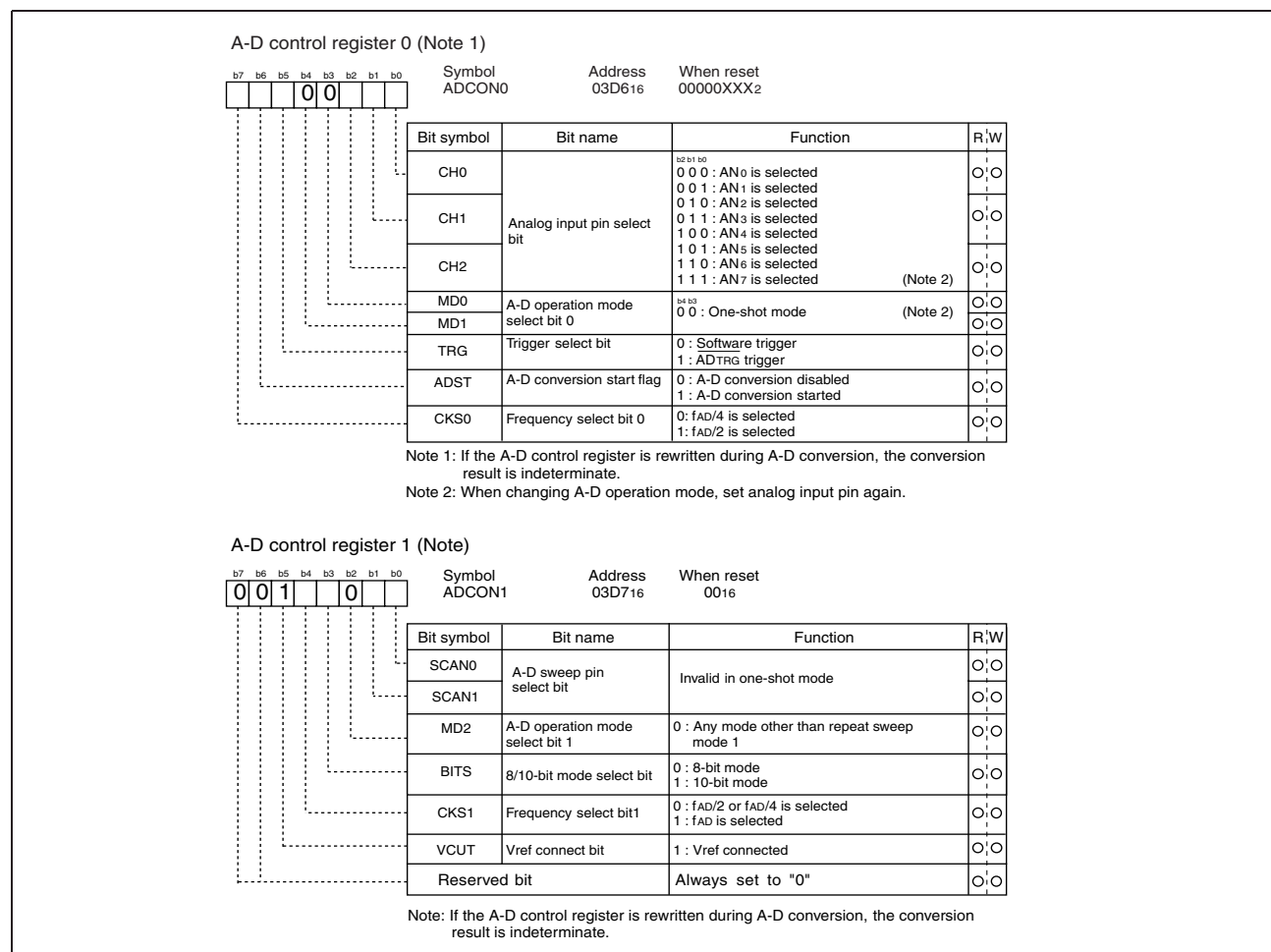
Figure 1.99: A-D conversion register in one-shot mode
