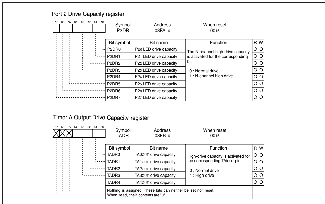
Figure 1.112: Port 2 and Timer A Output drive capacity registers
