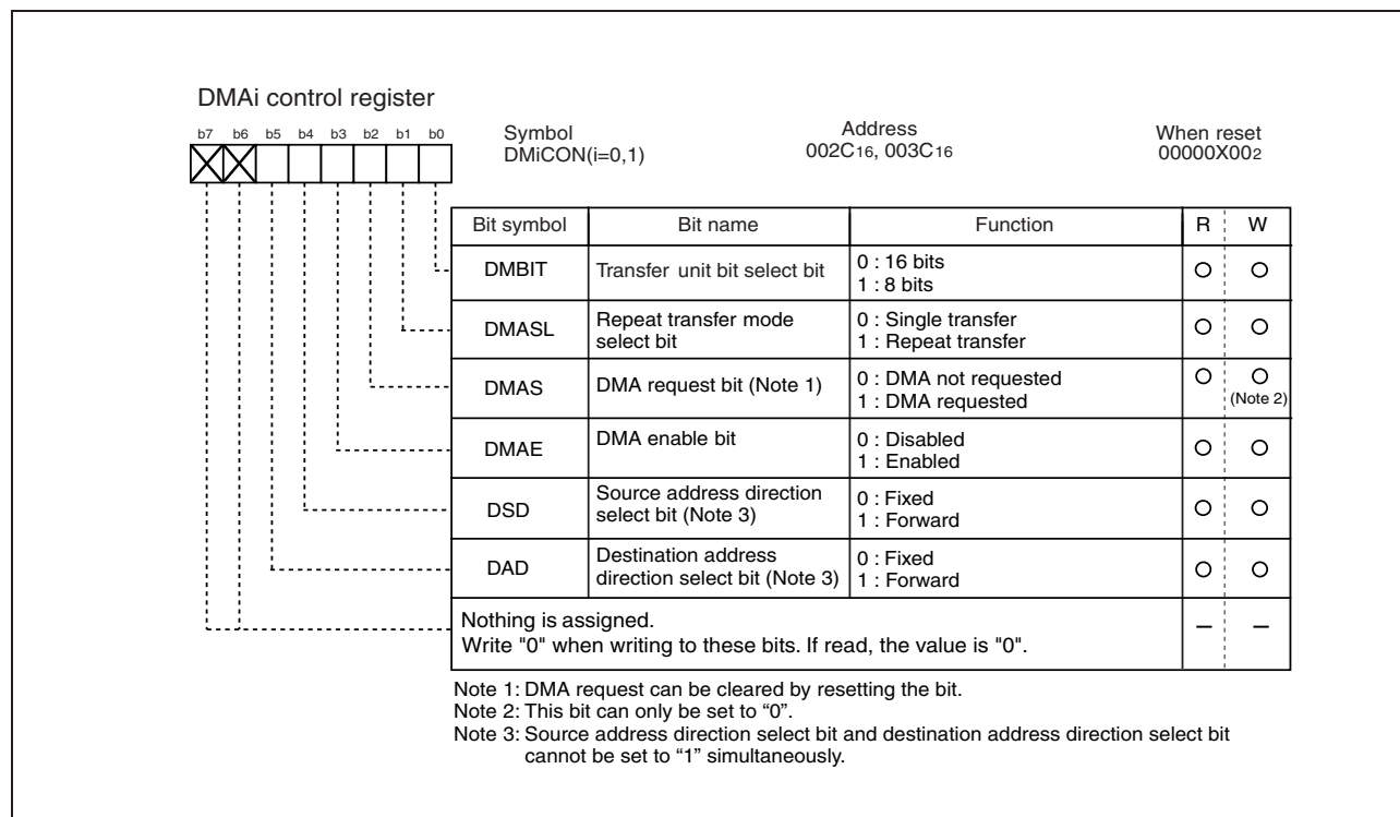
Figure 1.55: DMAC register (2)
