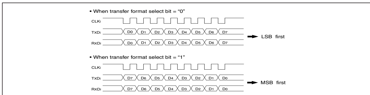
Figure 1.84: Transfer format
