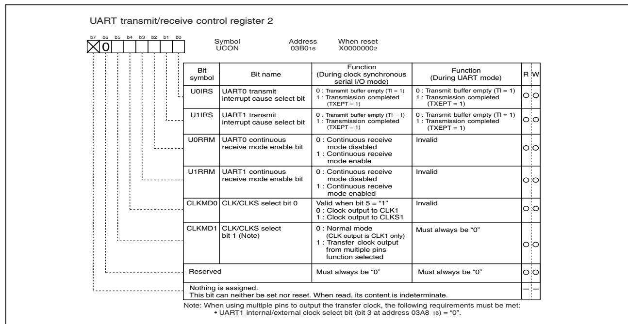
Figure 1.80: Serial I/O-related registers (5)
