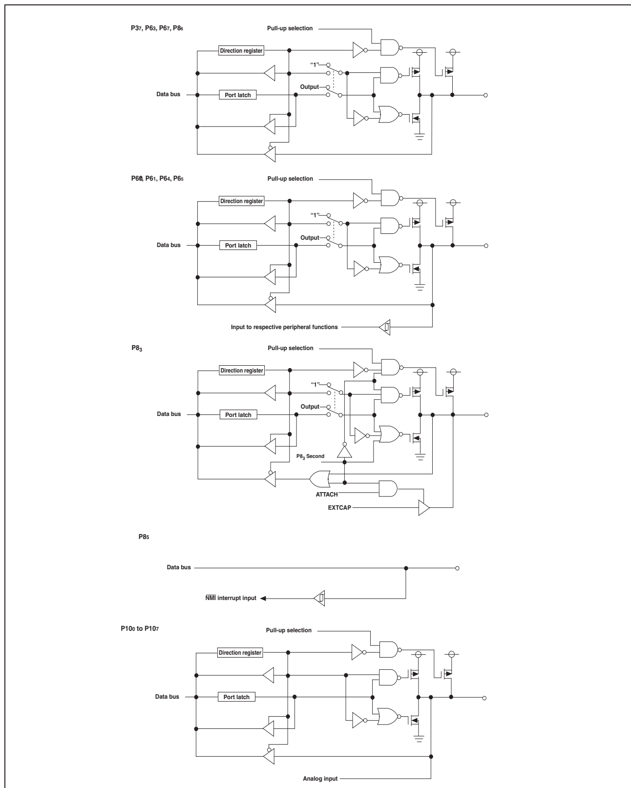
Figure 1.107: Programmable I/O ports (2)
