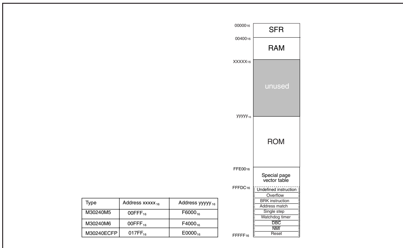
Figure 1.8: Memory Map
