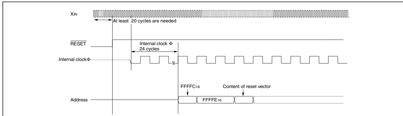
Figure 1.10: Reset sequence
