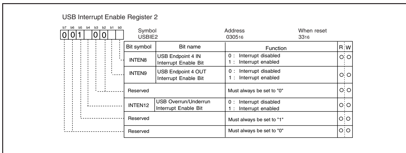
Figure 1.37: USB Interrupt Enable Register 2
