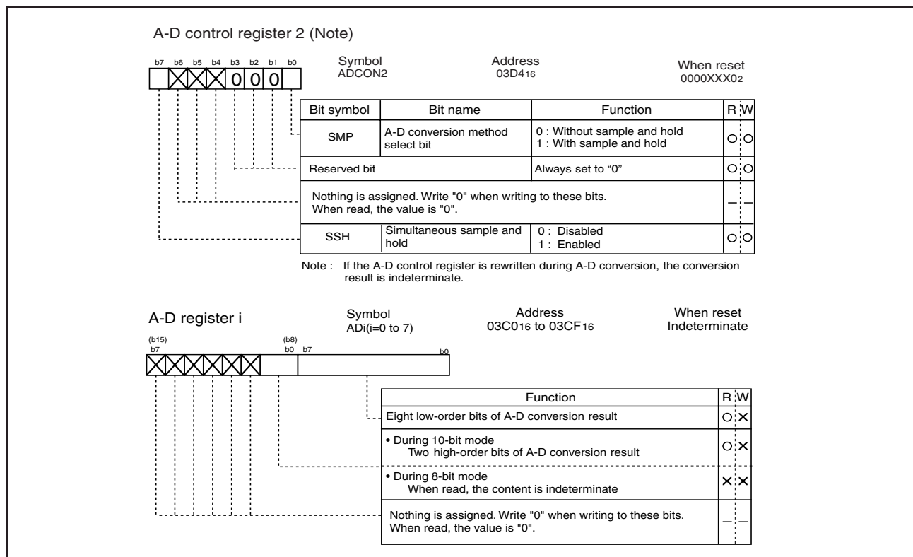
Figure 1.98: A-D converter-related registers (2)
