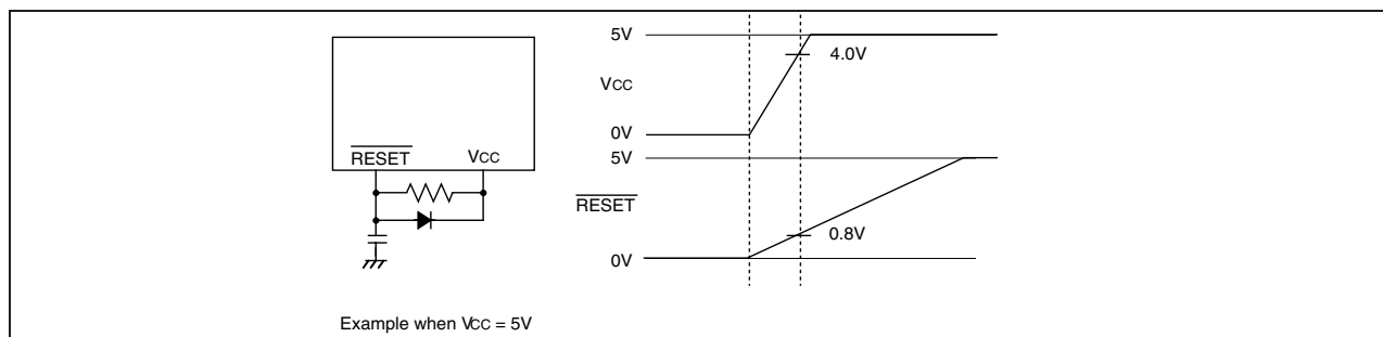
Figure 1.9: Reset circuit
