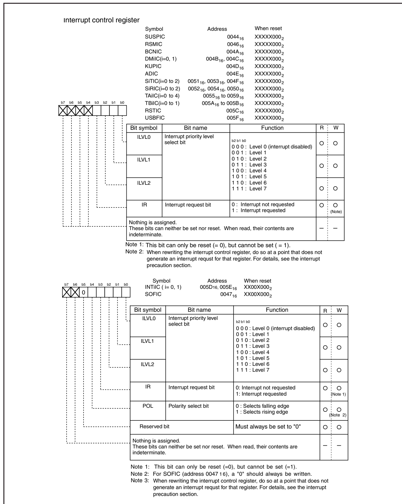
Figure 1.16: Interrupt control registers
