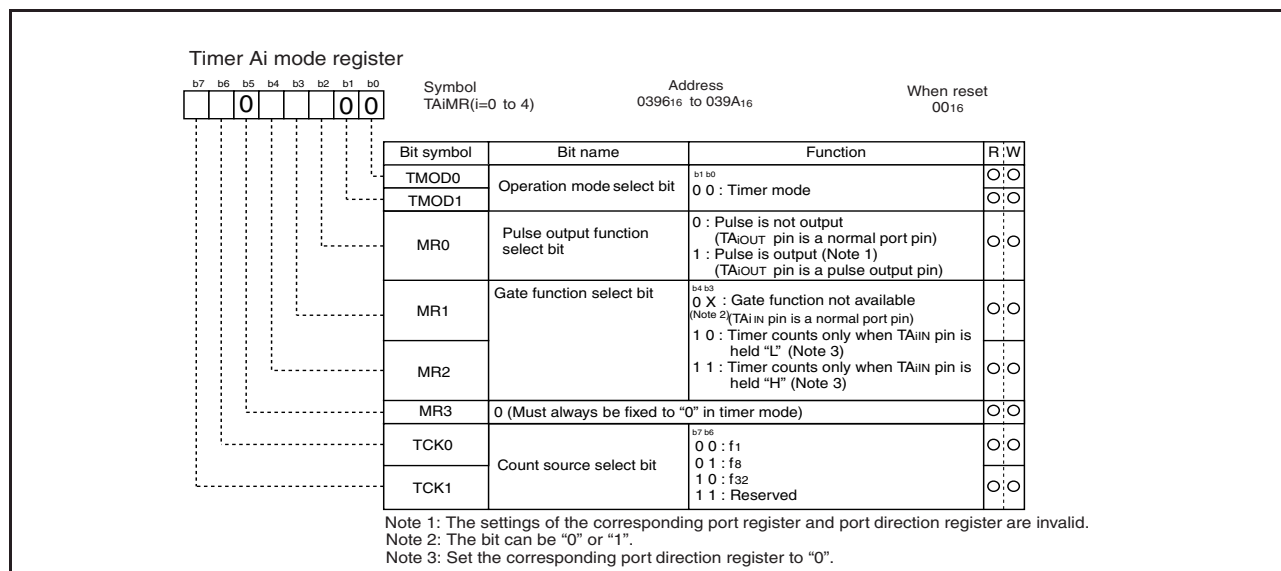
Figure 1.63: Timer Ai mode register in timer mode
