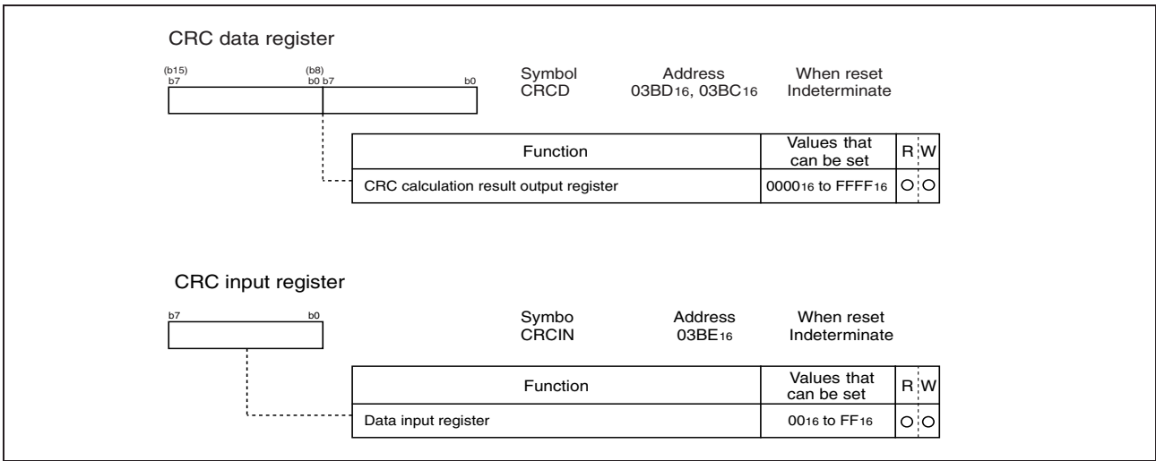
Figure 1.105: CRC-related registers
