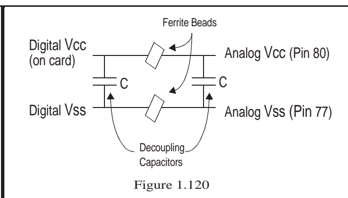
Figure 1.120: Power Supply
