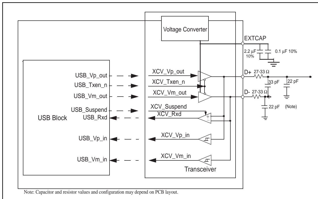
Figure 1.121: Configuration of External USB components
