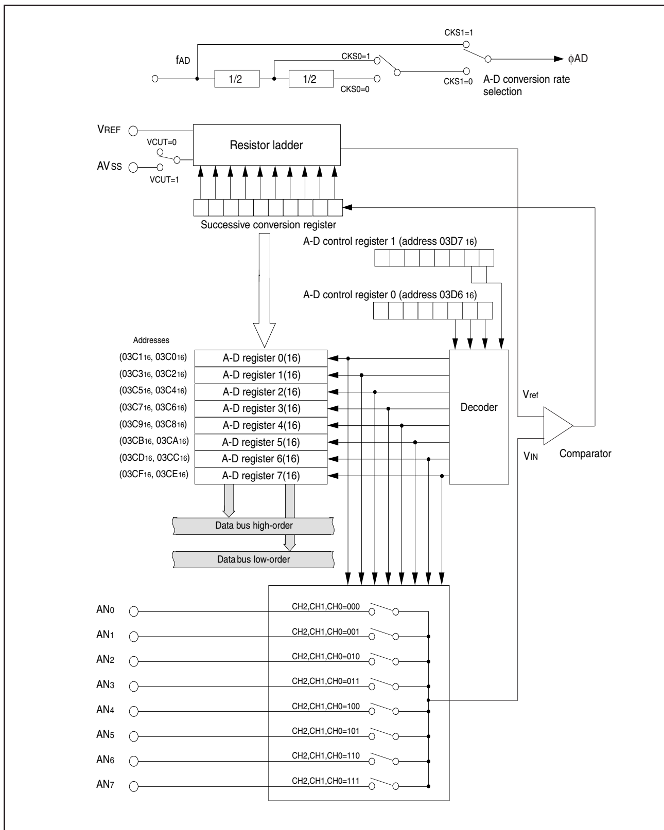
Figure 1.96: Block diagram of A-D converter
