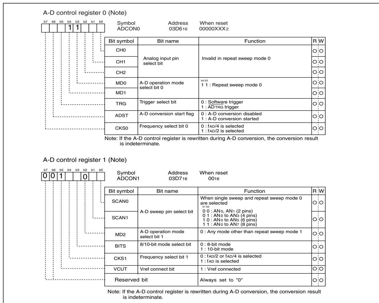
Figure 1.102: A-D conversion register in repeat-sweep mode 0
