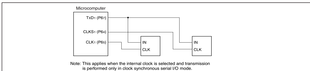
Figure 1.85: The transfer clock output from the multiple pins function usage
