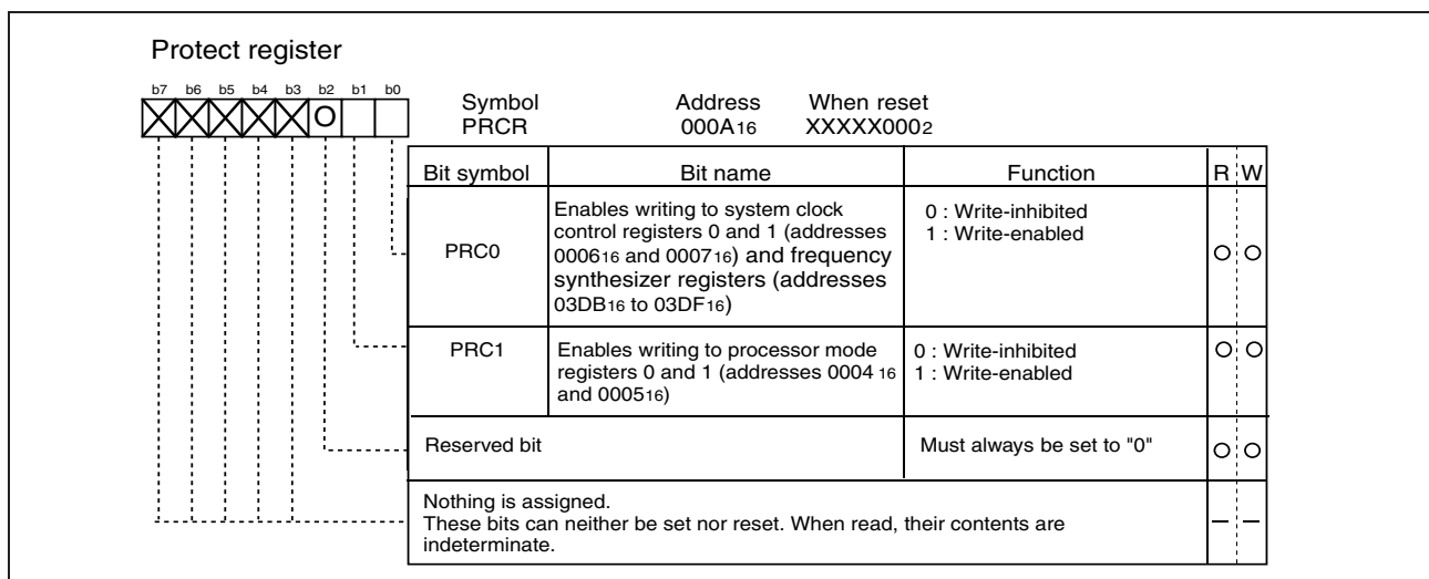
Figure 1.14: Protect register
