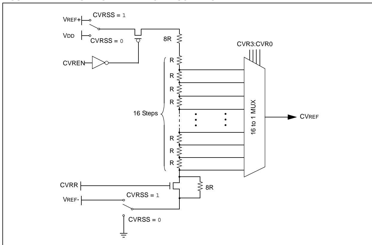
FIGURE 21-1: VOLTAGE REFERENCE BLOCK DIAGRAM
