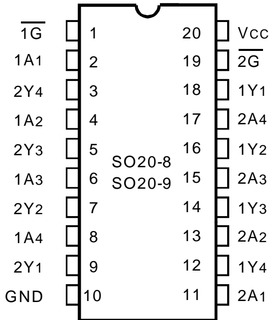
QSOP/TSSOP TOP VIEW
