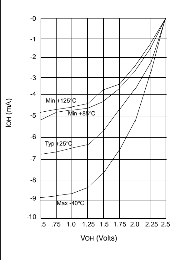
FIGURE 12-7: IOH vs. VOH, VDD = 2.5 V
