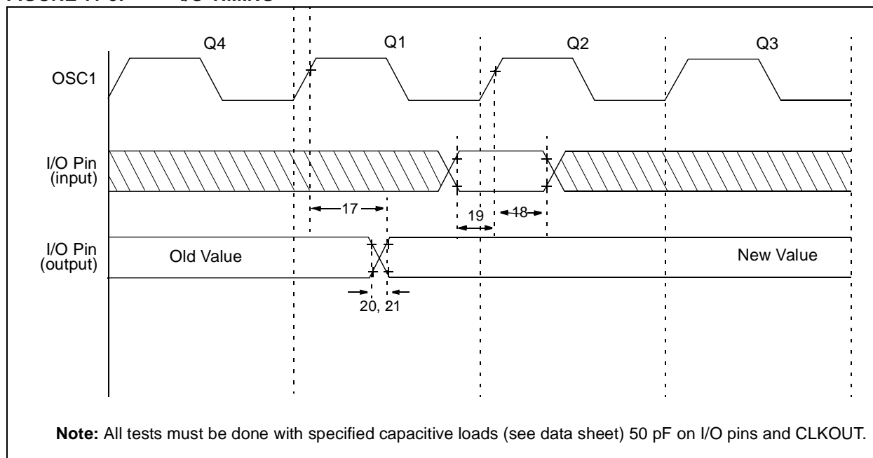
FIGURE 11-5: I/O TIMING
