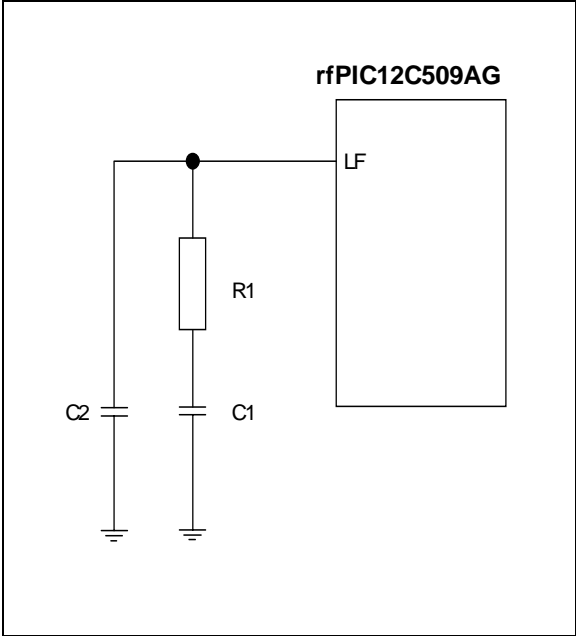
FIGURE 7-5: EXAMPLE LOOP FILTER CIRCUIT
