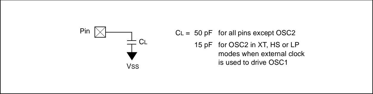
FIGURE 11-3: LOAD CONDITIONS
