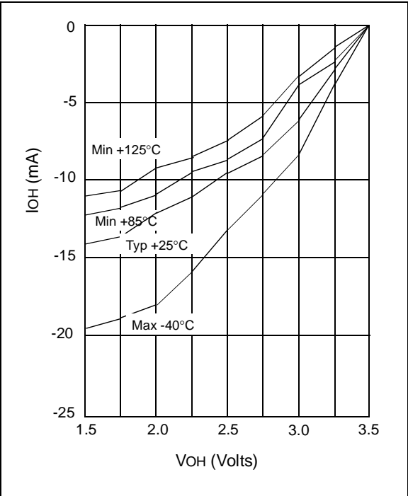
FIGURE 12-8: IOH vs. VOH, VDD = 3.5 V
