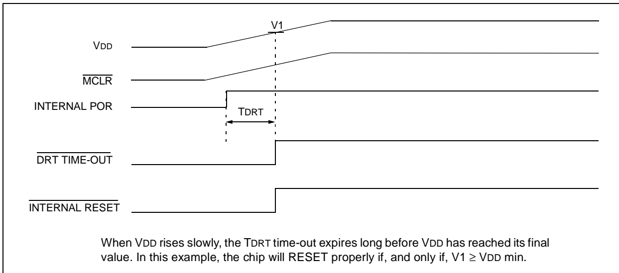
FIGURE 8-9: TIME-OUT SEQUENCE ON POWER-UP ( \overline{\text{MCLR}} TIED TO \text{V}_{\text{DD}} ): SLOW \text{V}_{\text{DD}} RISE TIME
