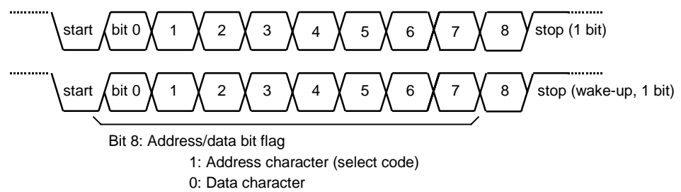
Figure 13.1 Data Formats
