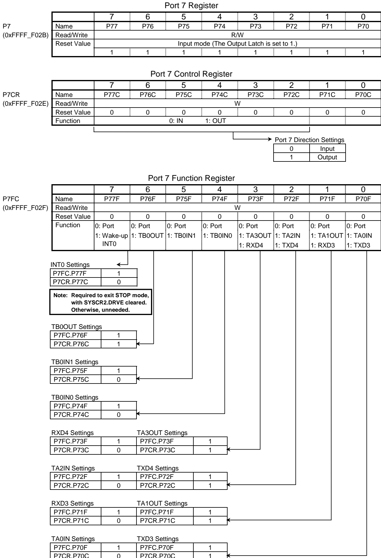
Figure 7.17 Port 7 Registers
