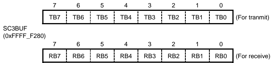
Figure 13.25 SIO3 Transmit/Receive Buffer Register (SC3BUF)
