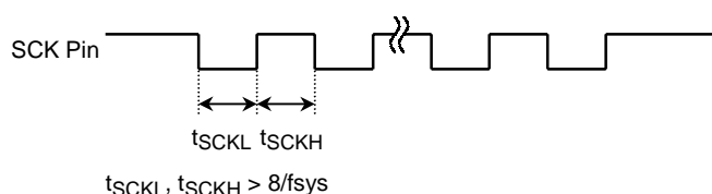
Figure 14.22 Maximum External Clock Frequency
