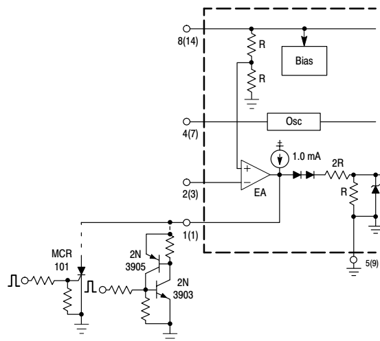
Figure 31. Latched Shutdown
