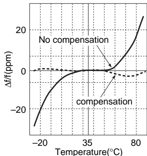
TCXO, Frequency compensation of crystal
