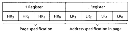
Figure 2-4. Configuration of H and L Registers
