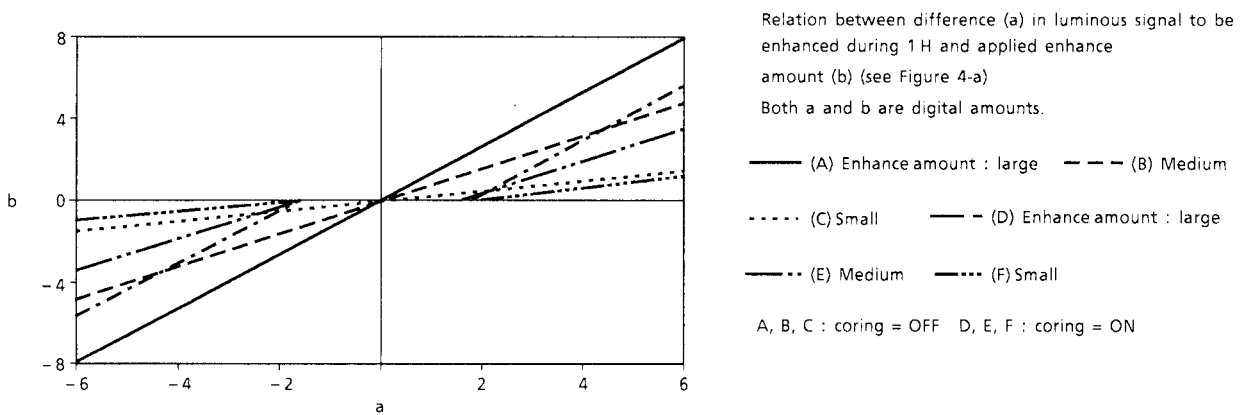
(Figure 4-c) VERTICAL ENHANCE CHARACTERISTICS(ENLARGED)
