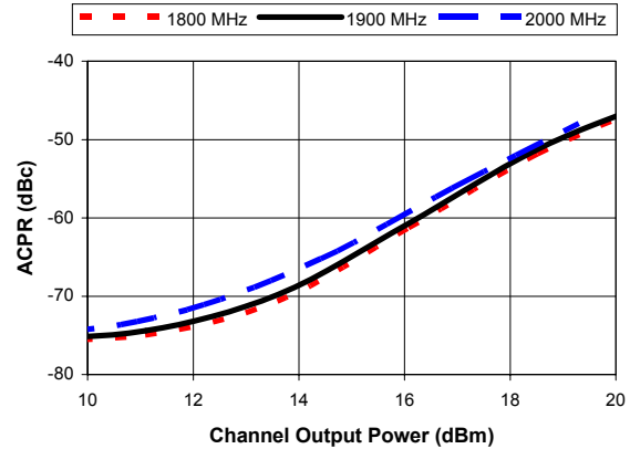
ACPR - PCS Band (9 channels Forward)
