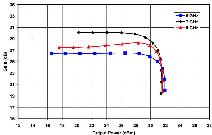
Figure 8. Gain vs. Output Power and Frequency at VD = 6V and IDQ = 640mA
