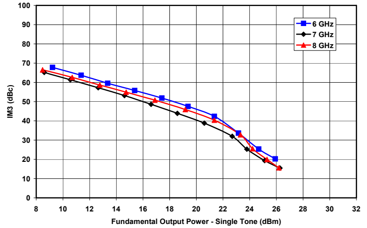
Figure 20. Third Order Intermod vs. Output Power and Frequency at VD = 6V and IDQ = 640mA
