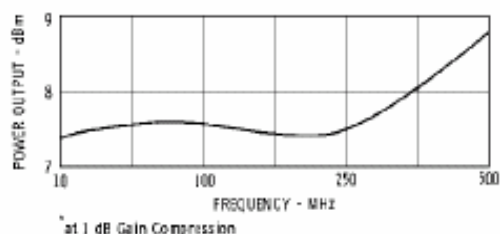
Power Output*
