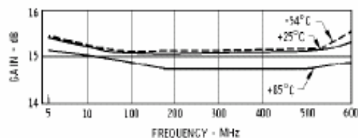
Gain
