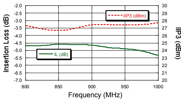
Low Gain Mode: Insertion Loss and Input IP3
