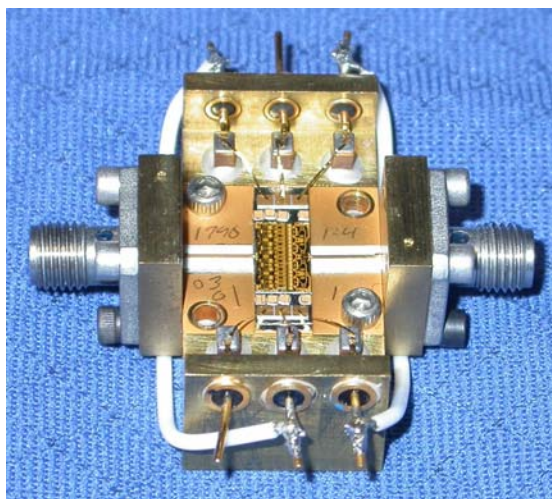
Figure 16. Fixture used to characterize MAAPGM0076-DIE under CW stimulus.
