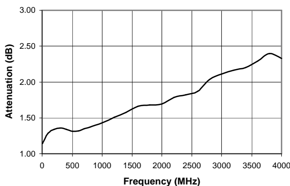
Insertion Loss
