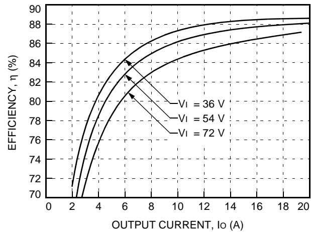
Figure 3. Typical FW300C1 Efficiency vs. Output Current at Room Temperature
