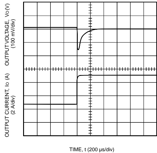
Figure 12. Typical JC100A Transient Response to Step Increase in Load from 50% to 75% of Full Load at Room Temperature and 28 V Input (Waveform Averaged to Eliminate Ripple Component.)
