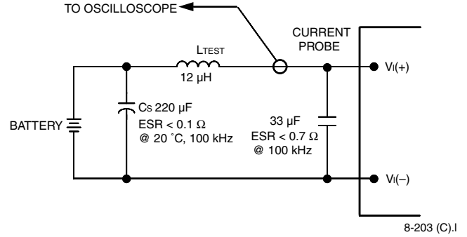
Note: Measure input reflected-ripple current with a simulated source inductance ( L_{TEST} ) of 12 \mu H. Capacitor C_s offsets possible battery impedance. Measure current as shown above.
