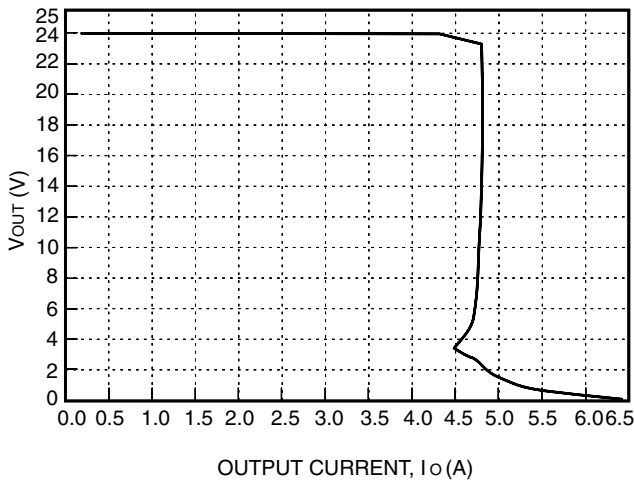
Figure 6. Typical JC100H Output Characteristics at Room Temperature, V_{IN} = 28\text{ V}
