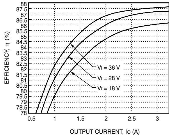
Figure 7. Typical JC050H Converter Efficiency vs. Output Current at Room Temperature
