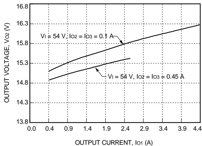
Figure 8. DW025ACL-M Typical Cross Regulation with Respect to I_{o1}
