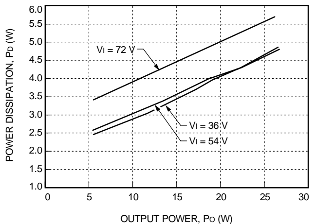
Figure 24. DW025ACL-M Fixed Losses, P_p
