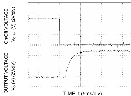
Figure 5. Typical Start-up Using Remote On/Off, negative logic version shown ( V_{IN} = V_{IN,NOM} , I_o = I_{o,max} ).
