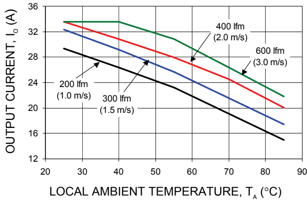
Figure 16. Output Current Derating for the QBK033A0B (Vo = 12V) in the Transverse Orientation with baseplate and 0.25-inch high heatsink; Airflow Direction from Vin(+) to Vin(-); Vin = 48V.
