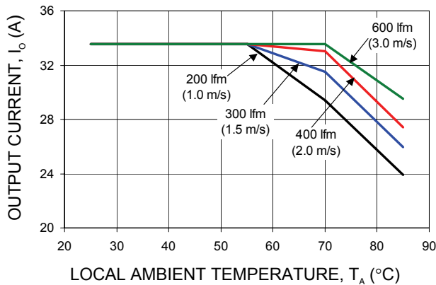
Figure 18. Output Current Derating for the QBK033A0B (Vo = 12V) in the Transverse Orientation with baseplate and 1.0-inch high heatsink; Airflow Direction from Vin(+) to Vin(-); Vin = 48V.
