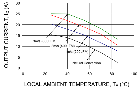
Figure 14. Output Current Derating for the QBK025A0B in the Transverse Orientation with no baseplate; Airflow Direction from V_{in}(+) to V_{in}(-) ; V_{in} = 48\text{ V} .
