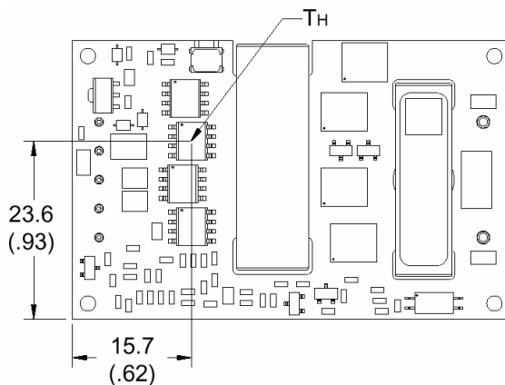
Figure 13. Location of the thermal reference temperature T_H .
