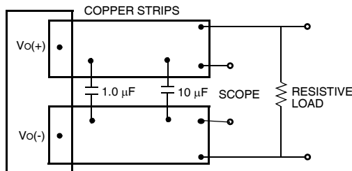
Figure 49. Input Reflected-Ripple Test Setup.
