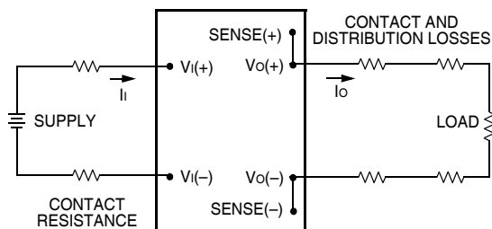
Figure 50. Peak-to-Peak Output Noise Measurement Test Setup.
