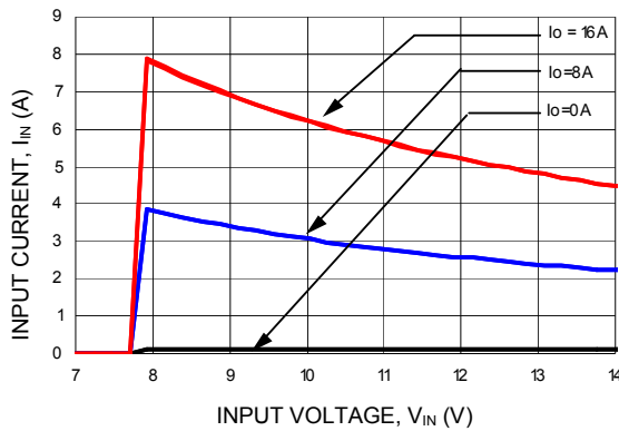
Figure 7. Input Voltage vs. Input Current ( V_O = 3.3 Vdc).
