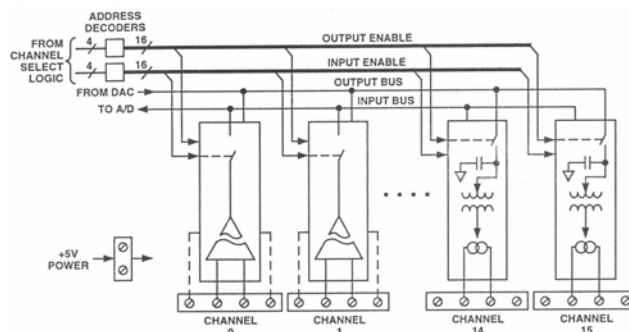
Figure 1 5B02 Functional Block Diagram
