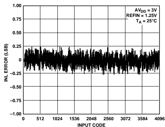
Figure 12. Typical AD5381-3 INL Plot
