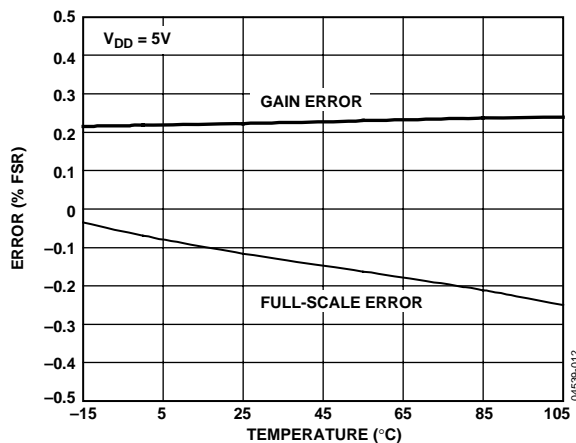
Figure 18. Gain Error and Full-Scale Error vs. Temperature
