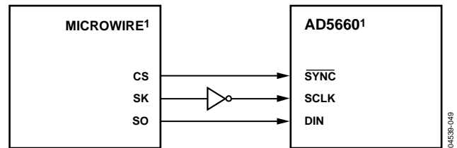
Figure 48. AD5660-to-MICROWIRE Interface
