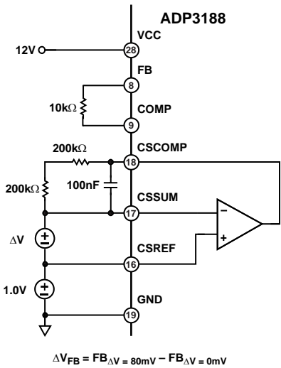
Figure 4. Positioning Voltage
