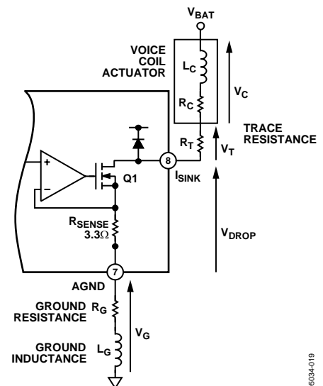
Figure 19. Effect of PCB Trace Resistance and Inductance
