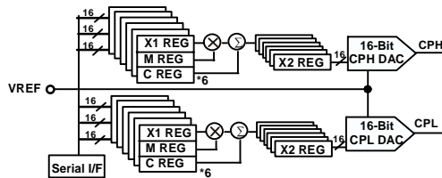
Figure 13. Comparator Registers
