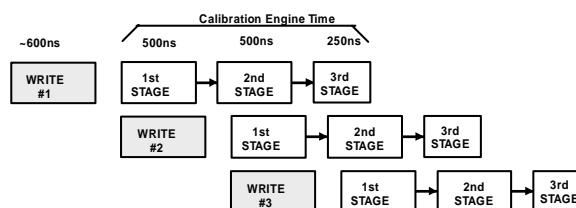
Figure 18. Multiple Single Channel writes engaging calibration engine
