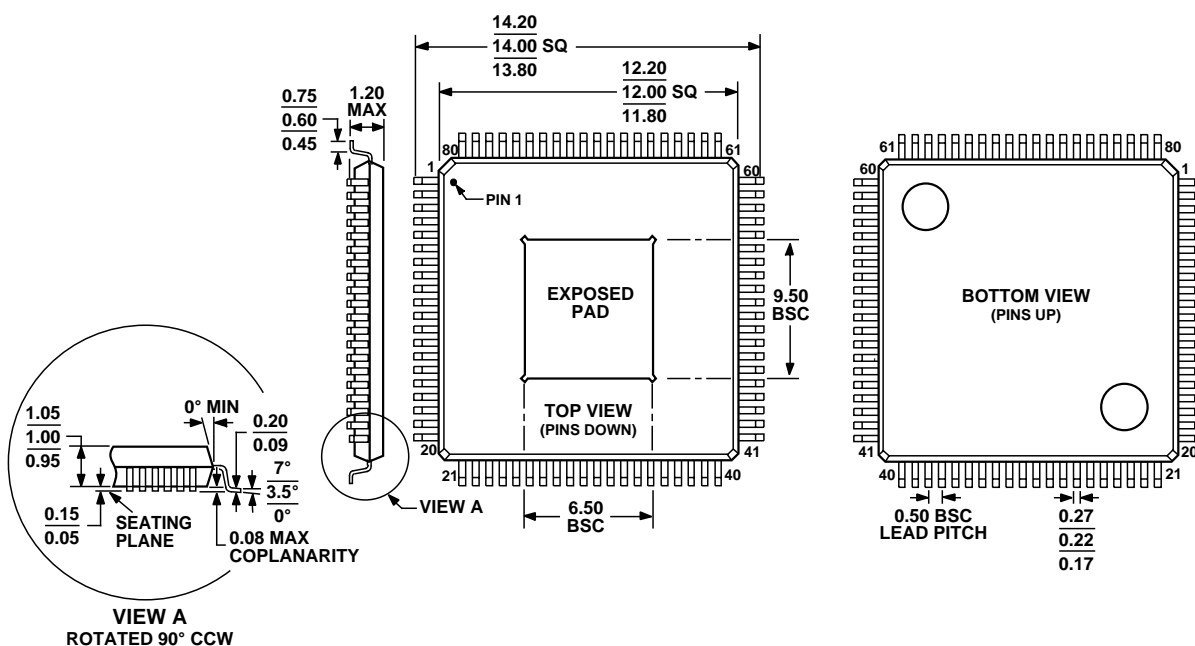
Figure 21. 80 lead TQFP/EP with exposed pad on bottom
