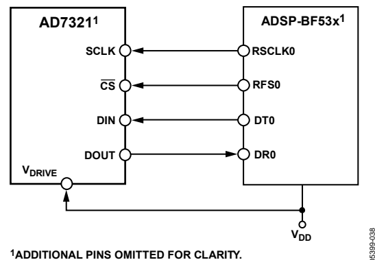
Figure 52. Interfacing the AD7321 to the ADSP-BF53x
