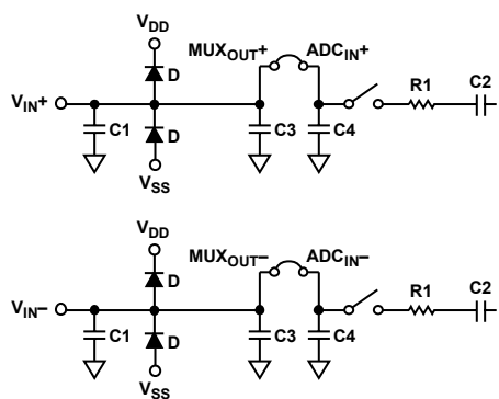
Figure 31. Equivalent Analog Input Circuit (Differential)
