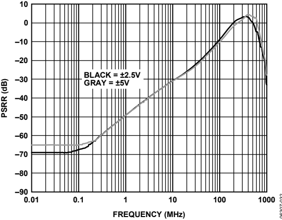
Figure 32. Negative Power Supply Rejection Ratio vs. Frequency
