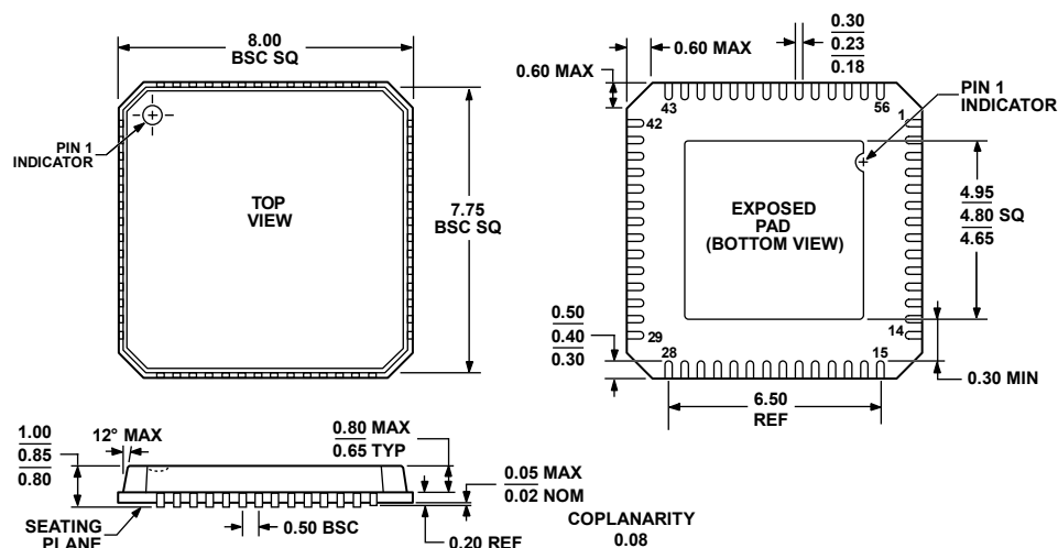
COMPLIANT TO JEDEC STANDARDS MO-220-VLLD-2 Figure 36. 56-Lead Lead Frame Chip Scale Package [LFCSP_VQ] 8 mm x 8 mm Body, Very Thin Quad (CP-56-3) Dimensions shown in millimeters
